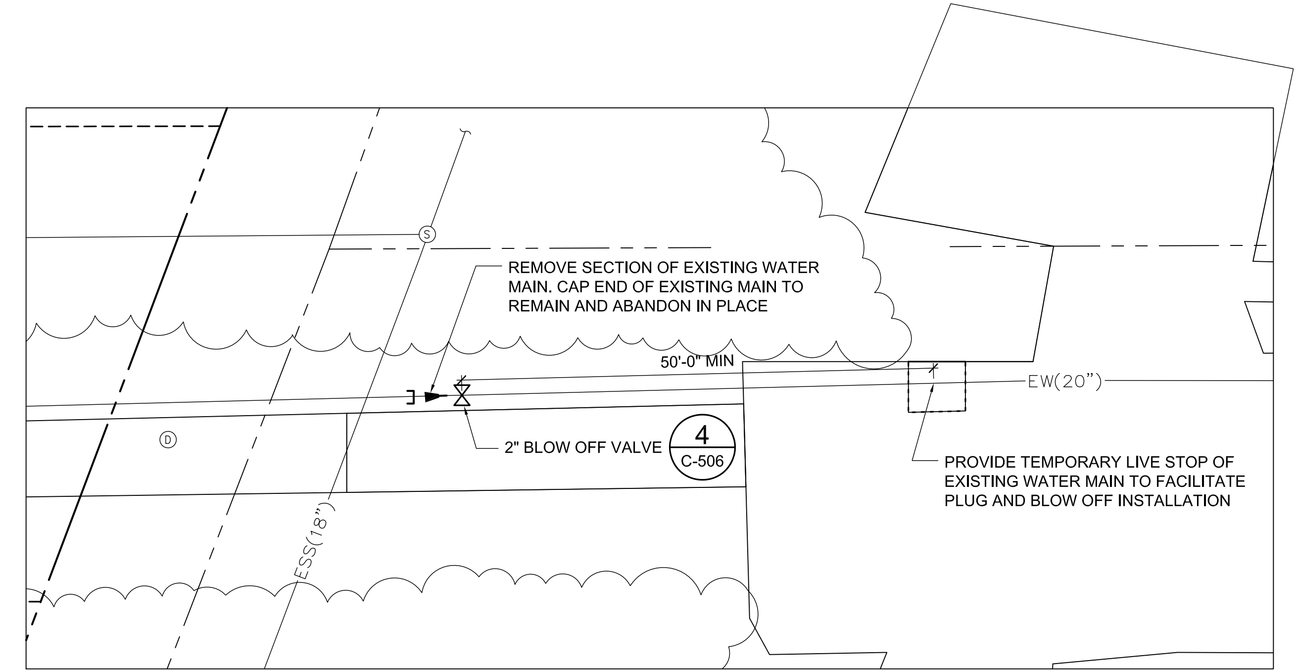
2 20" MAIN AT PINECREST STREET - UTILITY PLAN CU101/ CU104 SCALE: 1"=10'
