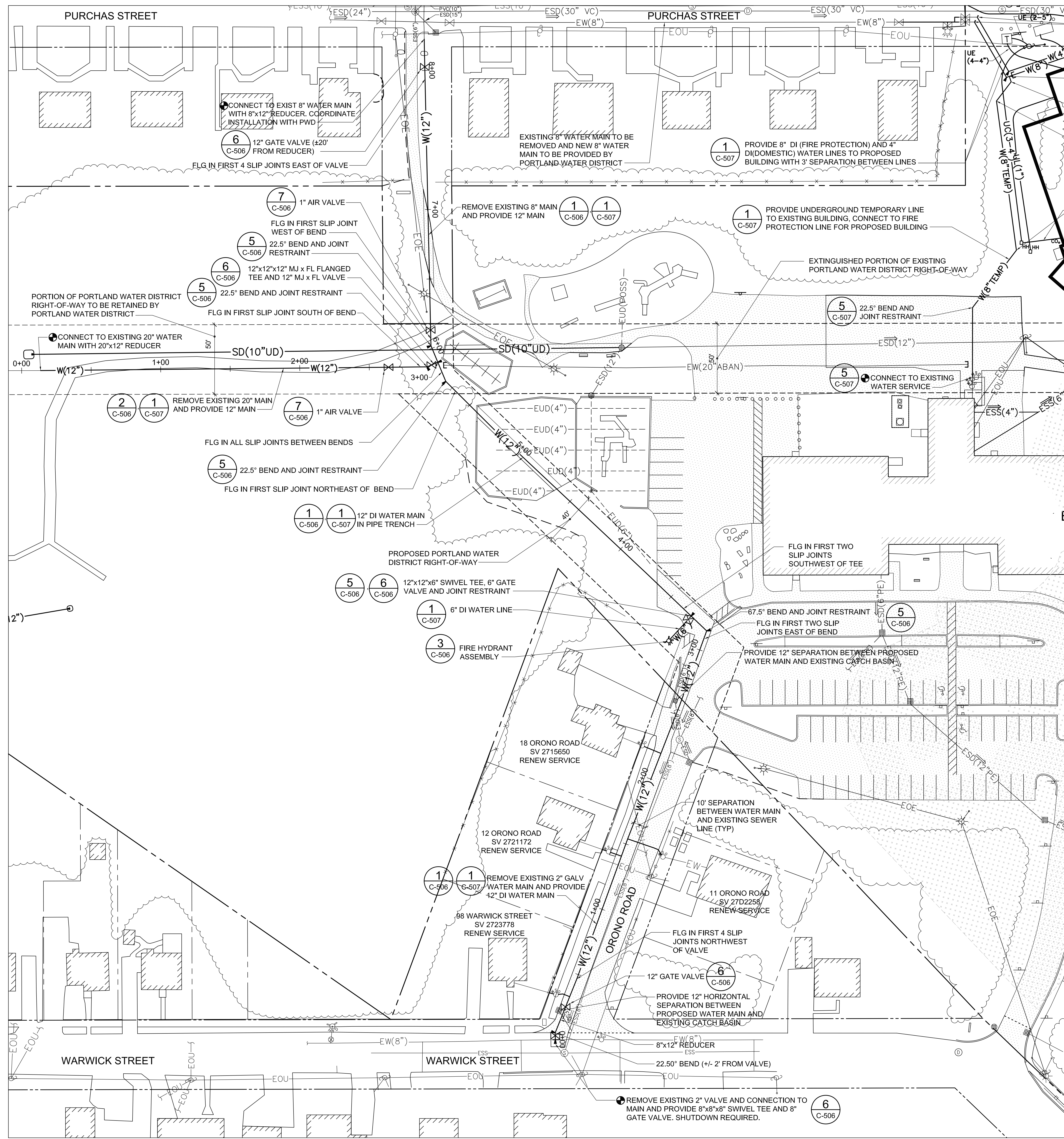
1 WATER MAIN CROSS CONNECTION-UTILITY PLAN CU101, CU103, CU104 SCALE: 1"=30'
