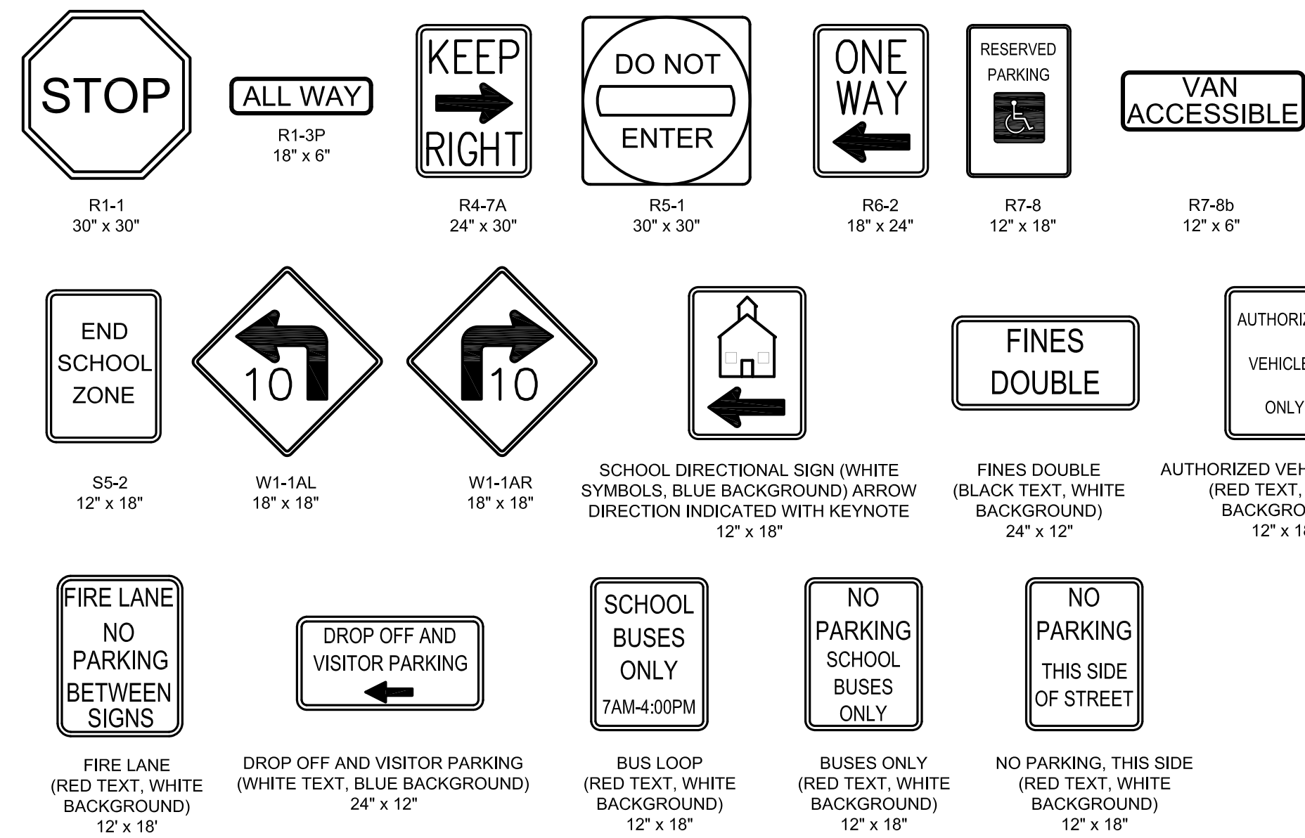
2 TRAFFIC SIGN DETAILS CM101.C-504 CM101 NOT TO SCALE
