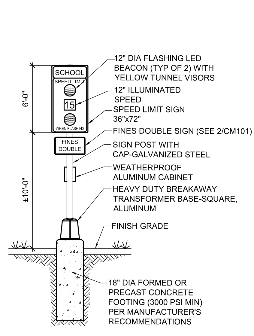
4 SPEED LIMIT BEACON CM101.C-504 CM101 NOT TO SCALE
