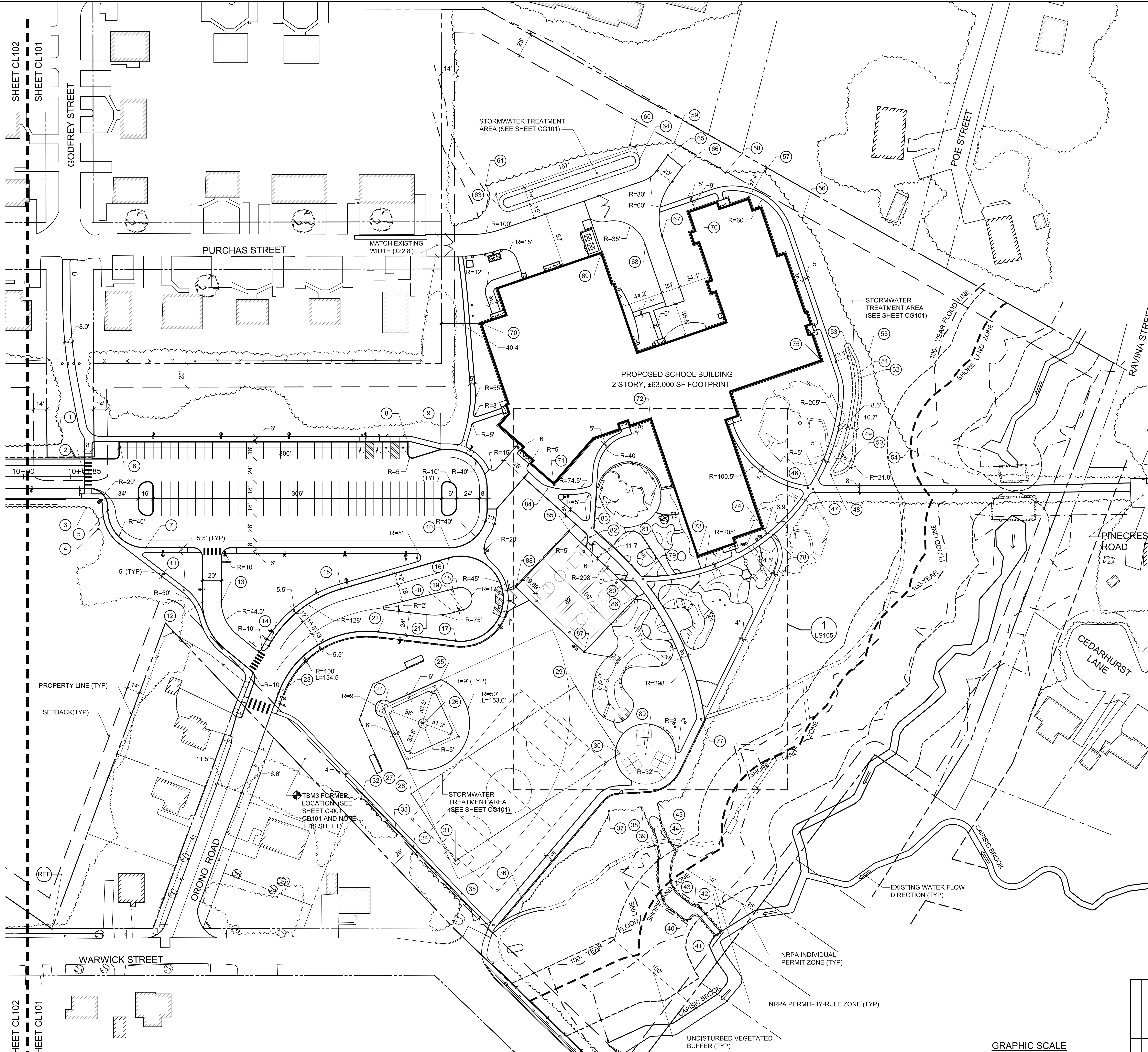
1 NORTH LAYOUT PLAN SCALE: 1"=40'
