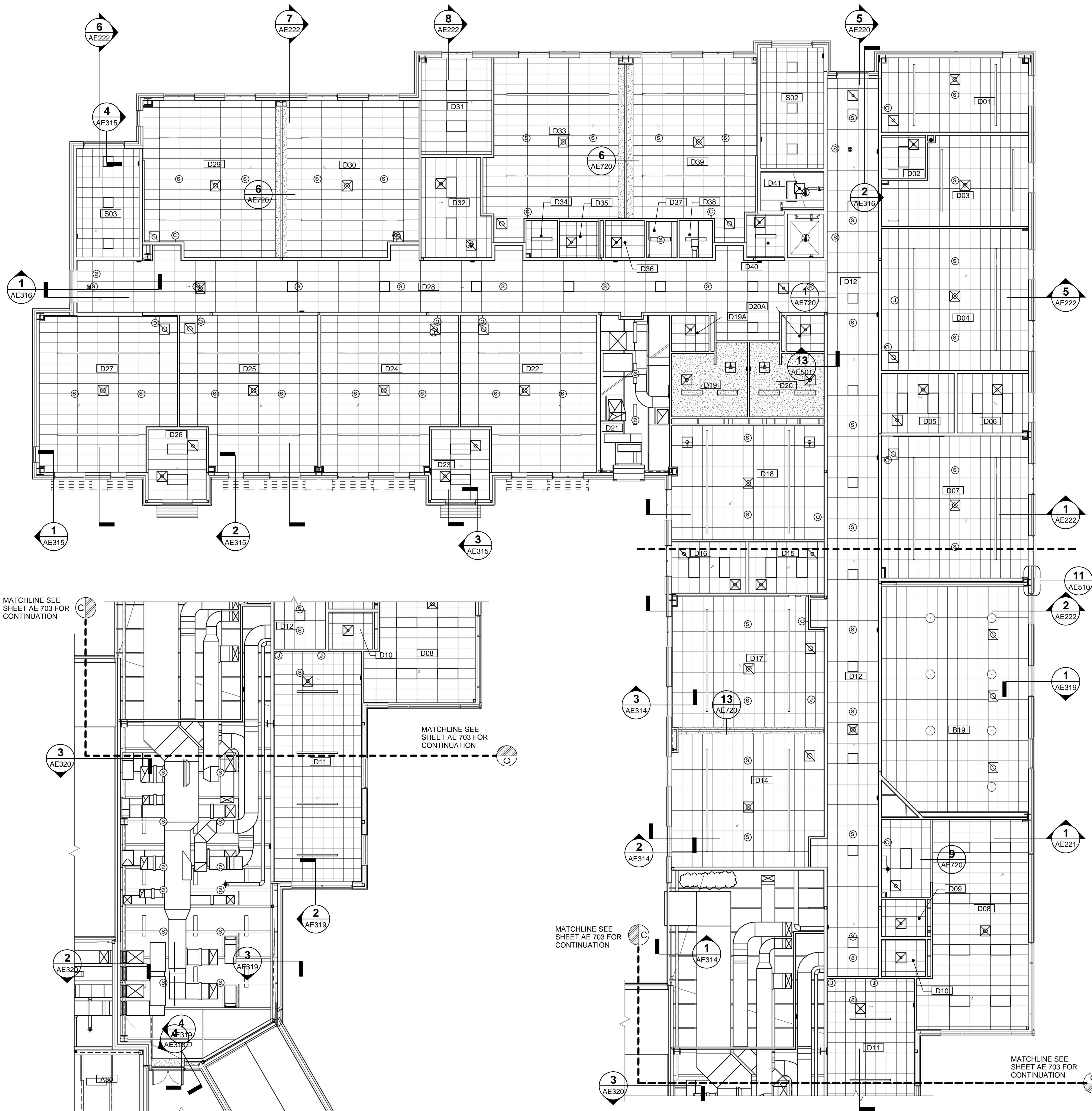
1 SECOND FLOOR REFLECTED CEILING PLAN AE201 AE704/ SCALE: 1/8" = 1'-0"
