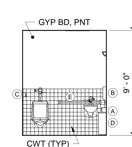
10 TOILET ROOM D09 - EAST ELEV AE422 SCALE: 1/4" = 1'-0"
