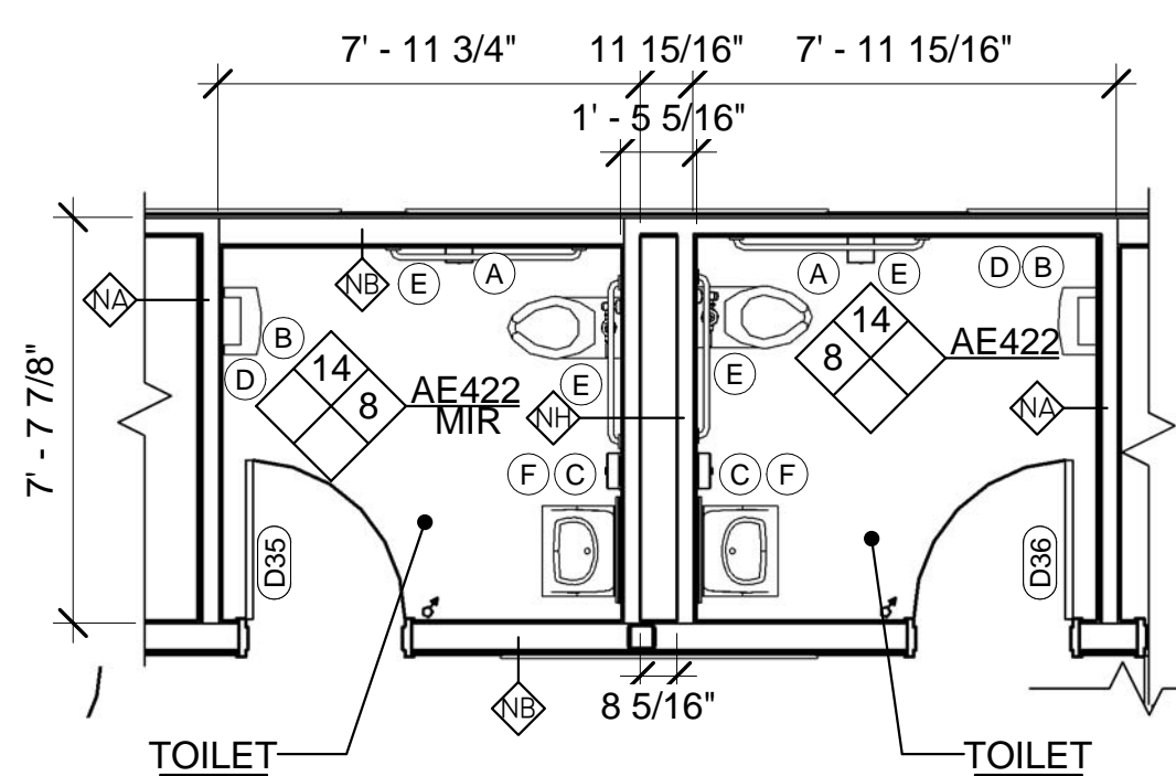
7 ENLARGED TOILET ROOM D35 AND D36 PLAN AE104/AE422 SCALE: 1/4" = 1'-0"
