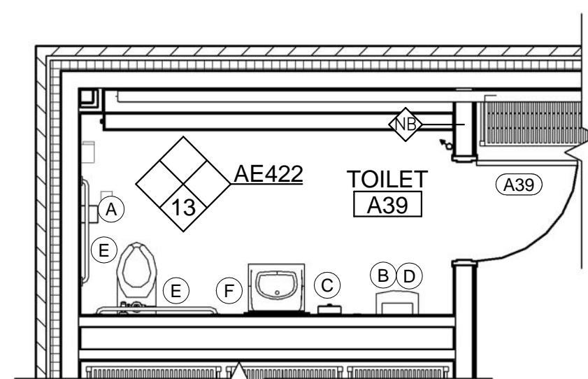
12 ENLARGED TOILET ROOM A39 PLAN AE101/AE422 SCALE: 1/4" = 1'-0"
