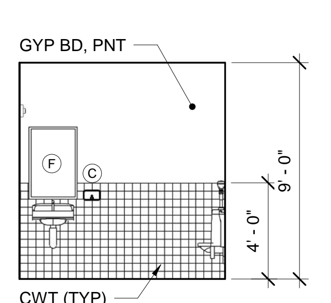
15 TOILET ROOM D09 - NORTH ELEV AE105/AE422 SCALE: 1/4" = 1'-0"
