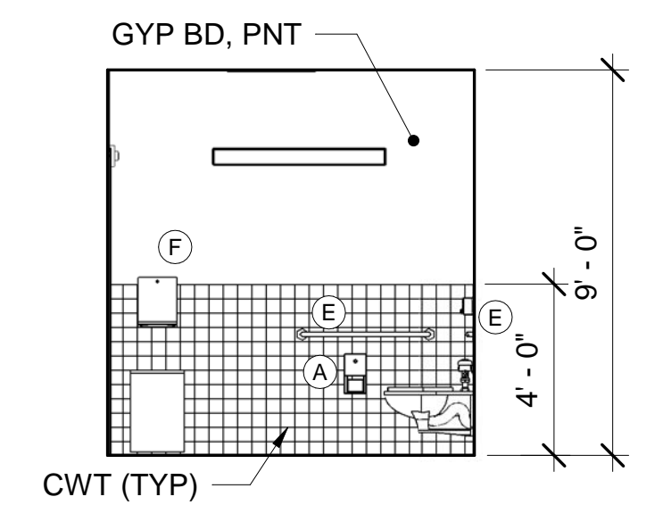
16 TOILET ROOM D10 - NORTH ELEV AE105/AE422 SCALE: 1/4" = 1'-0"
