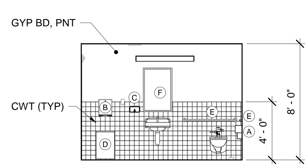
13 TOILET ROOM A39 - SOUTH ELEV AE422 SCALE: 1/4" = 1'-0"
