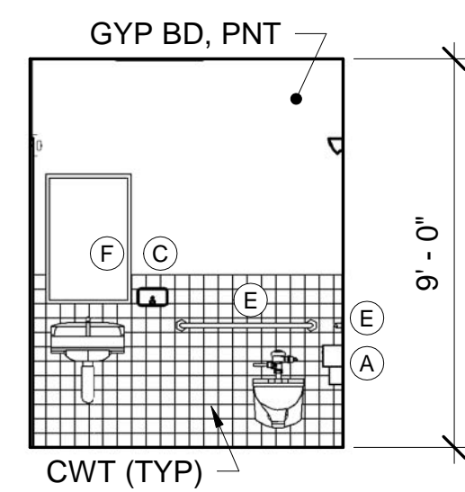
8 TOILET ROOM D36 - WEST ELEV AE422 SCALE: 1/4" = 1'-0"
