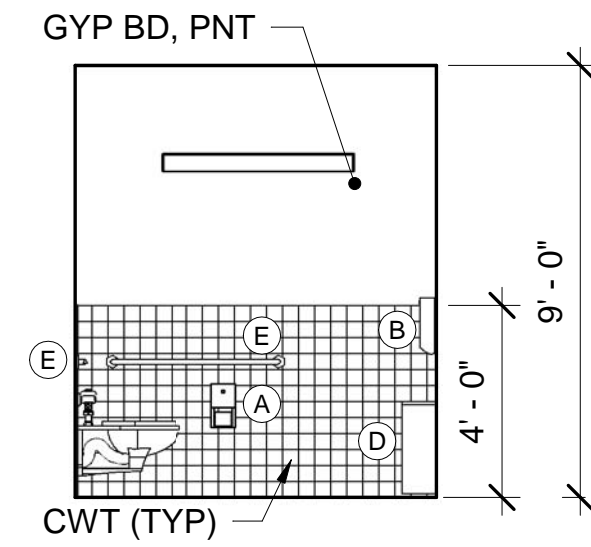
14 TOILET ROOM D36 - NORTH ELEV AE422 SCALE: 1/4" = 1'-0"
