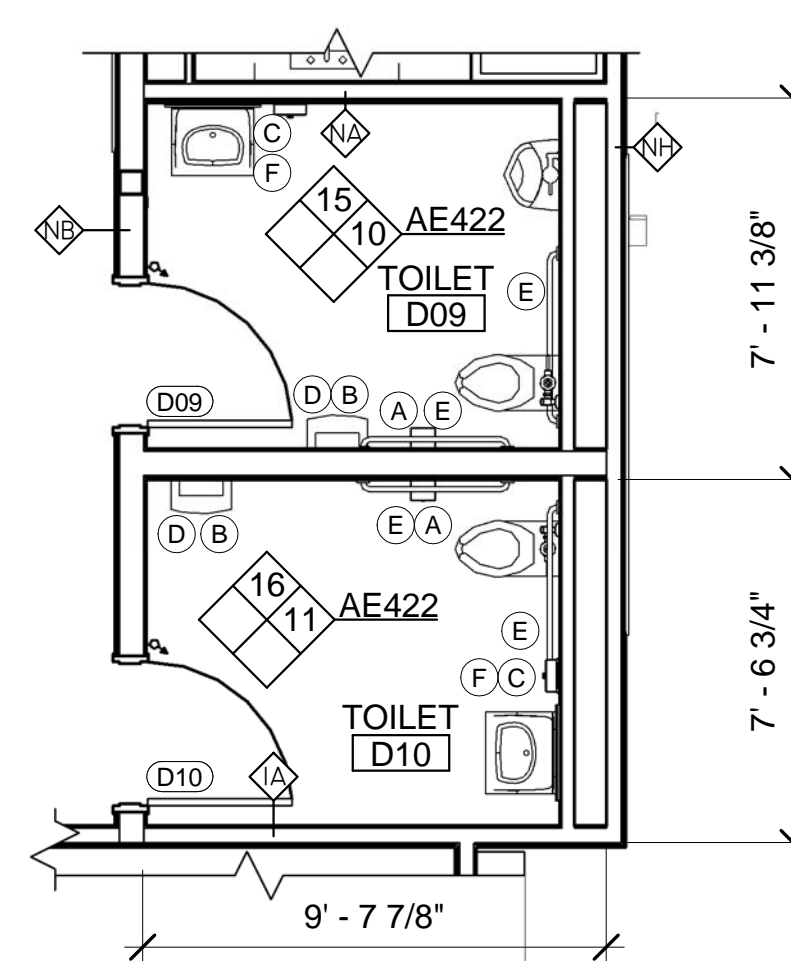
9 ENLARGED TOILET ROOM D09 AND D10 PLAN AE104/AE422 SCALE: 1/4" = 1'-0"
