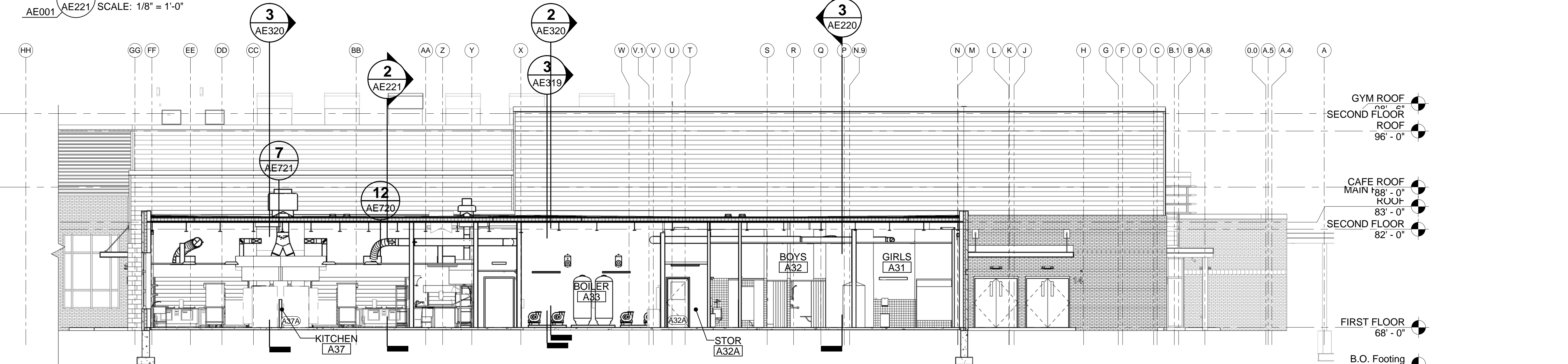
3 BUILDING SECTION THRU KITCHEN AND BOILER ROOM WING A-2
