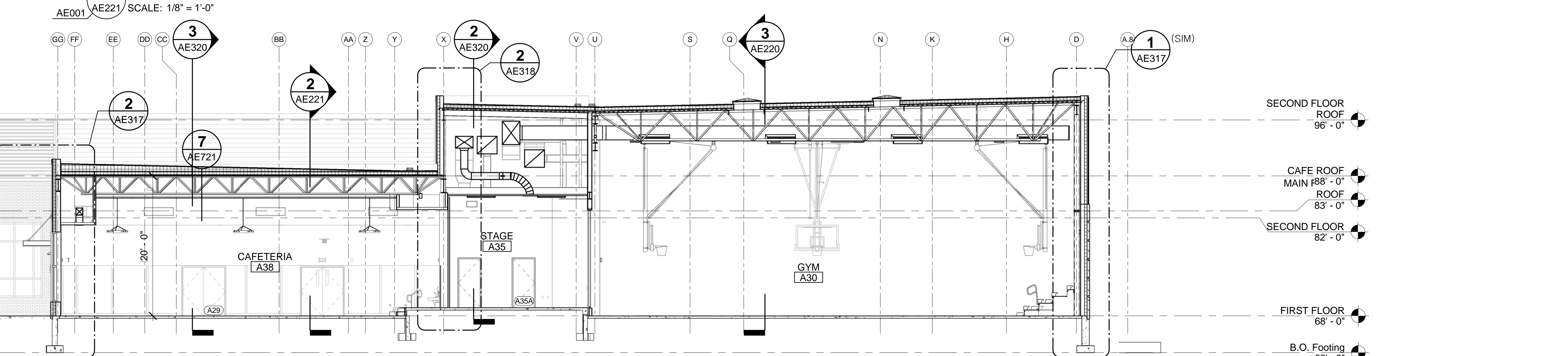
4 BUILDING SECTION THRU CAFETERIA AND GYM WING A-2
