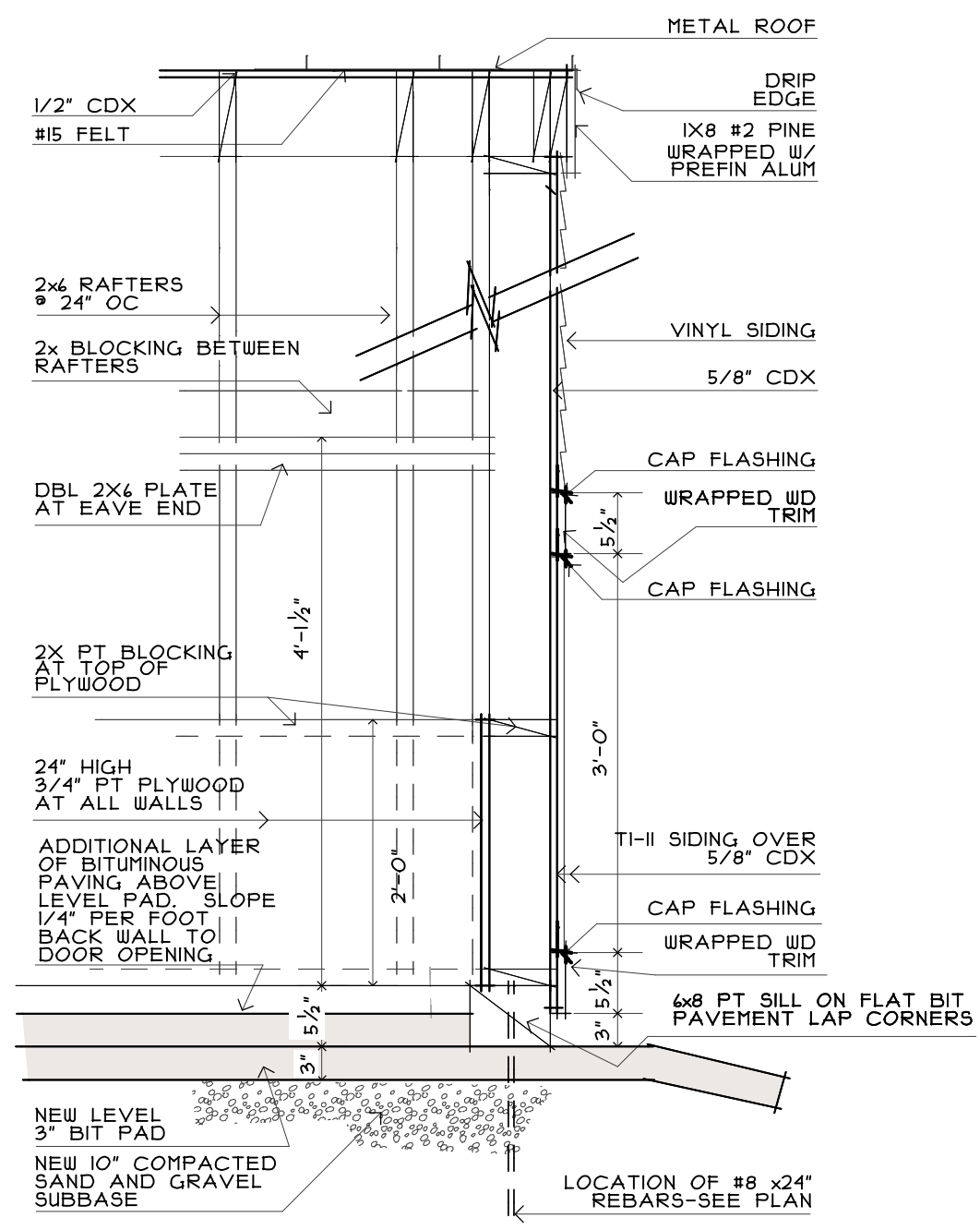
3 DETAIL AT RAKE OF SHED A4 SCALE: 3/4"=1'-0"
