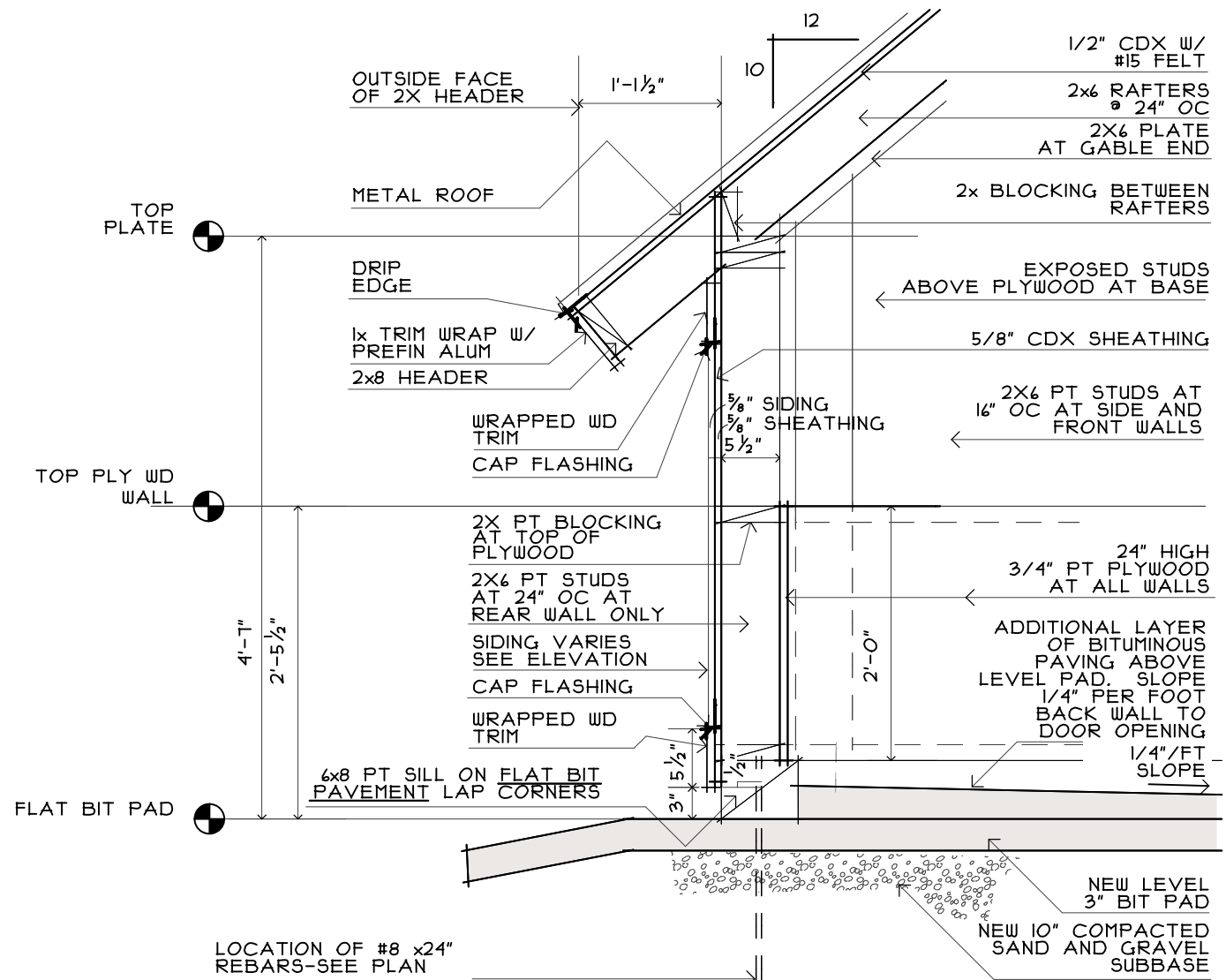
2 DETAIL AT LOW EAVE OF SHED A4 SCALE: 3/4"=1'-0"
