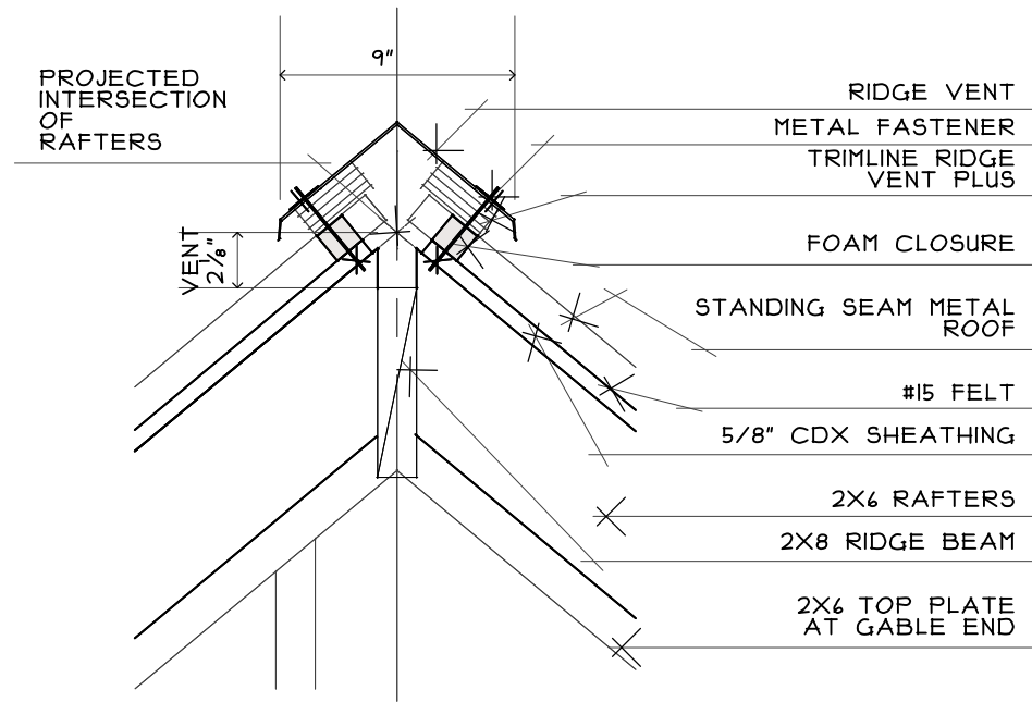
1 DETAIL AT RIDGE VENT A4 SCALE: 1 1/2"=1'-0"
