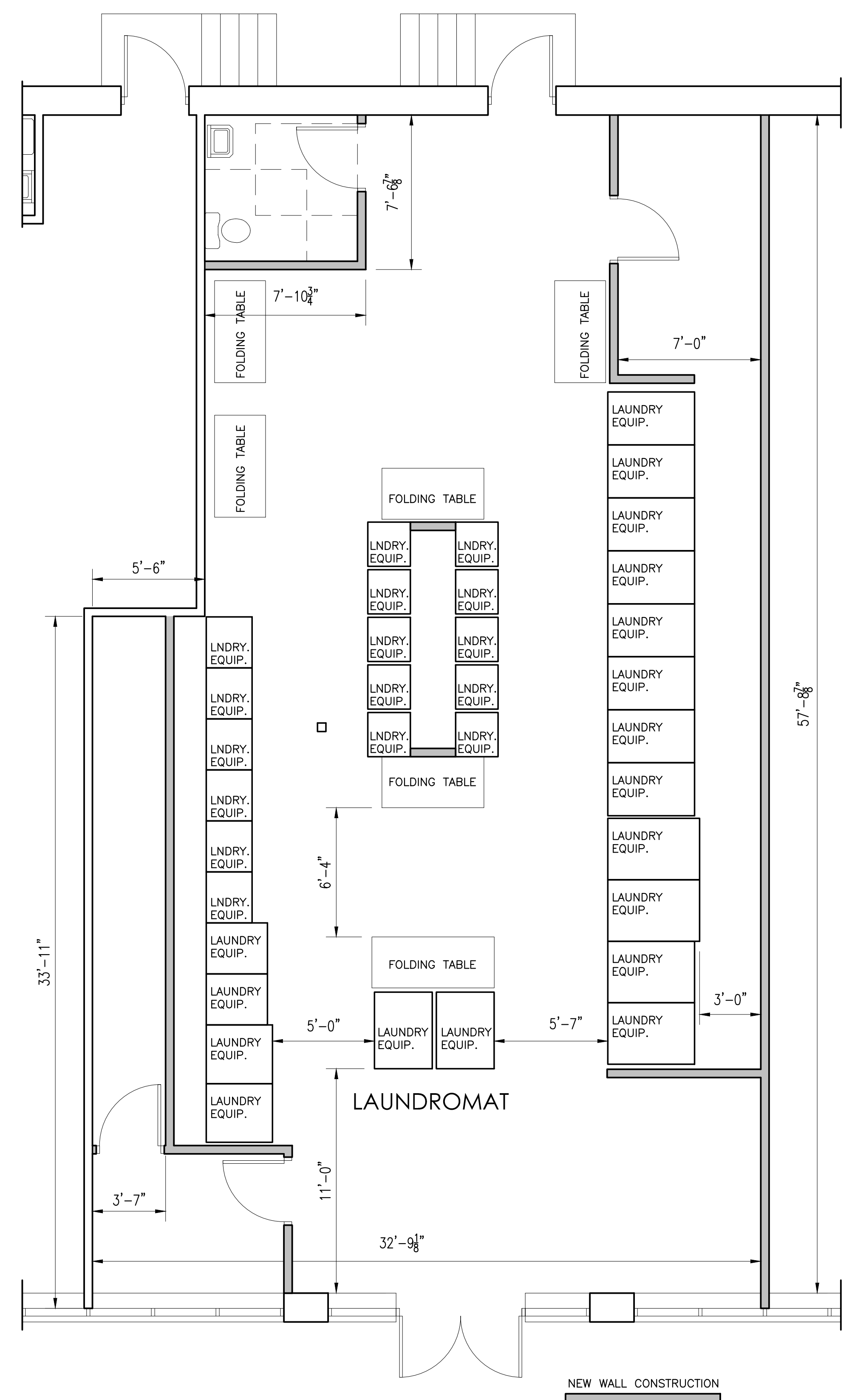
2 1/8"=1'-0" PROPOSED LAUNDROMAT LAYOUT
