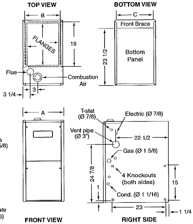
KG7SC 90+ High Efficiency Upflow/Horizontal Series
