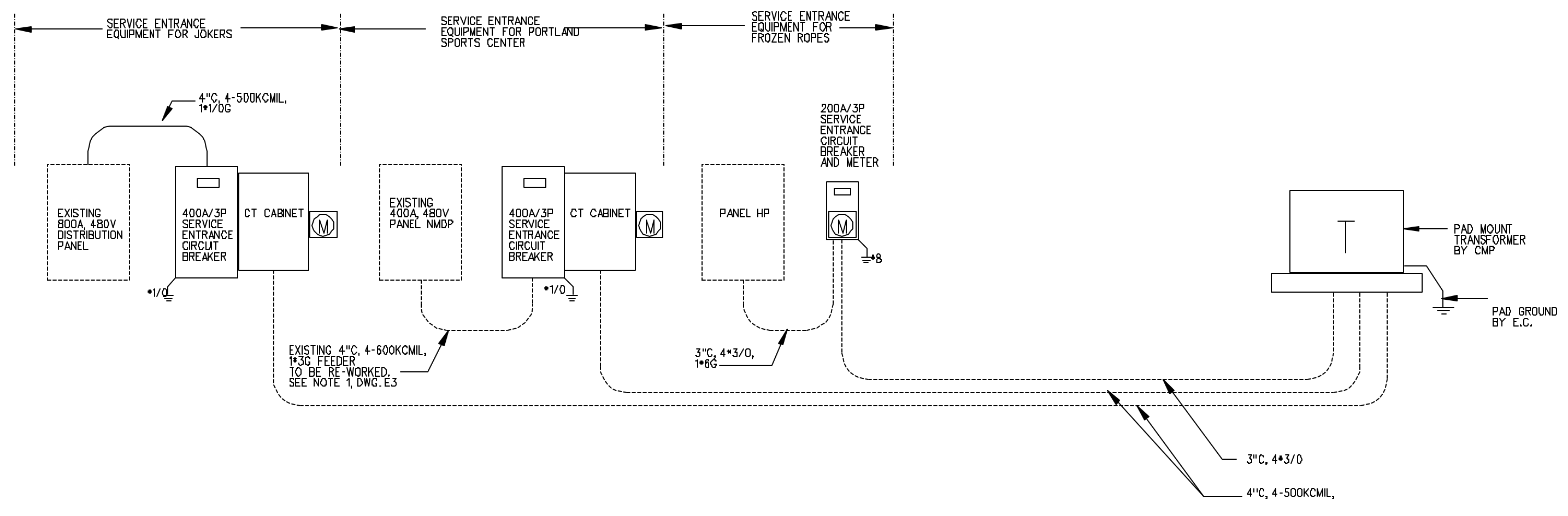
POWER RISER DIAGRAM NOT TO SCALE
