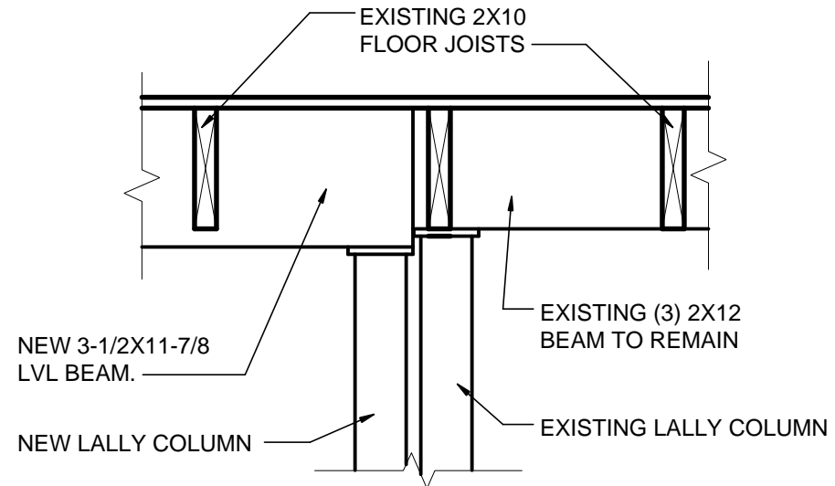
2 NEW BEAM TO LALLY COLUMN SCALE - 1" = 1'-0"
