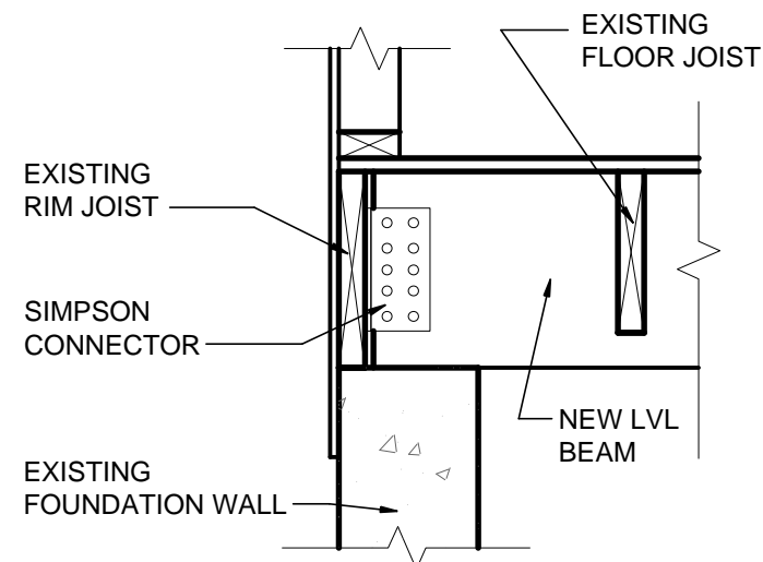
3 BEAM TO FOUNDATION WALL DETAIL SCALE - 1" = 1'-0"
