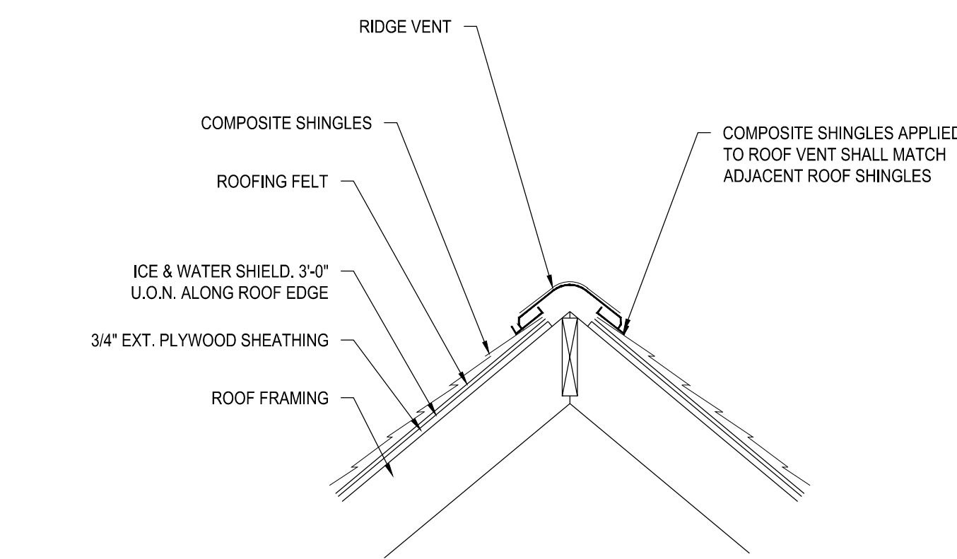
43 TYPICAL RIDGE VENT SCALE: NOT TO SCALE
