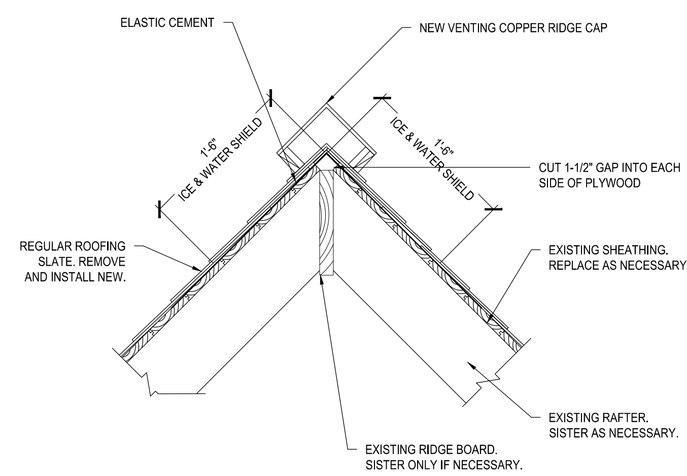
42 SLATE DETAIL AT RIDGE SCALE: NOT TO SCALE
