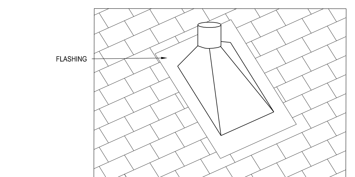
21 FLASHING FOR VENTILATION ON SLOPE OF SLATE ROOF SCALE: NOT TO SCALE
