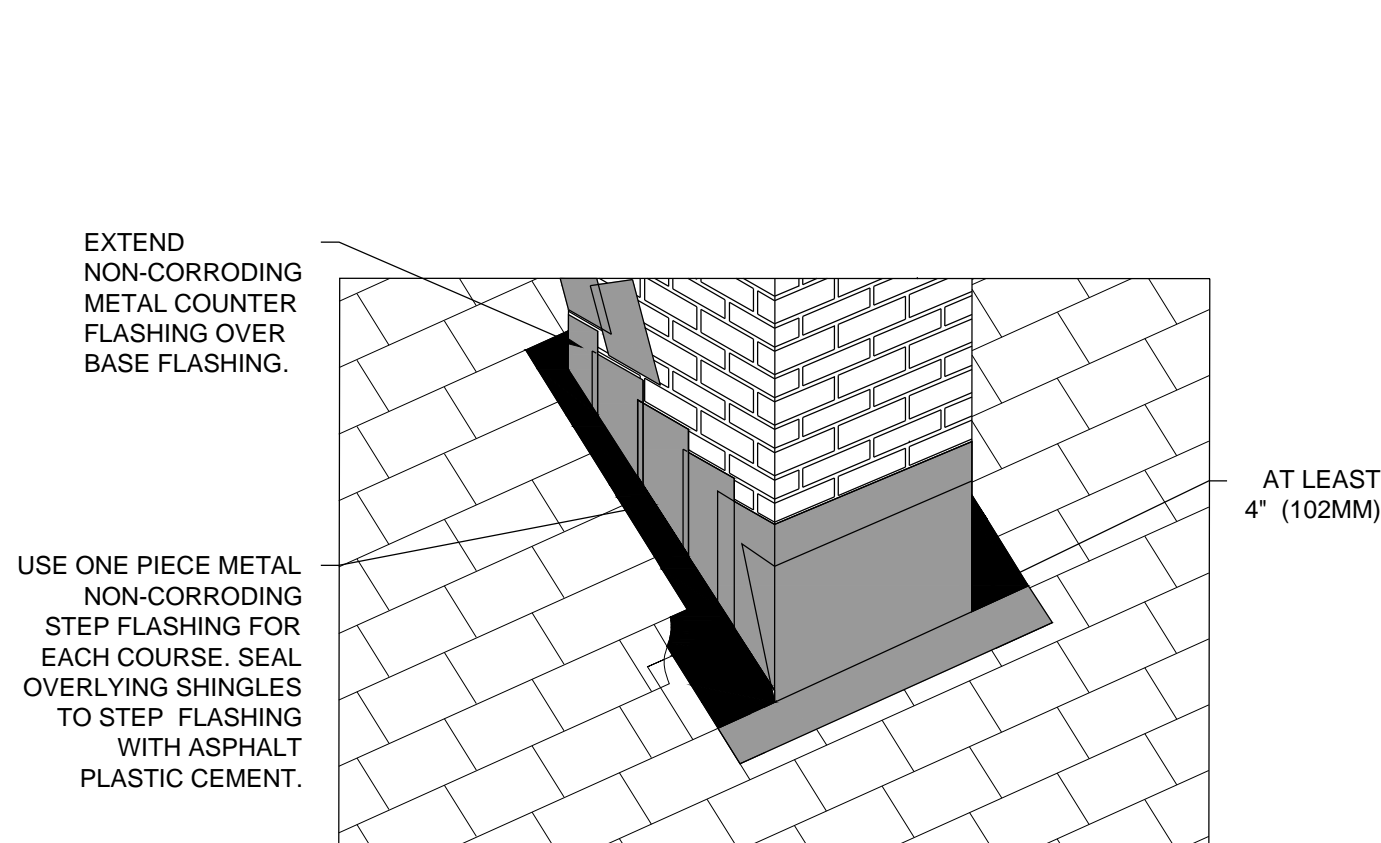
30 CHIMNEY FLASHING DETAIL ON SLOPE OF SLATE ROOF SCALE: NOT TO SCALE
