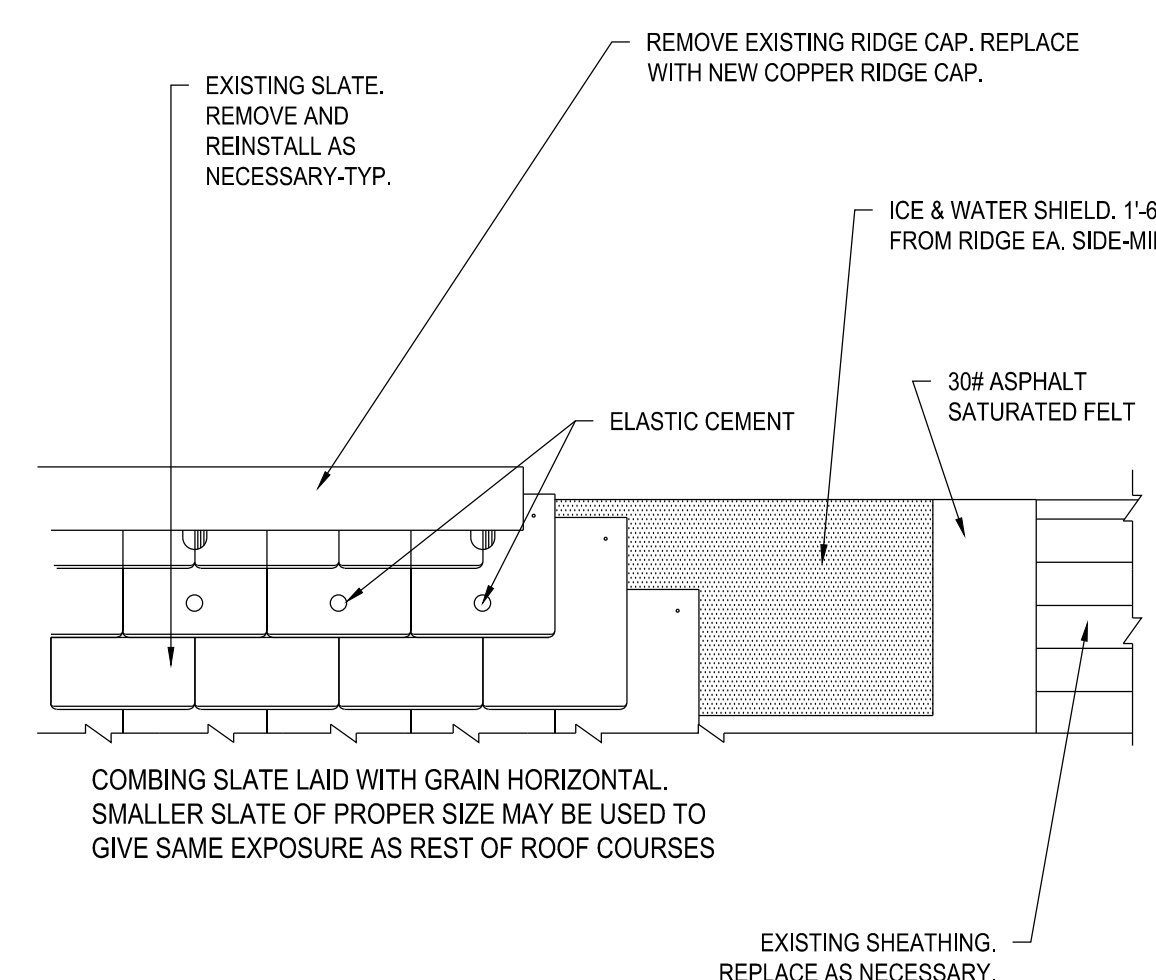
51 RIDGE DETAIL SCALE: NOT TO SCALE
