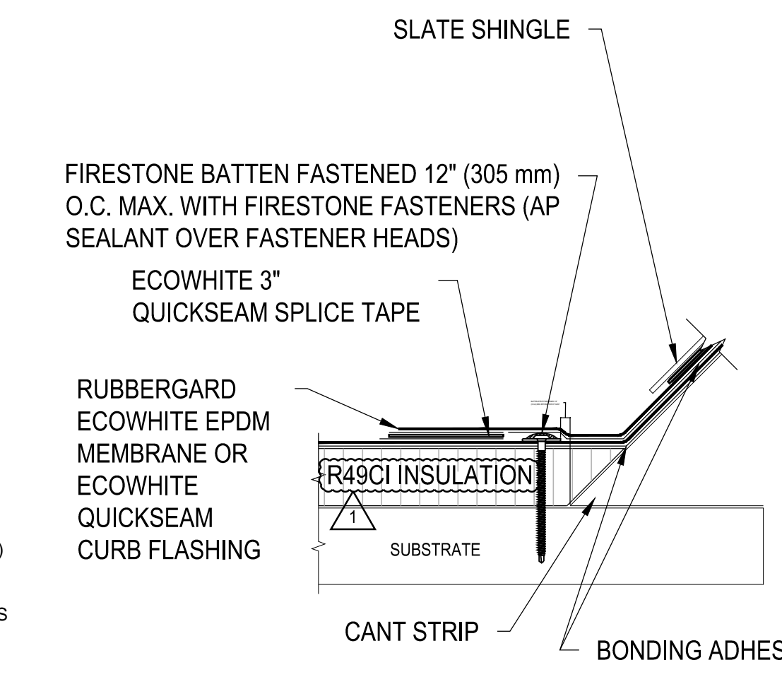
10 TIE-IN AT SLATE ROOF SCALE: NOT TO SCALE
