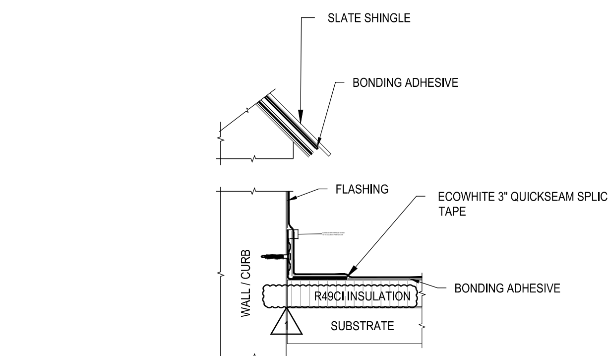
22 BASE TIE-IN AT SLATE ROOF SCALE: NOT TO SCALE
