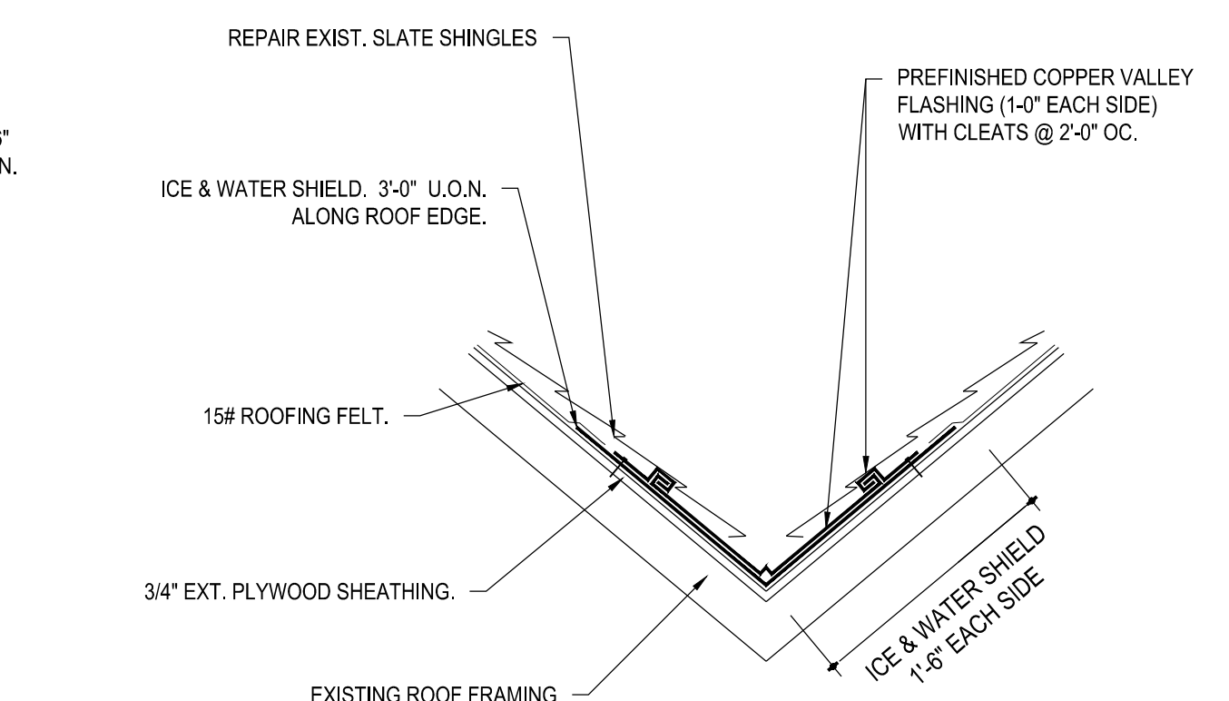
41 TYPICAL VALLEY FLASHING SCALE: NOT TO SCALE
