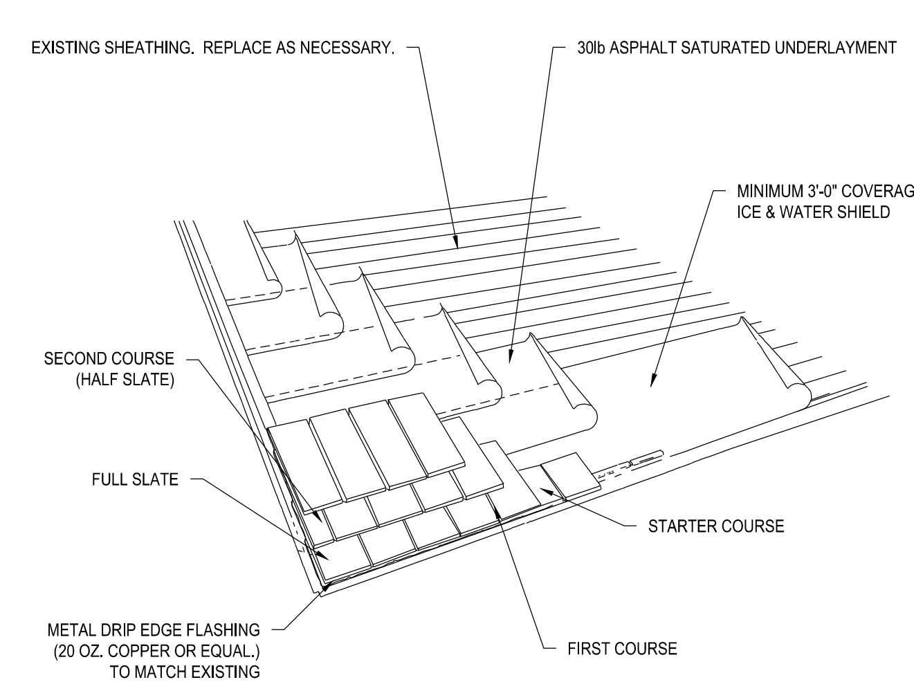
23 SLATE DETAIL AT EAVES SCALE: NOT TO SCALE
