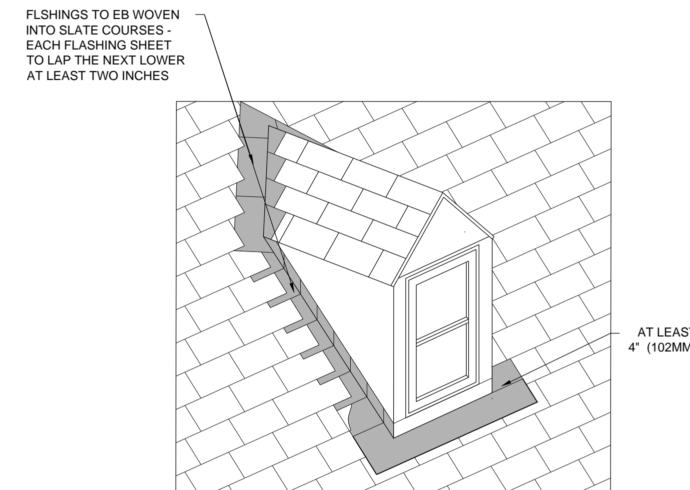
31 BUILT IN BASE FLASHING FOR DORMER WINDOW ON SLATE ROOF SCALE: NOT TO SCALE
