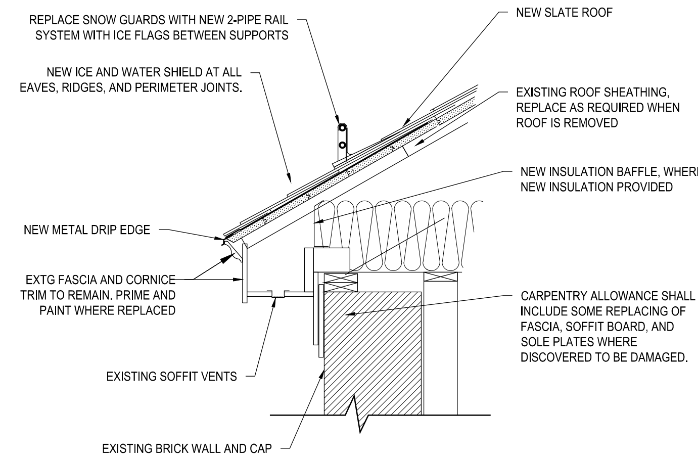
33 TYPICAL EAVE DETAIL SCALE: NOT TO SCALE
