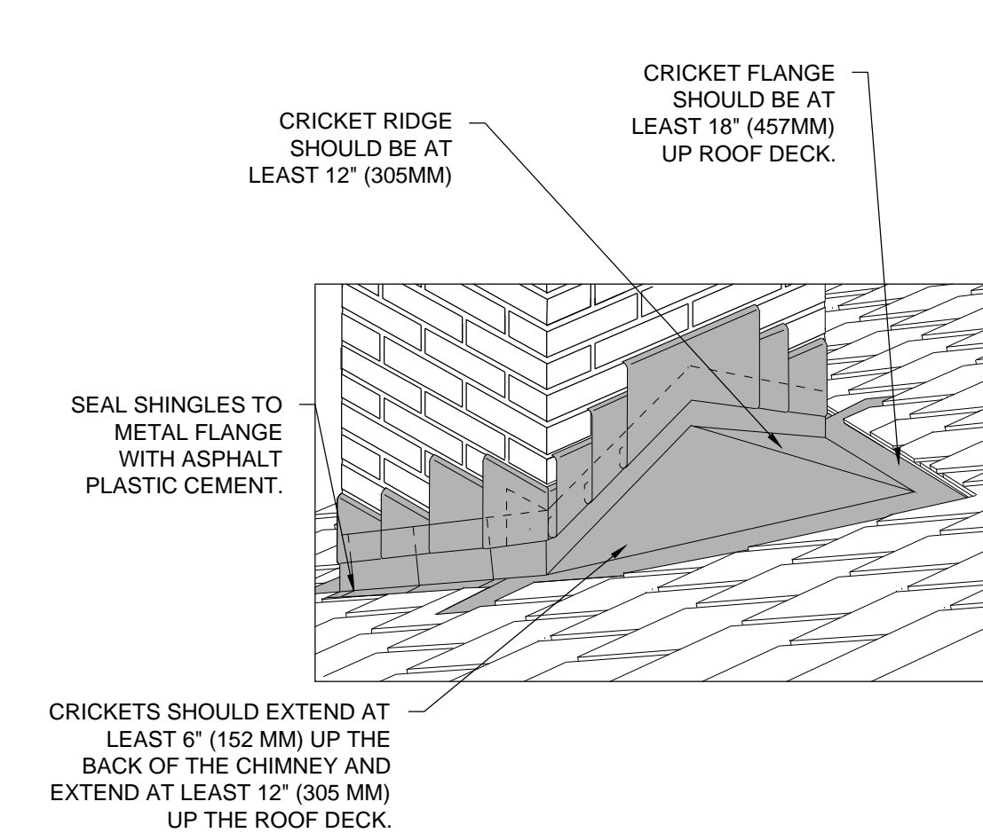
13 CHIMNEY CRICKET DETAIL SCALE: NOT TO SCALE
