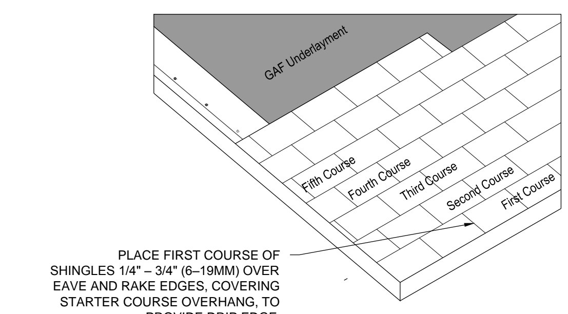
11 SHINGLE INSTALLATION DETAIL SCALE: NOT TO SCALE
