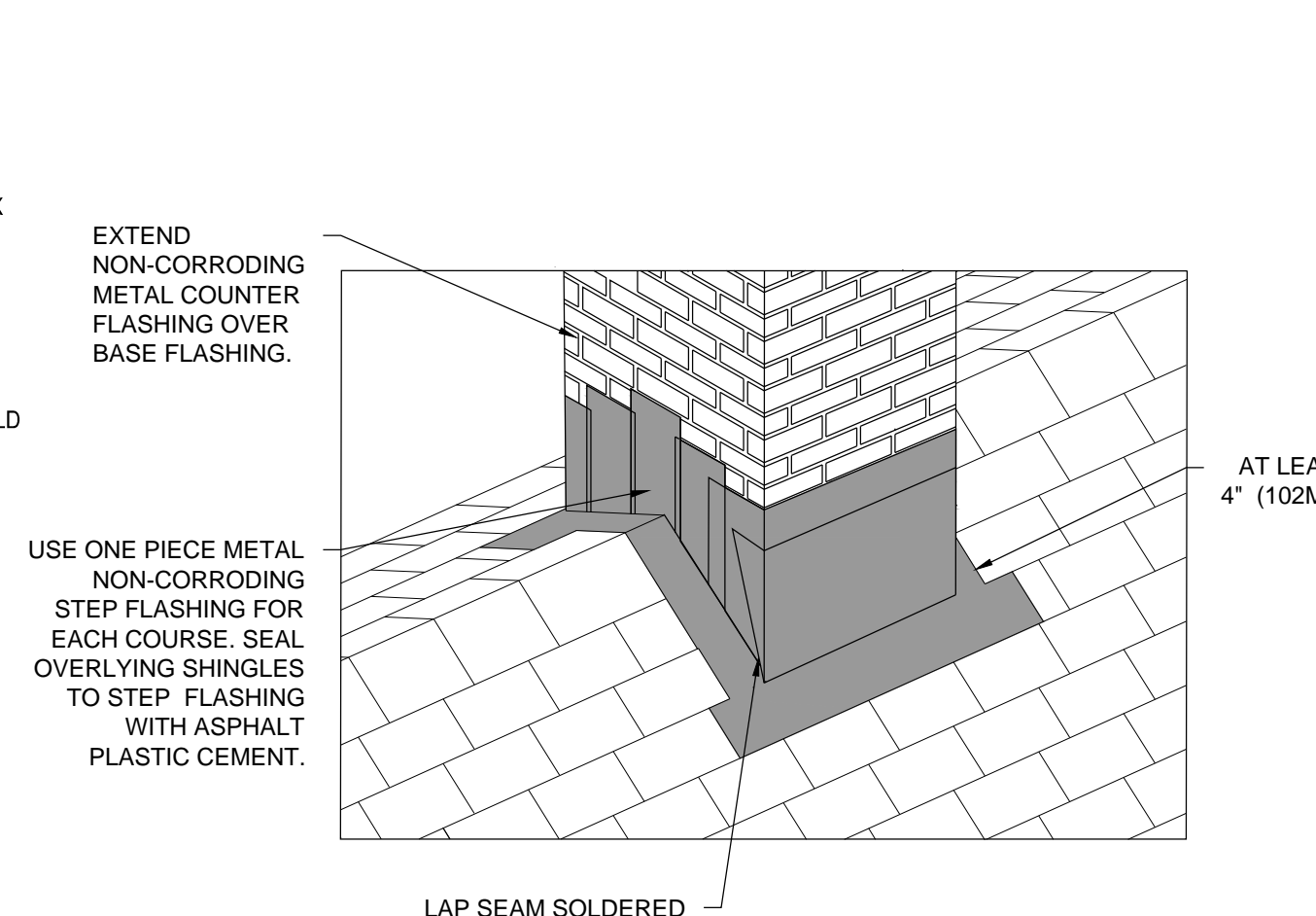
40 CHIMNEY FLASHING DETAIL ON RIDGE OF SLATE ROOF SCALE: NOT TO SCALE
