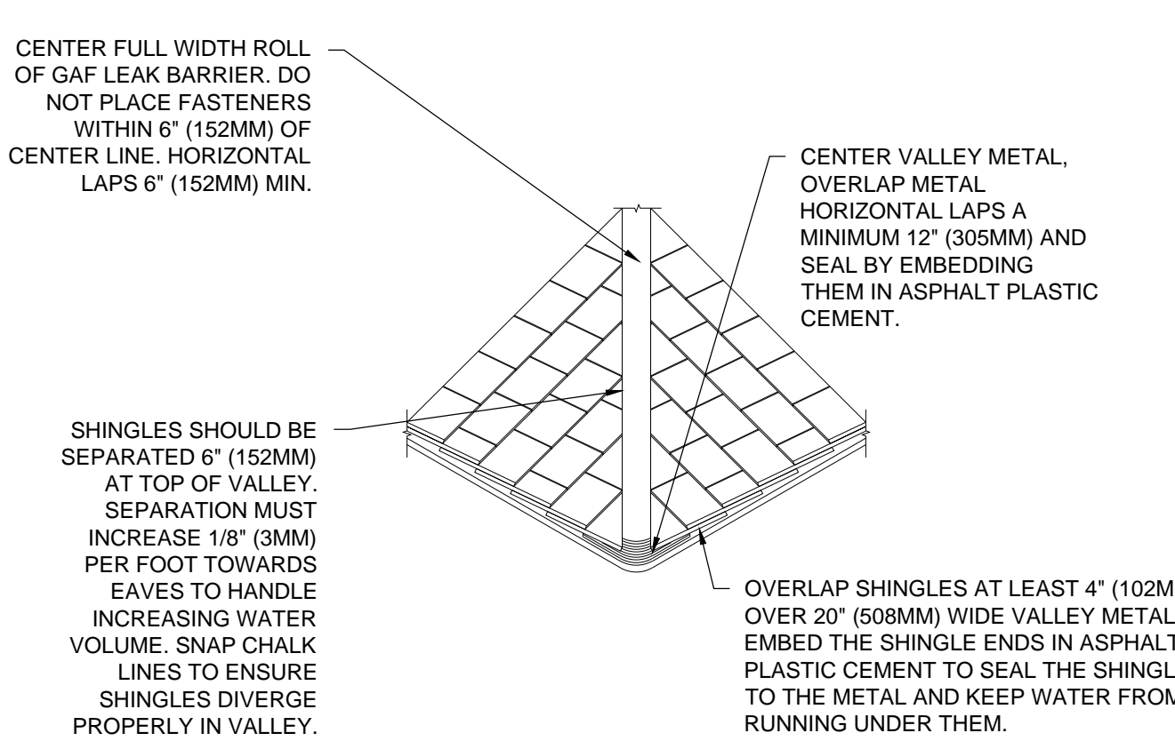
20 OPEN VALLEY DETAIL SCALE: NOT TO SCALE
