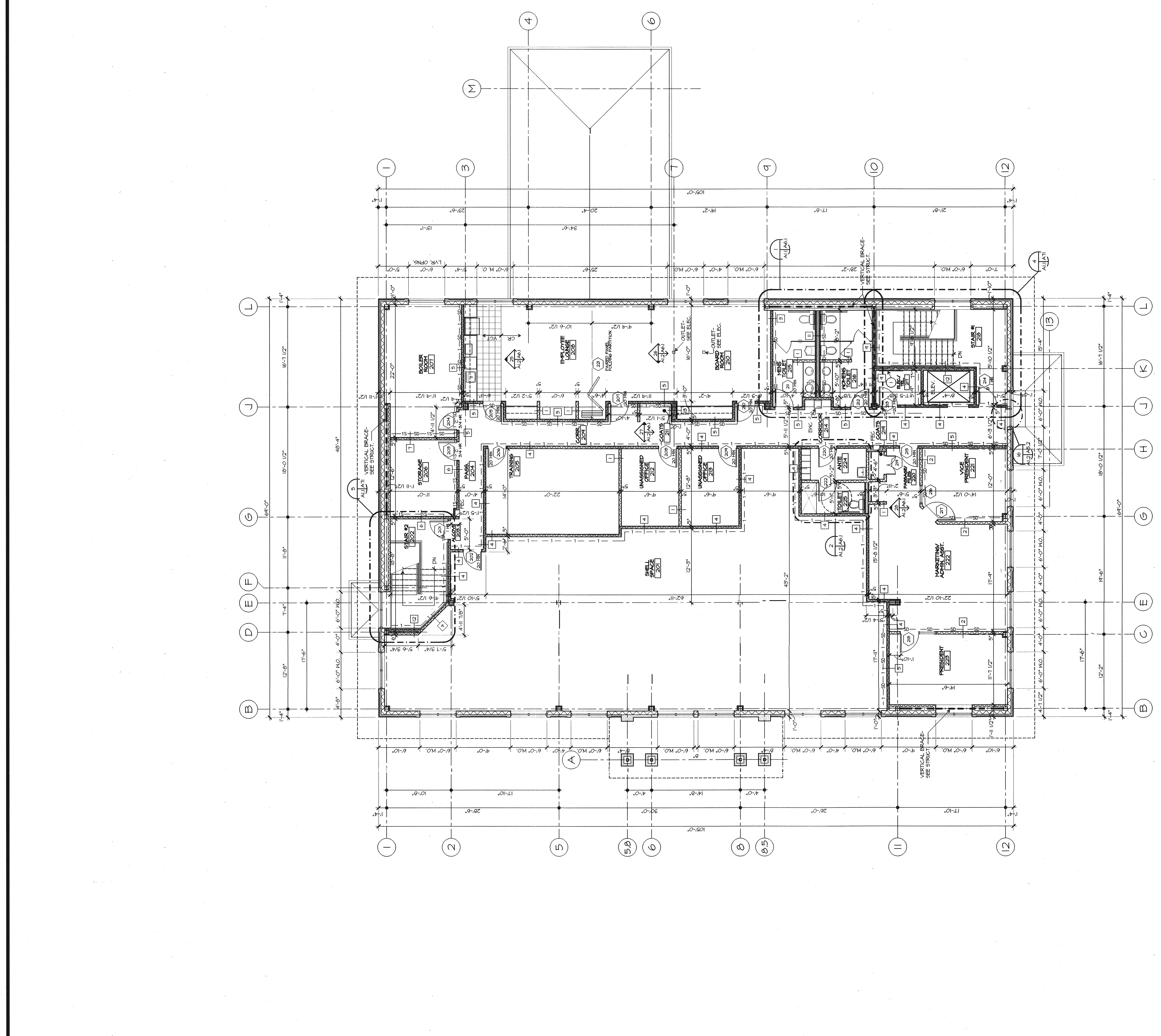
W N E S SECOND FLOOR PLAN SCALE: 1/8" = 1'-0"
