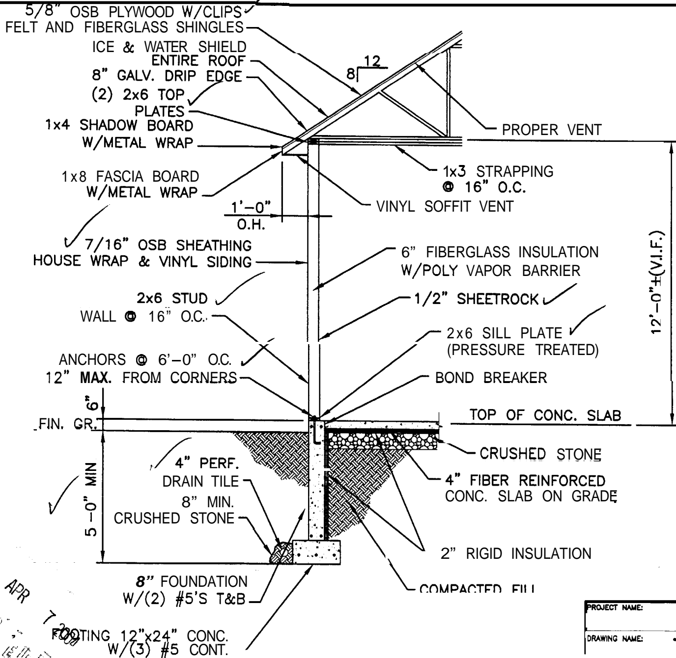
(A) TYPICAL WALL SECTION
