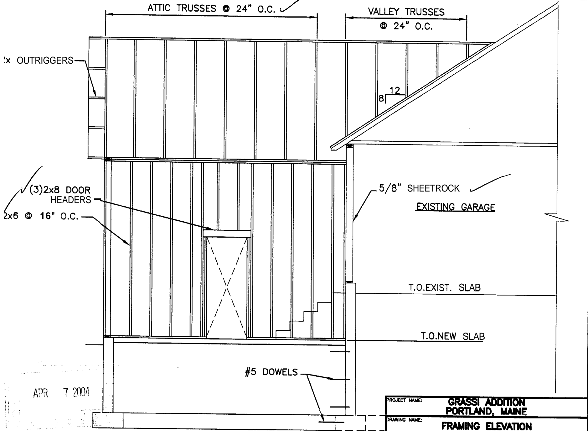
(A) FRAMING ELEVATION
