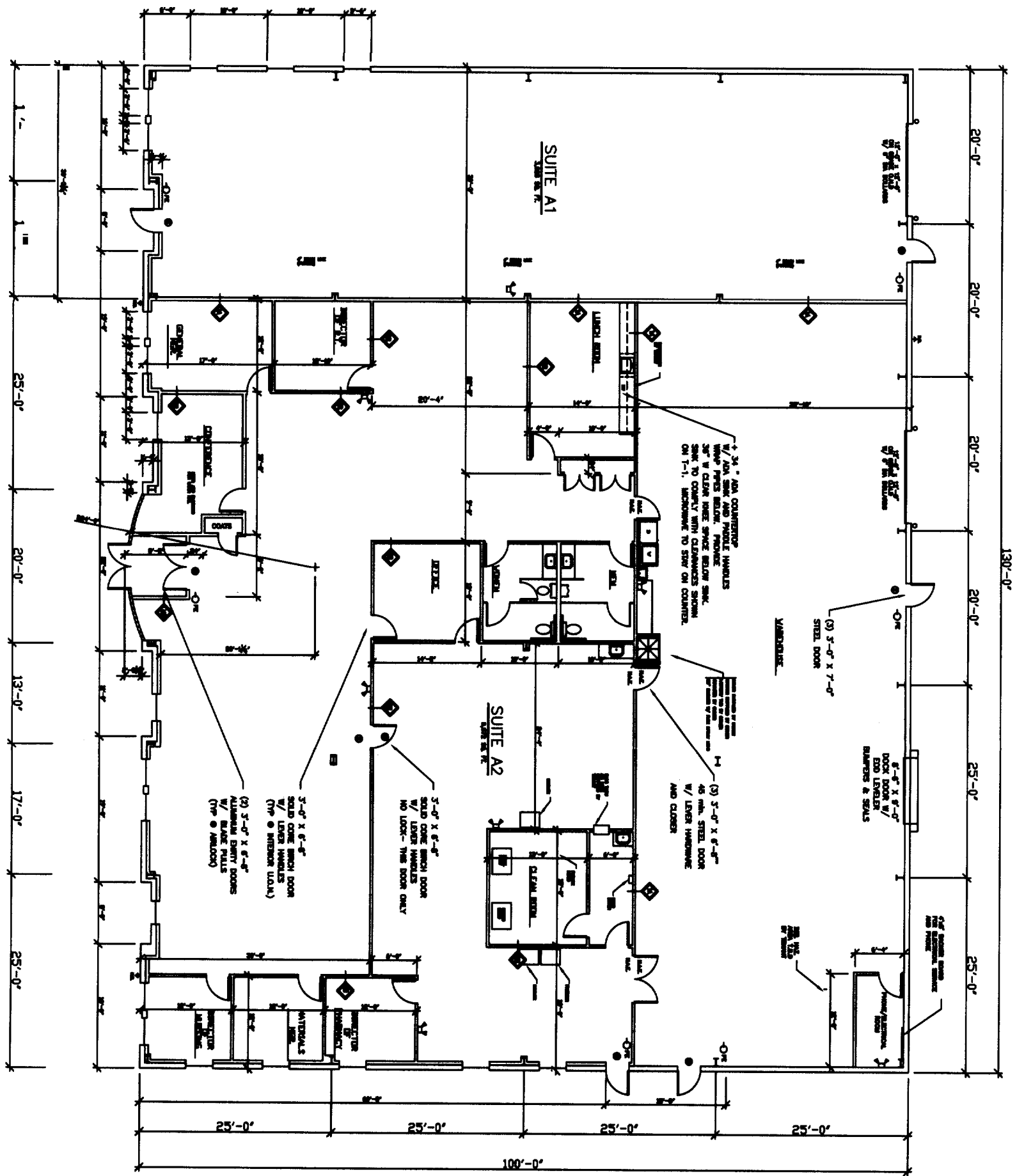
EXISTING FLOOR PLAN SCALE 1/16" = 1'-0"
