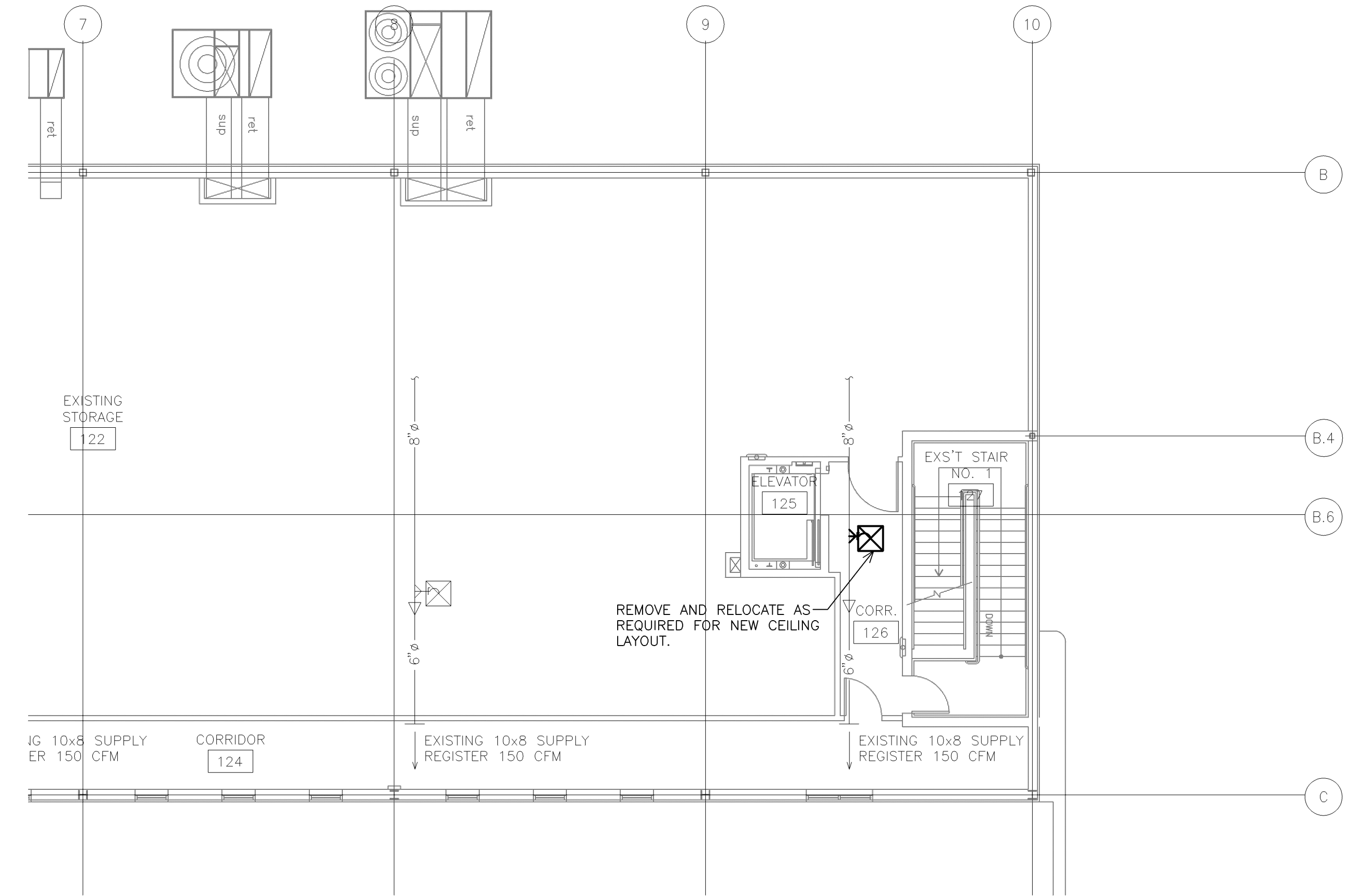
1 LEVEL TWO HVAC PLAN SCALE: 1/8" = 1'-0"
