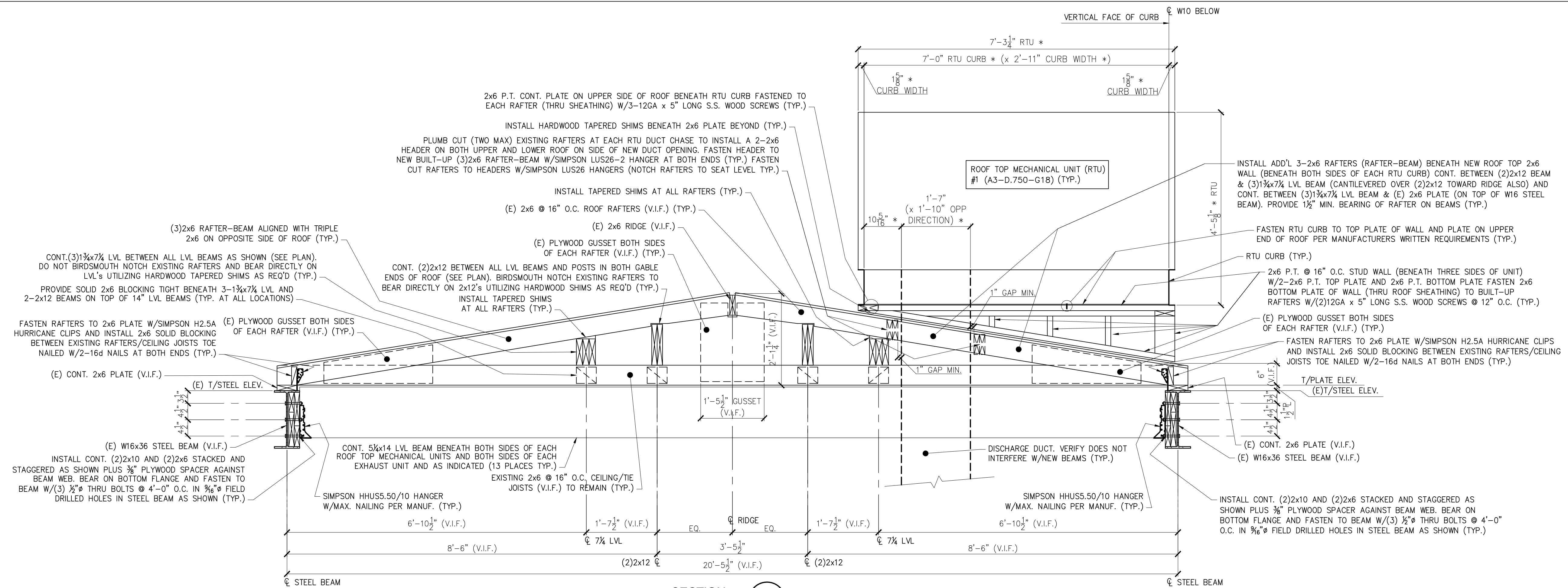
SECTION 1 3/4" = 1'-0"
