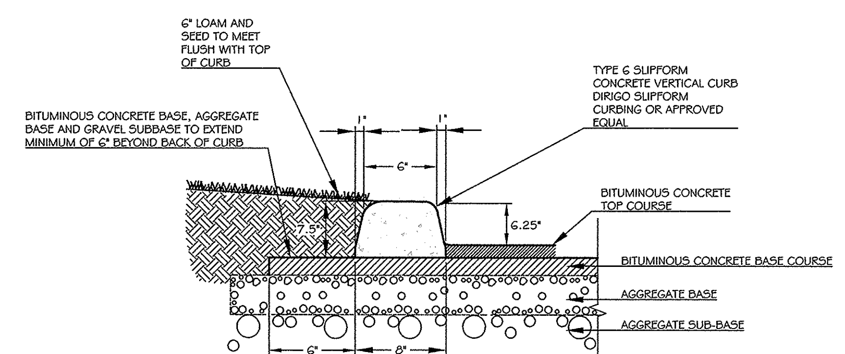
7 VERTICAL CURB DETAIL (SLIPFORM CONCRETE OR BIT. CONCRETE) NOT TO SCALE
