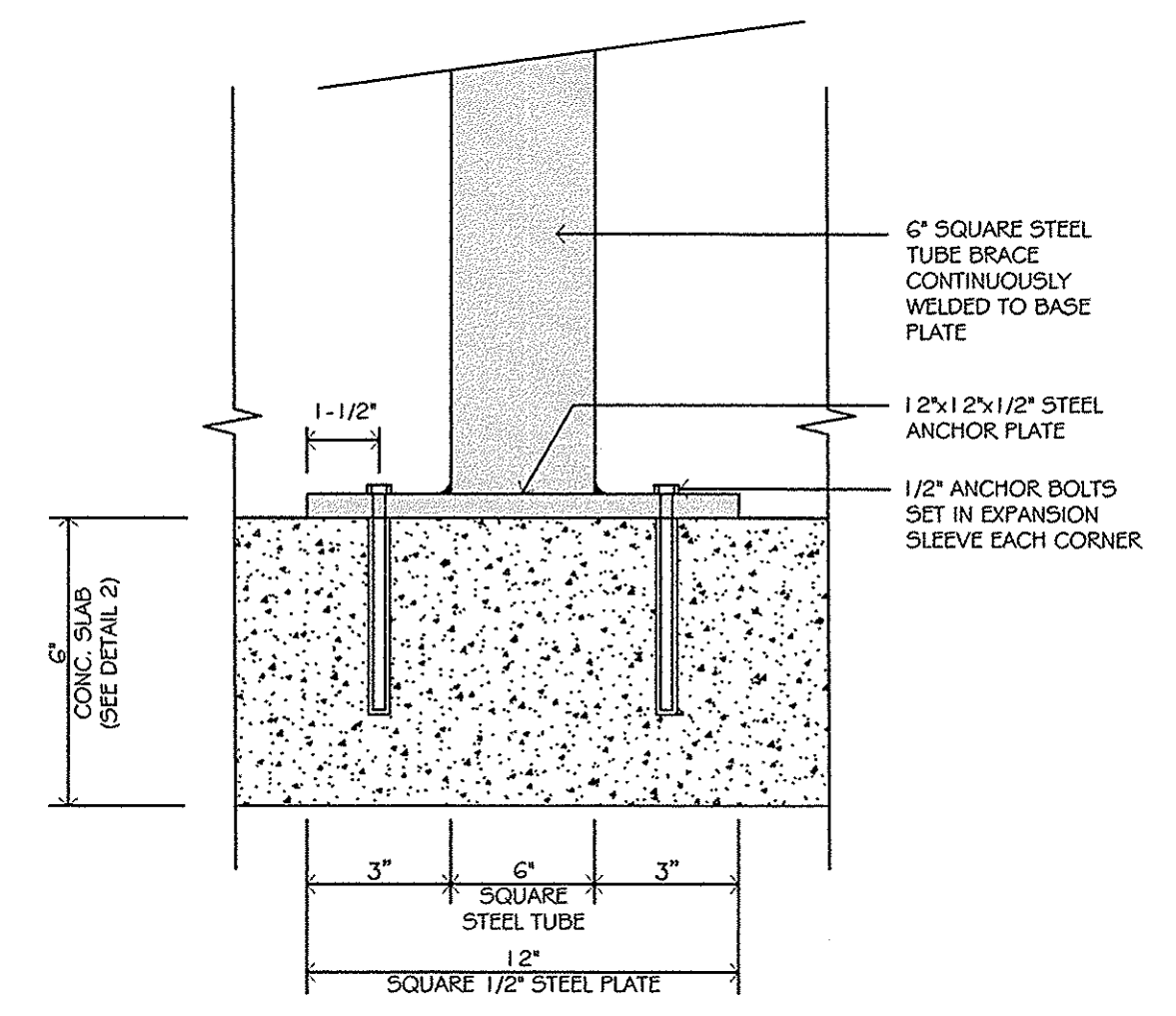
5 BASE PLATE / STEEL POST DETAIL NOT TO SCALE
