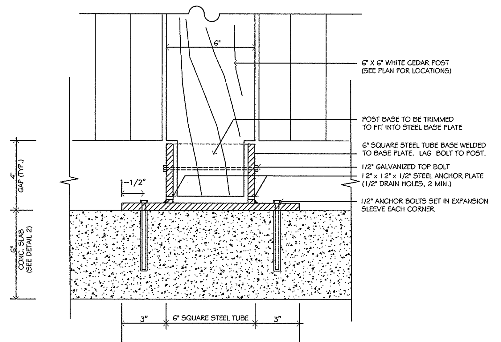
4 BASE PLATE / WOOD POST DETAIL NOT TO SCALE
