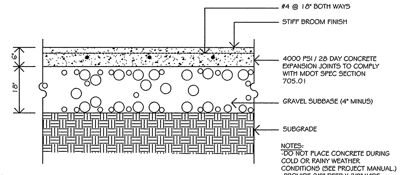
2 CONCRETE PAD AT DUMPSTER PAD NOT TO SCALE
