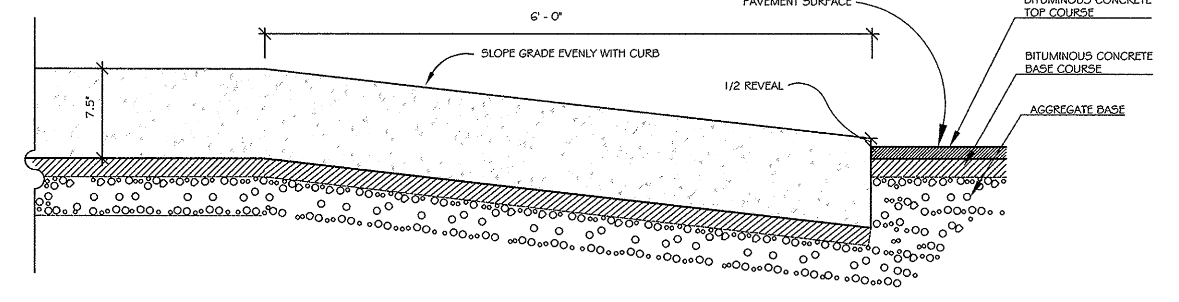
8 CURB TIPDOWN DETAIL (SLIPFORM CONCRETE OR BIT. CONCRETE) NOT TO SCALE
