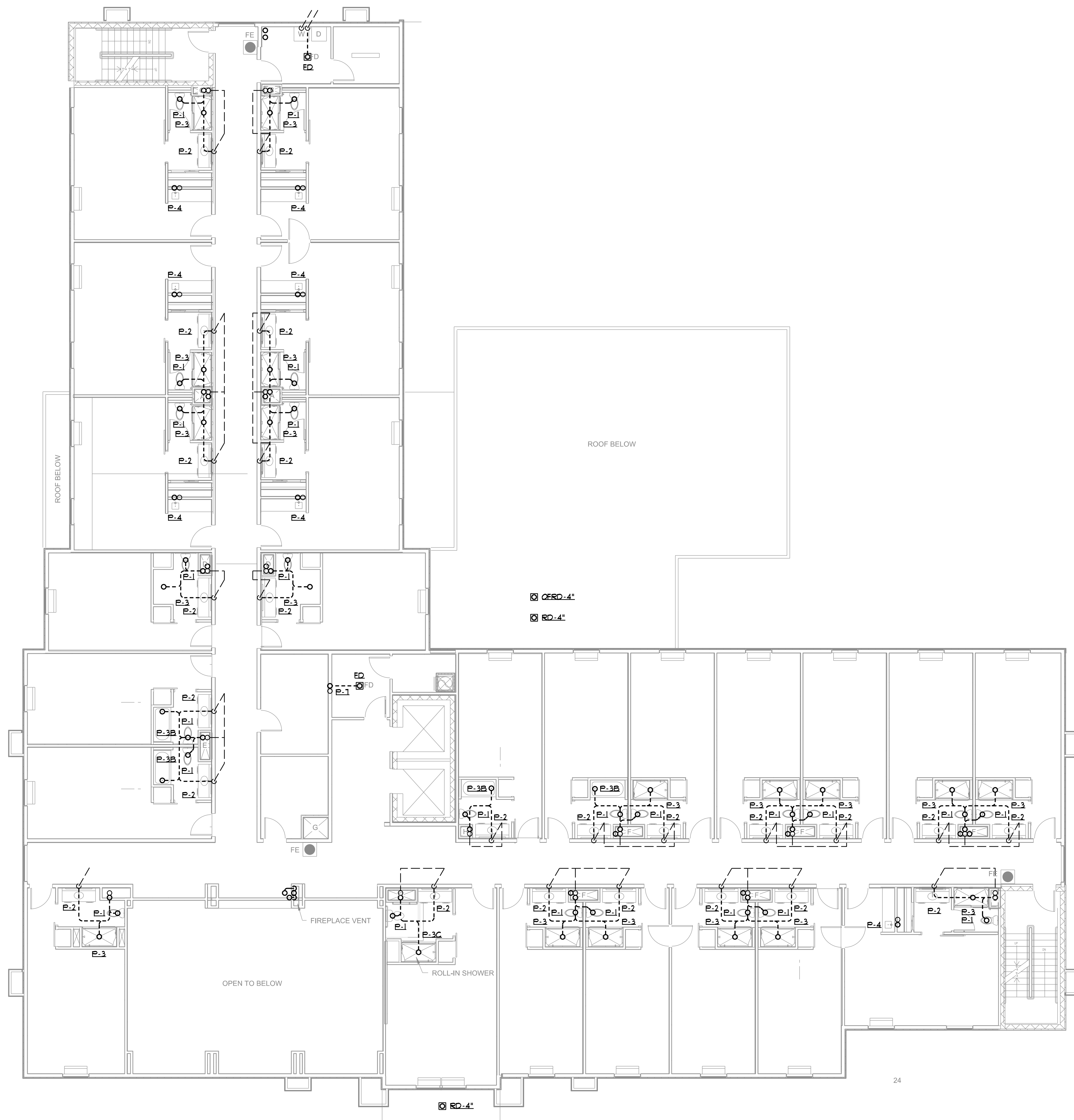
SECOND FLOOR SANITARY PLUMBING PLAN SCALE - 1/8"=1'-0"
