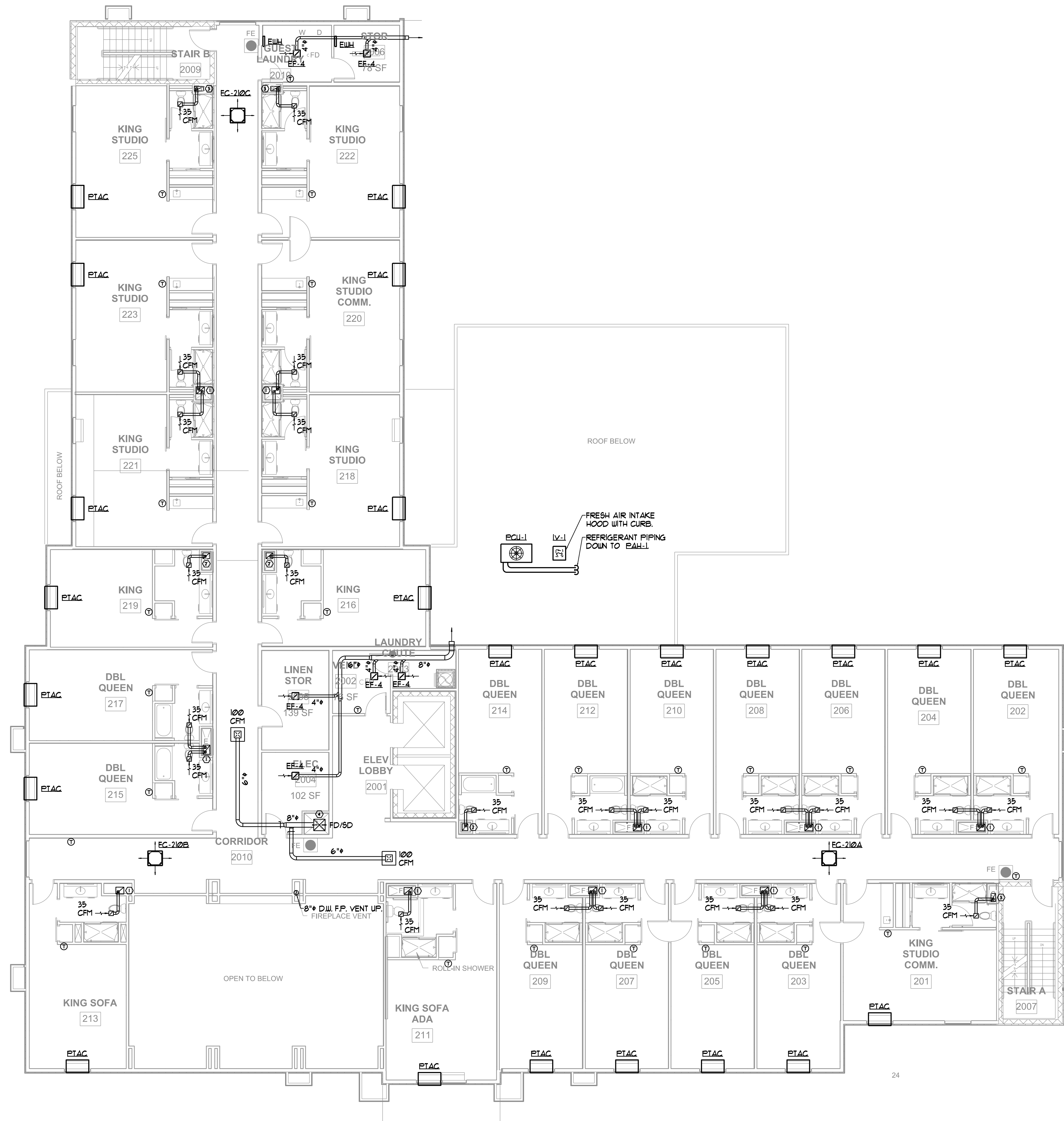
SECOND FLOOR MECHANICAL PLAN SCALE - 1/8" = 1'-0"
