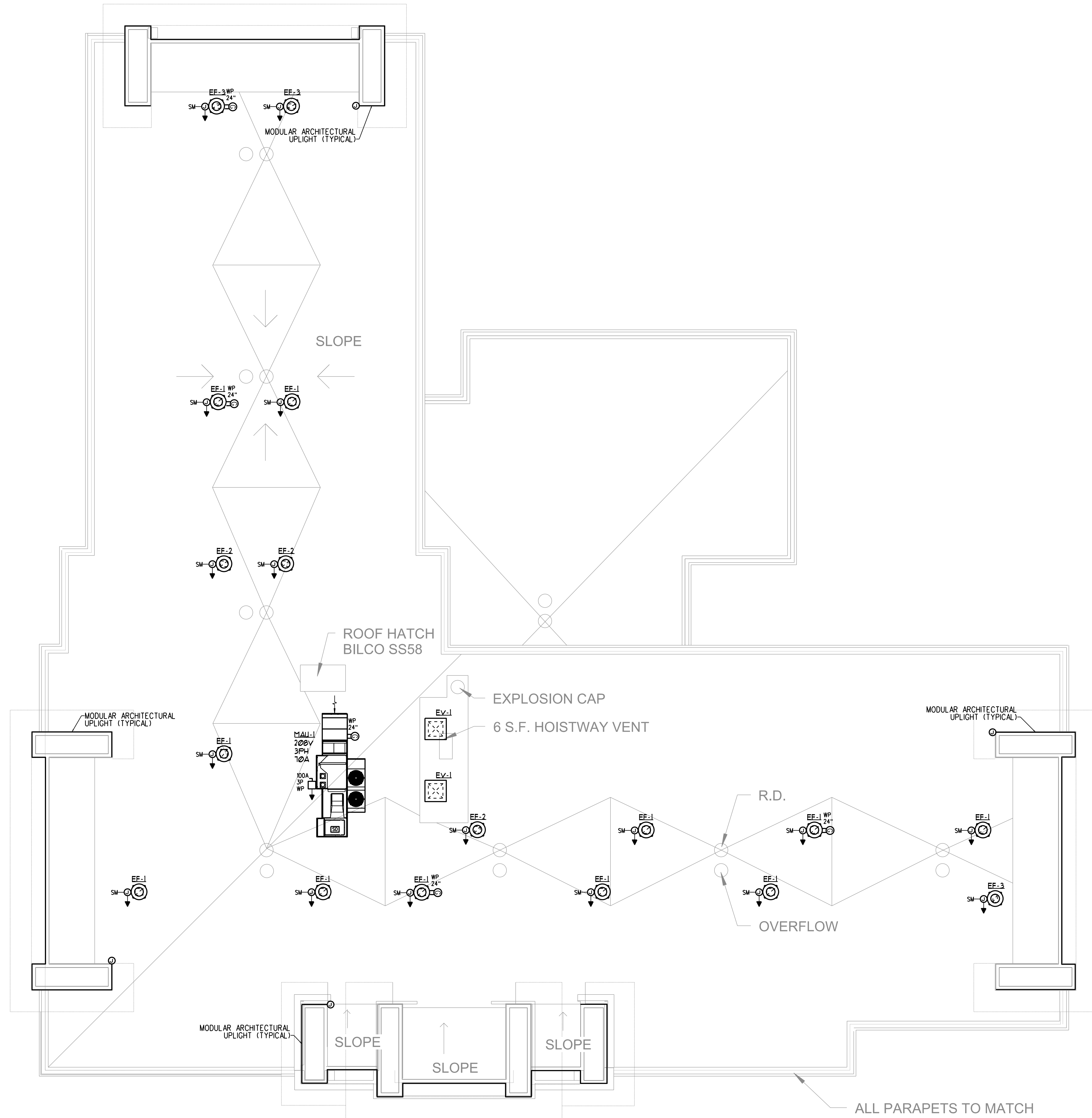
ROOF ELECTRICAL PLAN SCALE - 1/8" = 1'-0"
