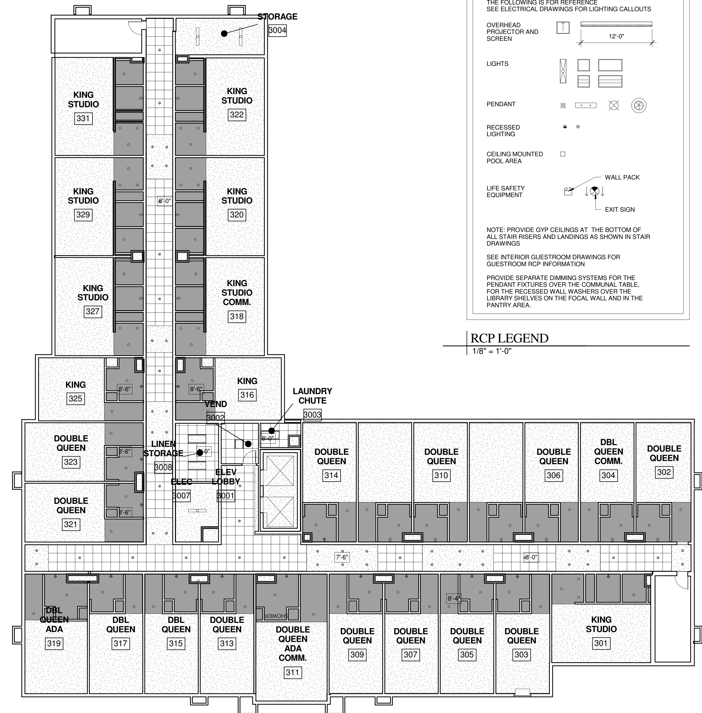
2 | THIRD & FOURTH FLOOR CEILING PLAN 3/32" = 1'-0"
