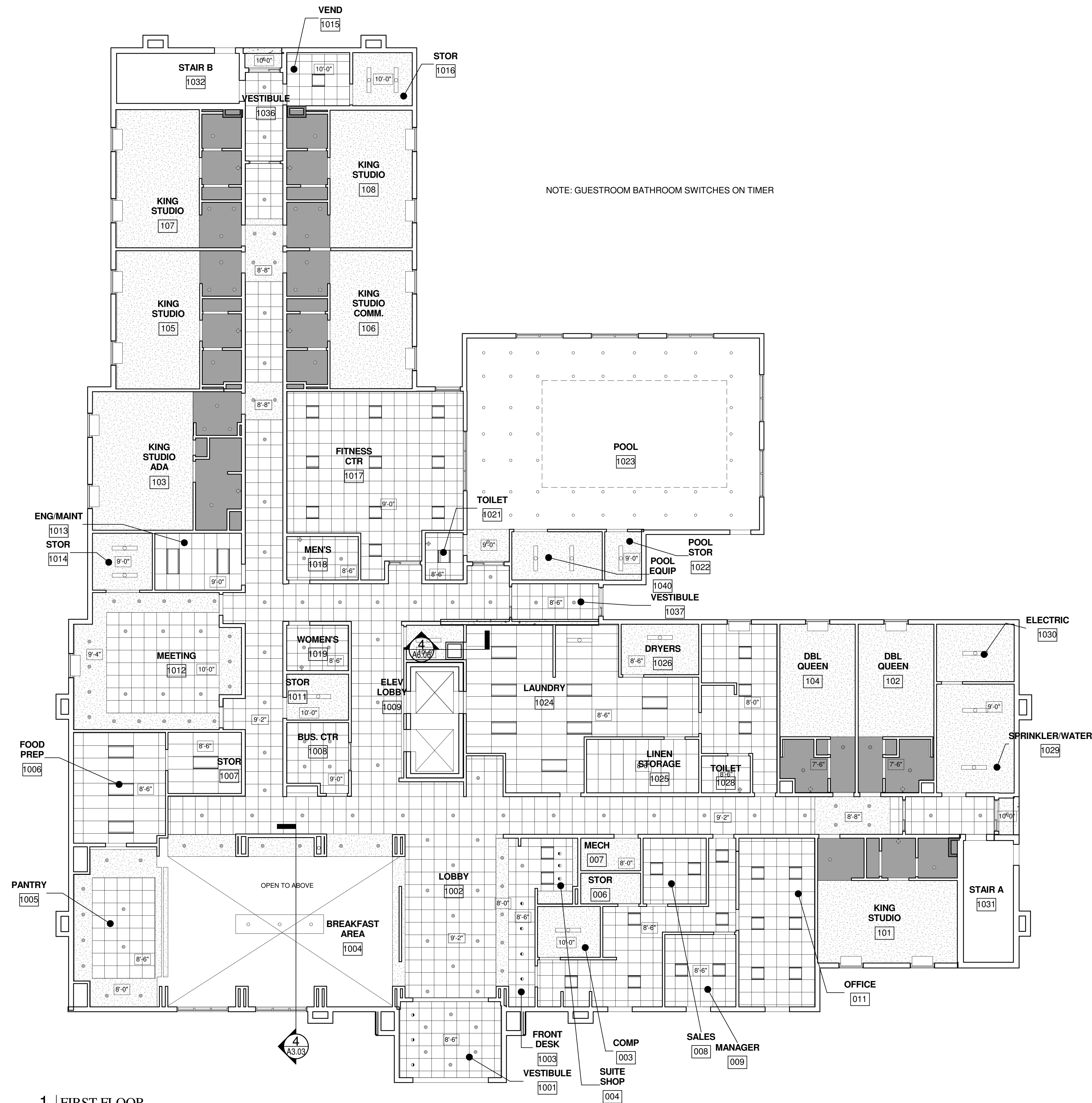
1 | FIRST FLOOR 1/8" = 1'-0"
