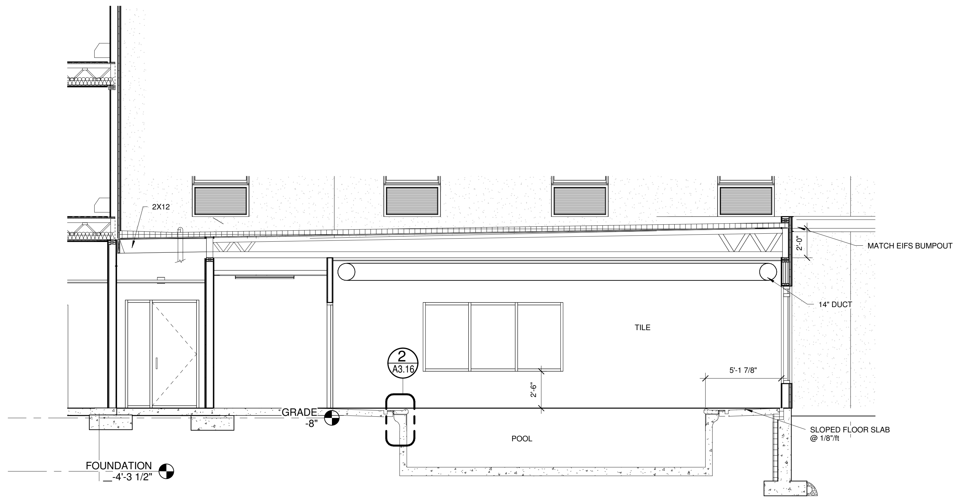
3 SECTION @ POOL 1/4" = 1'-0"
