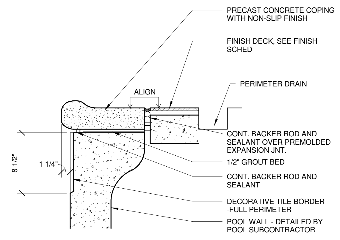
2 POOL COPING DETAIL 1 1/2" = 1'-0"
