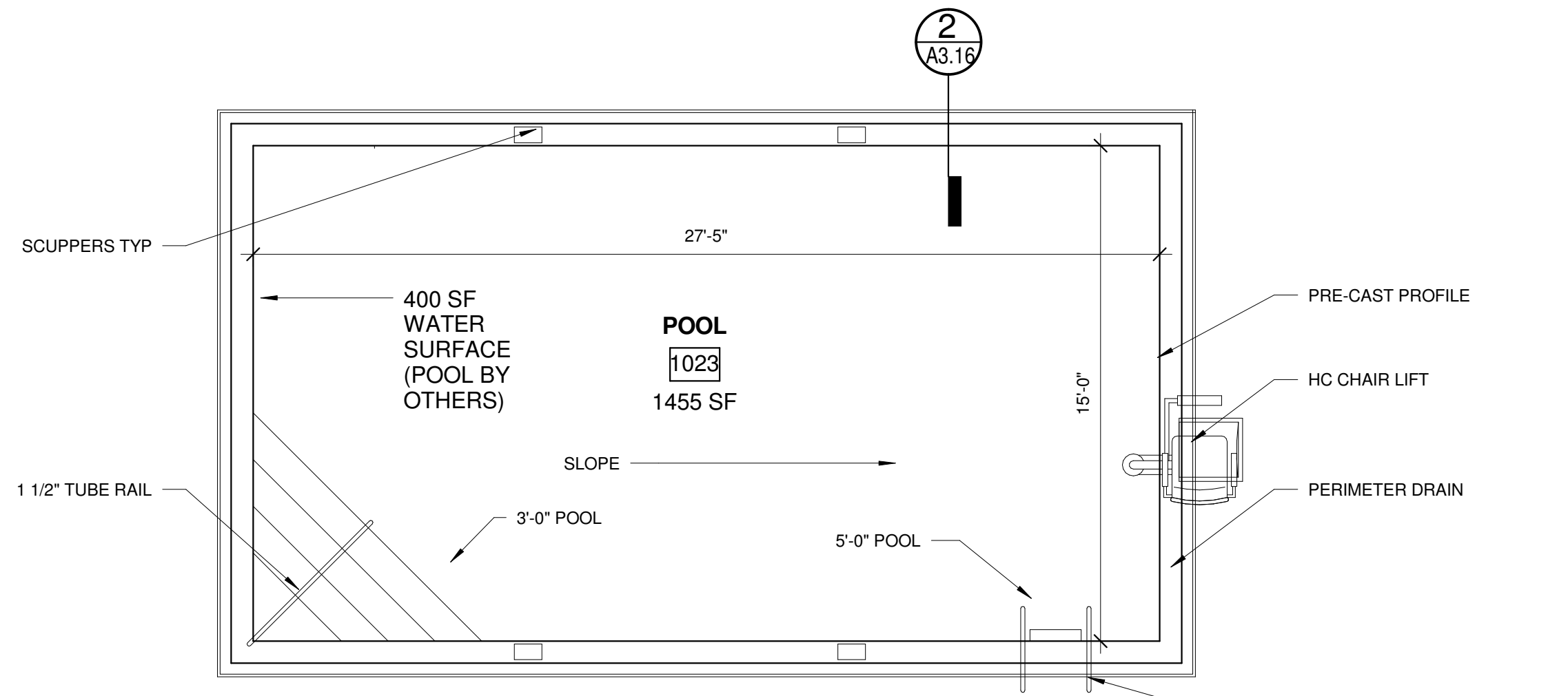
1 POOL PLAN 1/4" = 1'-0"
