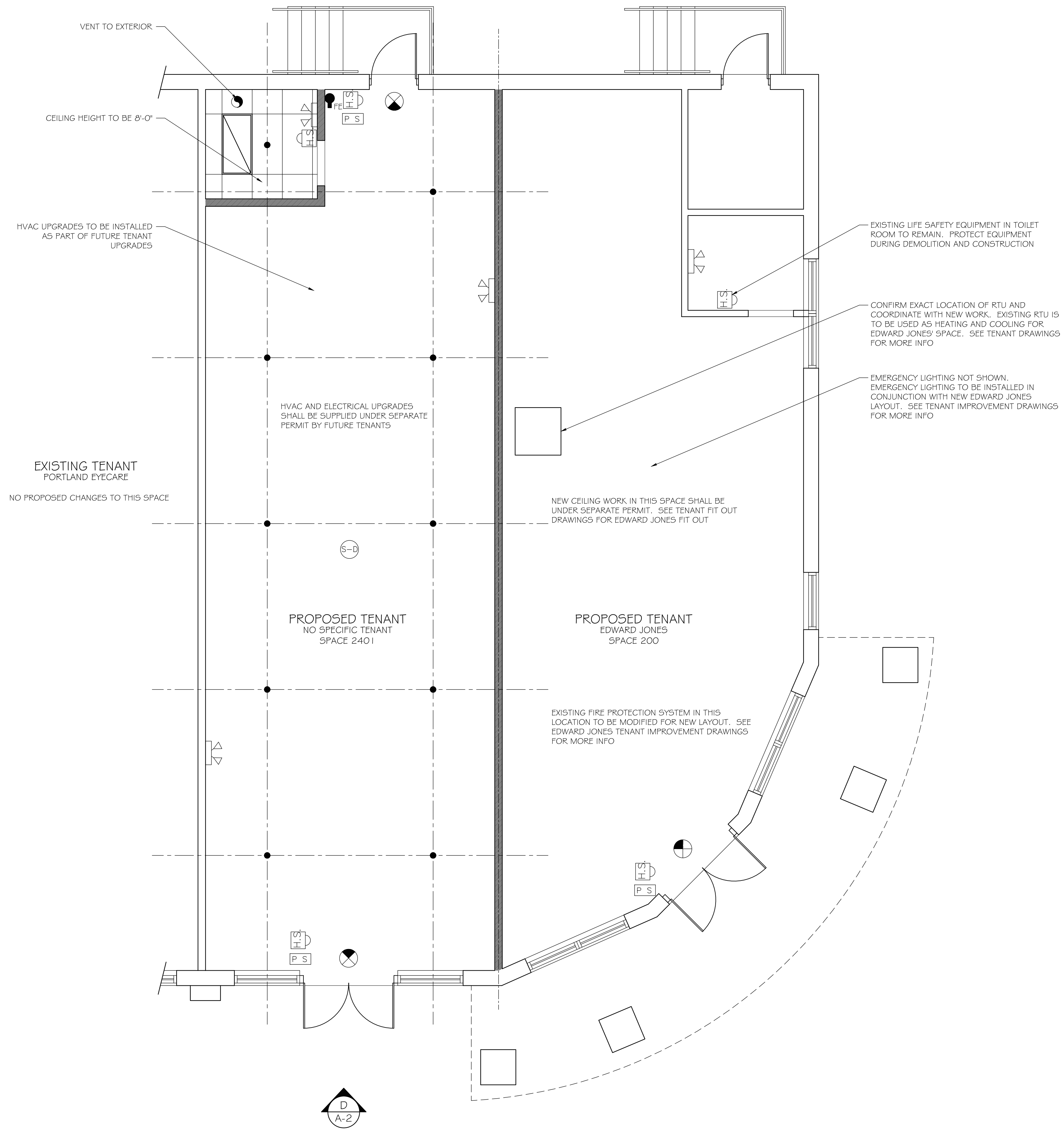
PROPOSED FLOOR PLAN SCALE: 1/4" = 1'-0"
