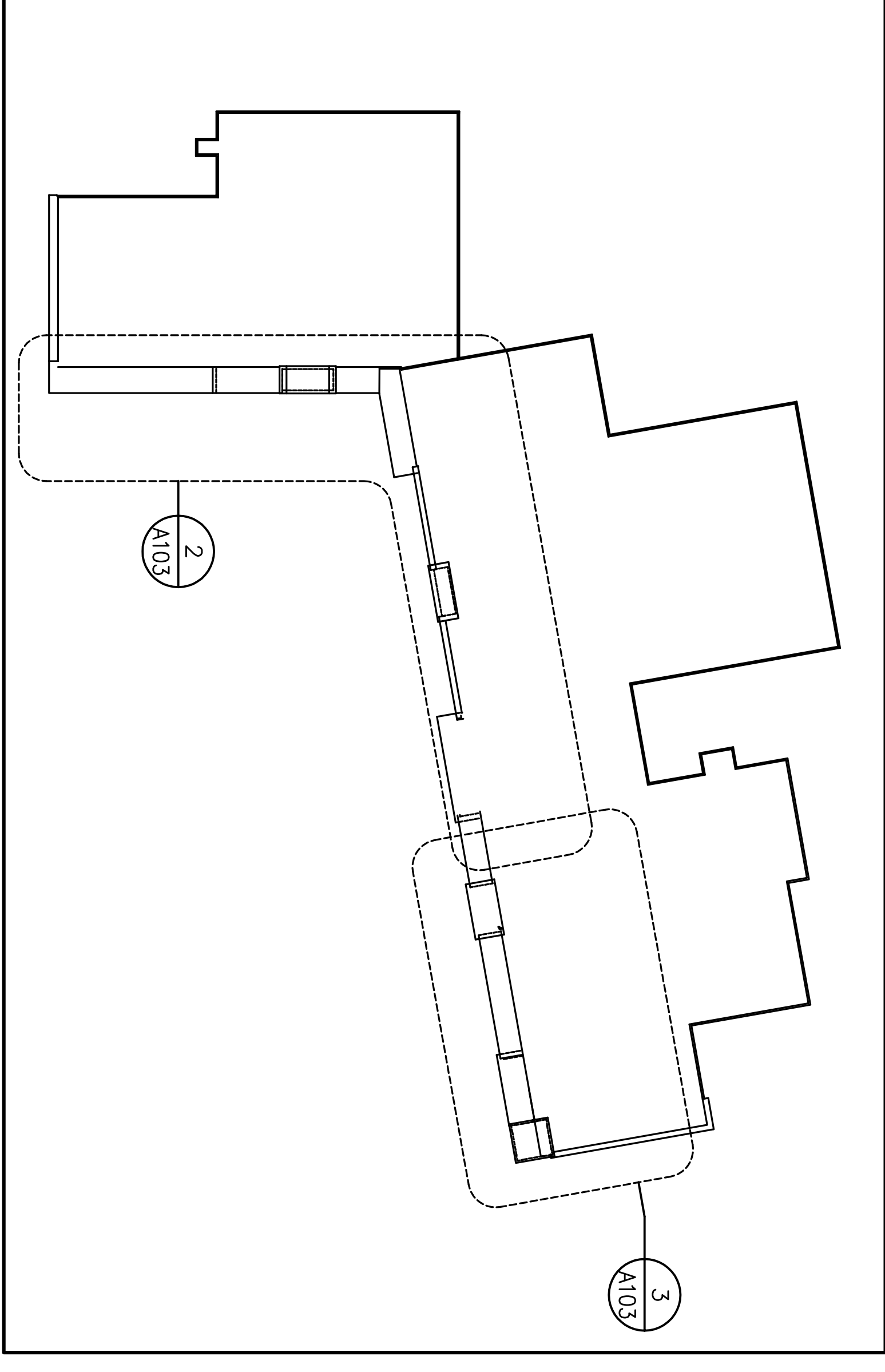
1 KEY ROOF PLAN SCALE: 1/8"=1'-0" A103
