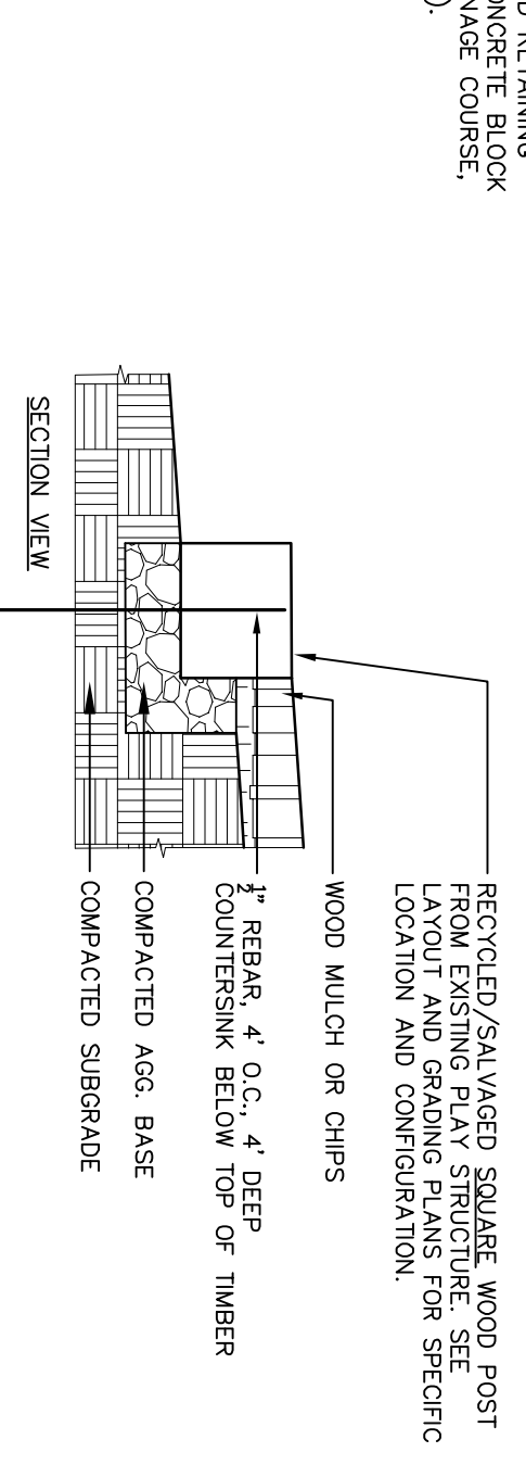
5 RECYCLED TIMBER TERRACE NOT TO SCALE
