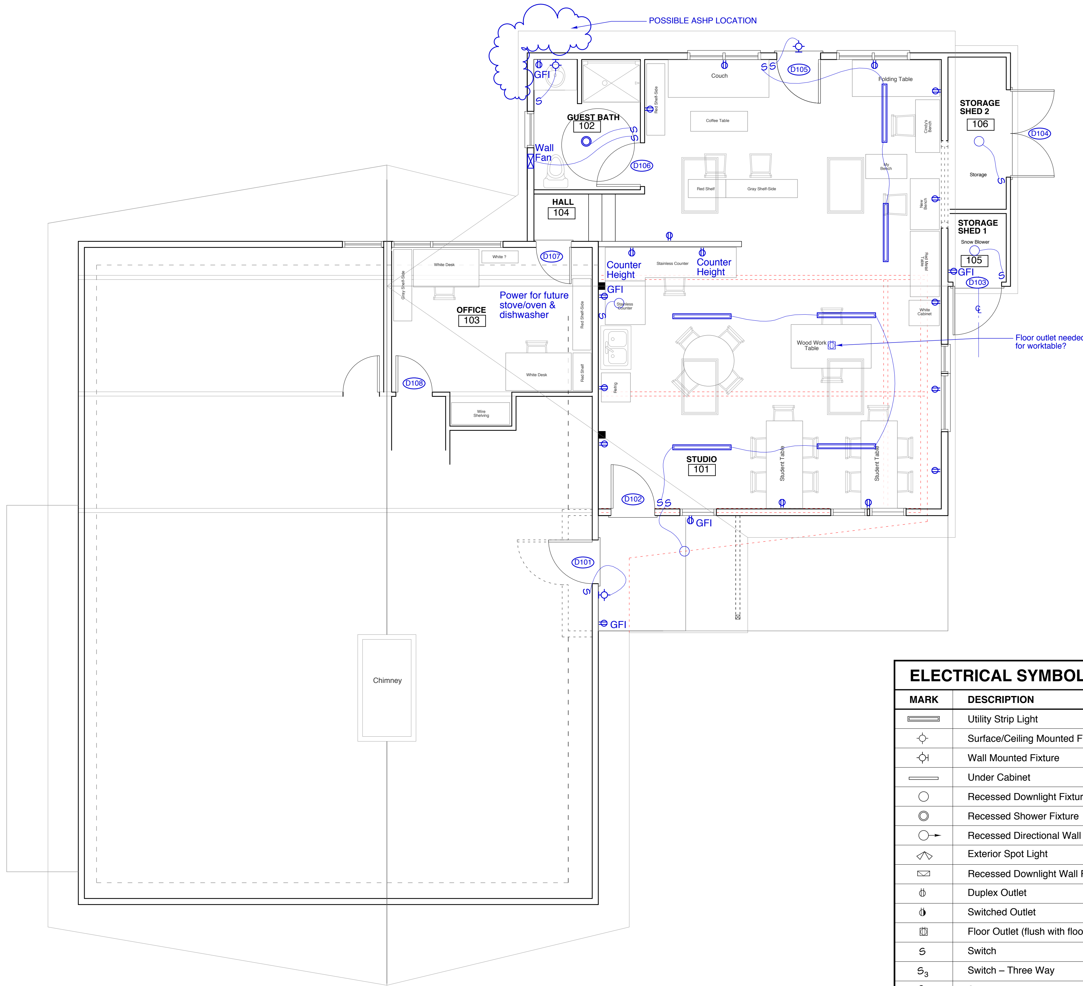
1 FIRST FLOOR ELECTRICAL PLAN SCALE: 1/4" = 1'-0"
