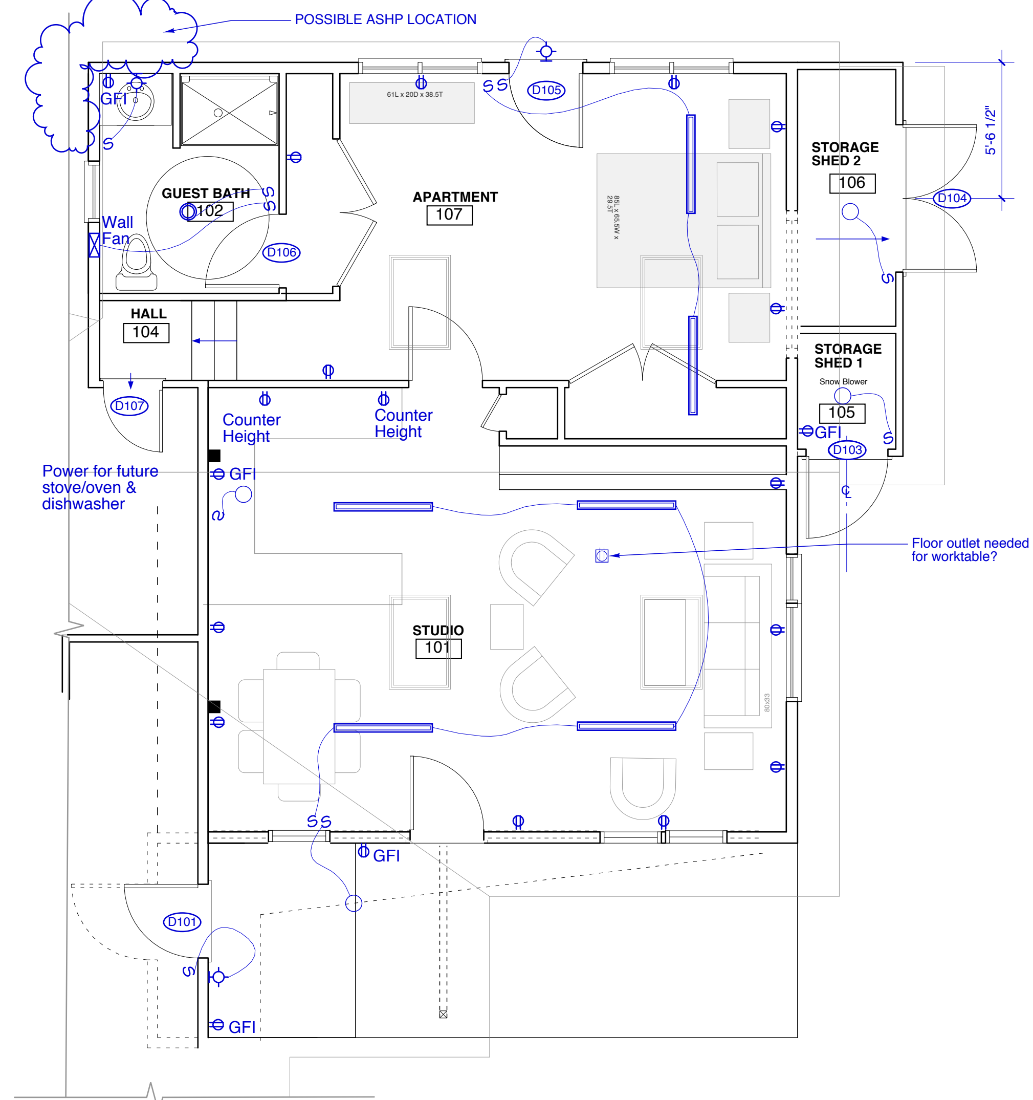
1 APT. FIRST FLOOR ELECTRICAL PLAN SCALE: 1/4" = 1'-0"
