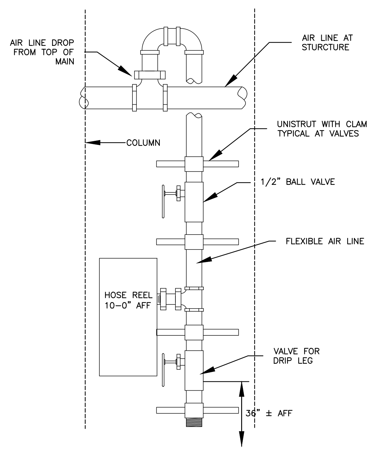
TYPICAL AIR DROP DETAIL NTS
