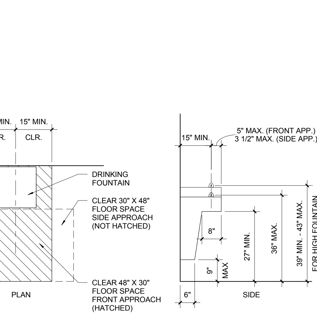
6 ACCESSIBLE DRINKING FOUNTAIN 1/2" = 1'-0"
