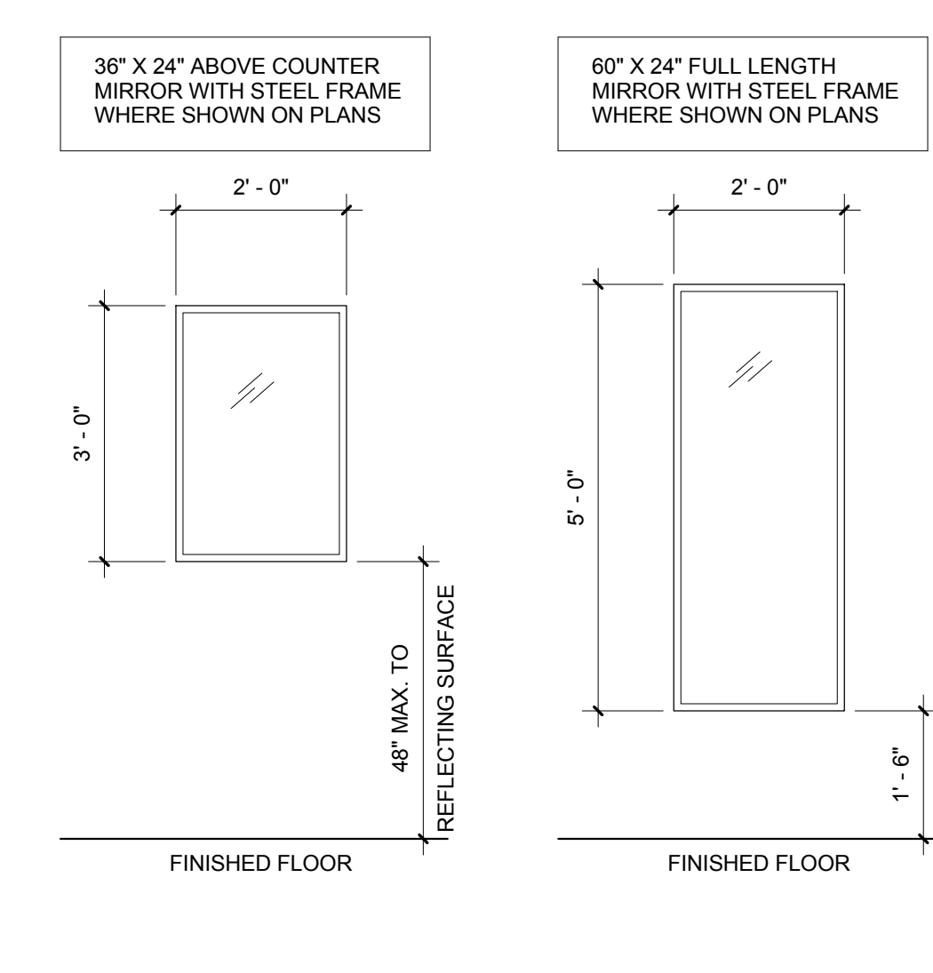
7 ACCESSIBLE MIRROR 1/2" = 1'-0"
