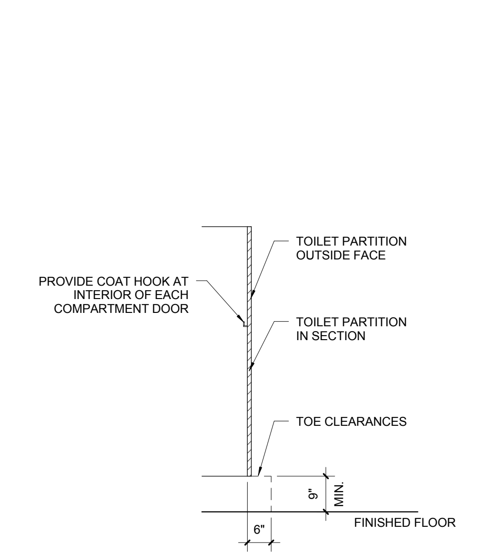
8 ACCESSIBLE PARTITION 1/2" = 1'-0"
