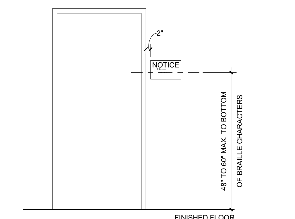
13 ACCESSIBLE SIGNAGE 1/2" = 1'-0"
