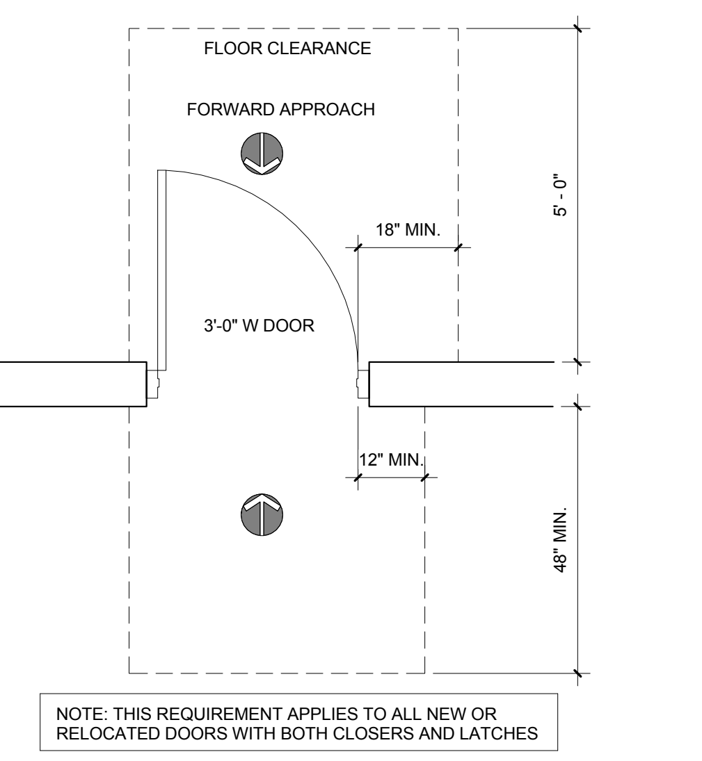
15 FLOOR CLEARANCE 1/2" = 1'-0"
