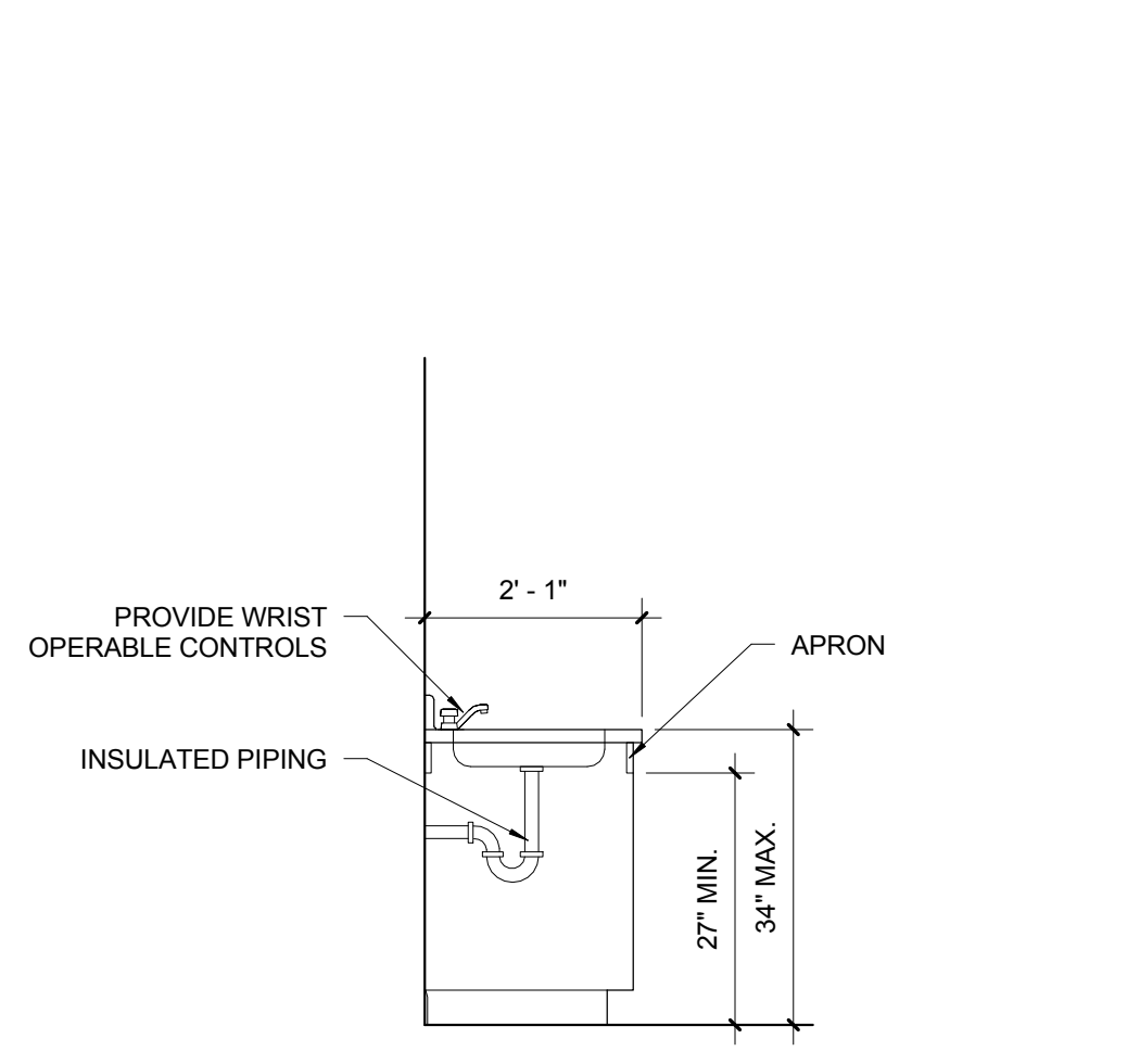
5 ACCESSIBLE SINK 1/2" = 1'-0"
