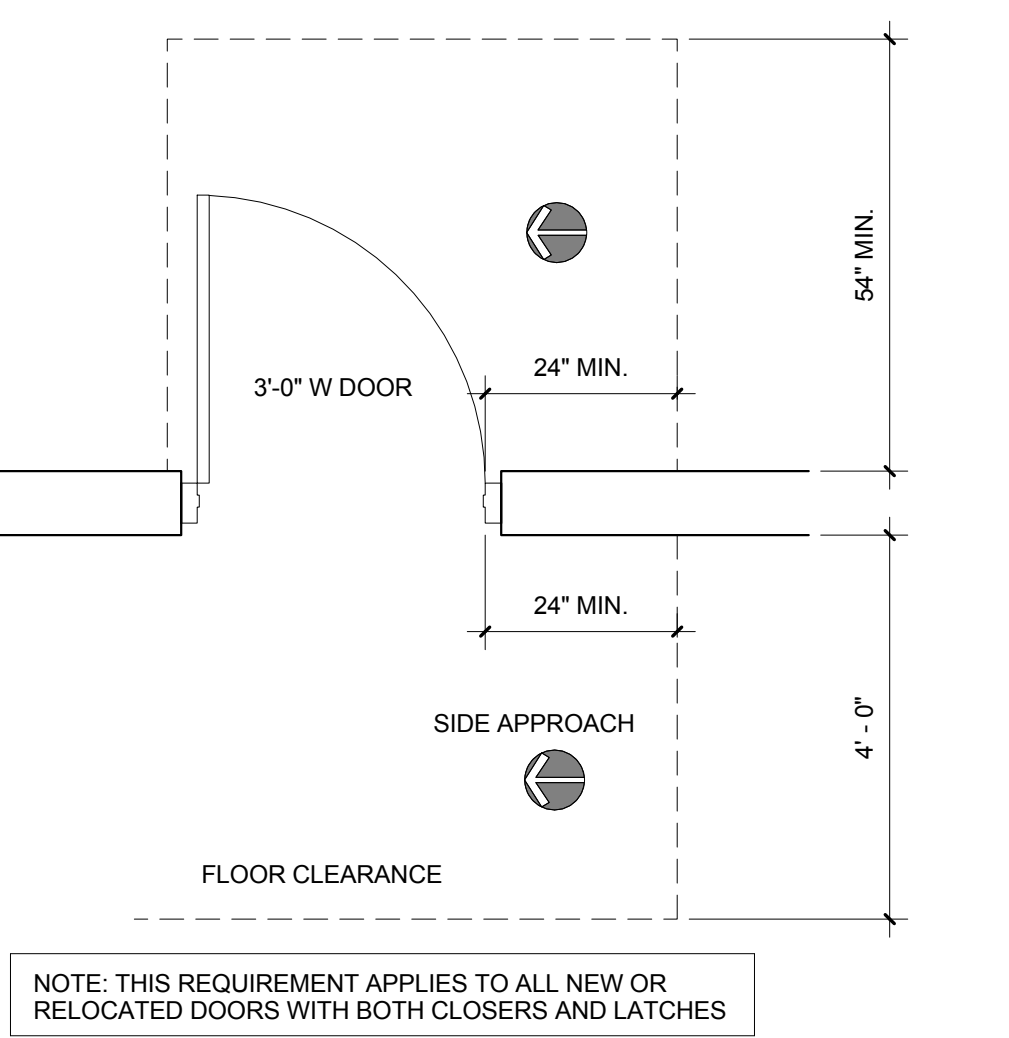
14 FLOOR CLEARANCE 1/2" = 1'-0"
