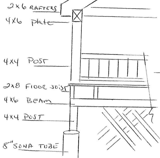
DETAIL SECTIONAL
