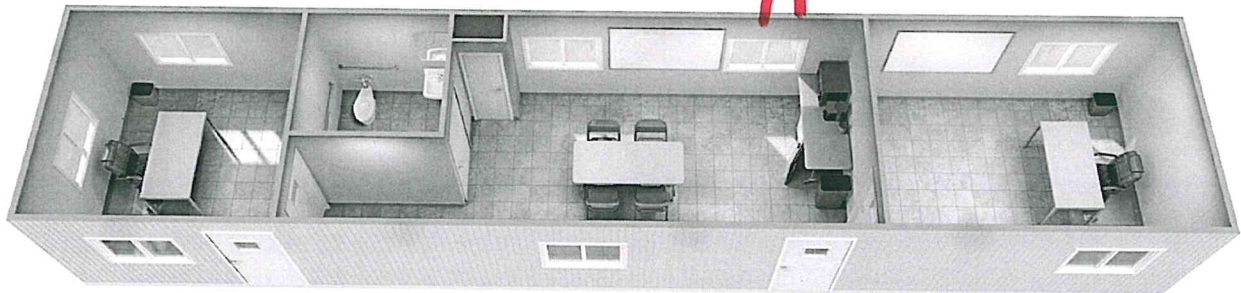
50 x 12 mobile office layout depicted. Includes 2 basic office packages and 1 basic conference room package.
