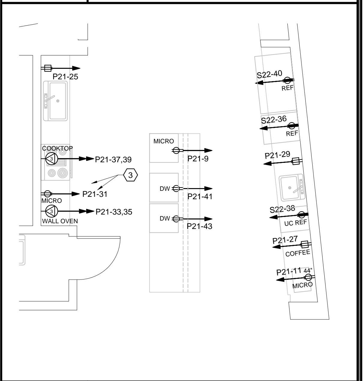
C9 ENLARGED KITCHEN PLAN 1/4"=1'-0"
