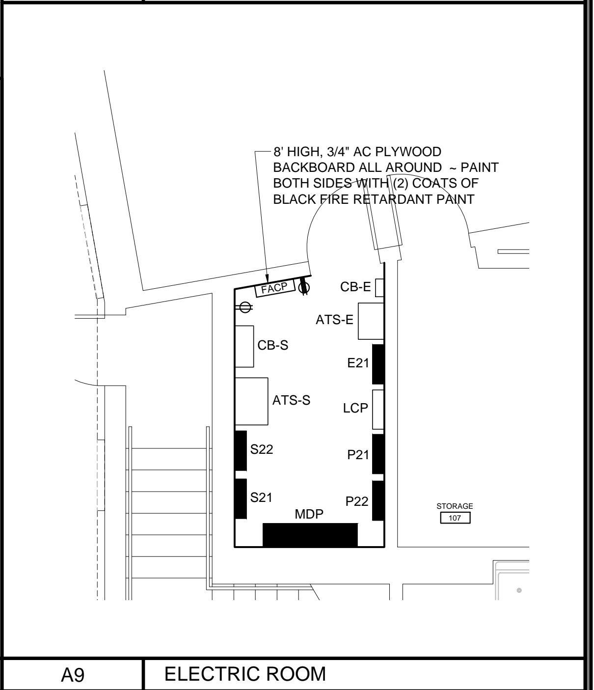
A9 ELECTRIC ROOM 1/4"=1'-0"
