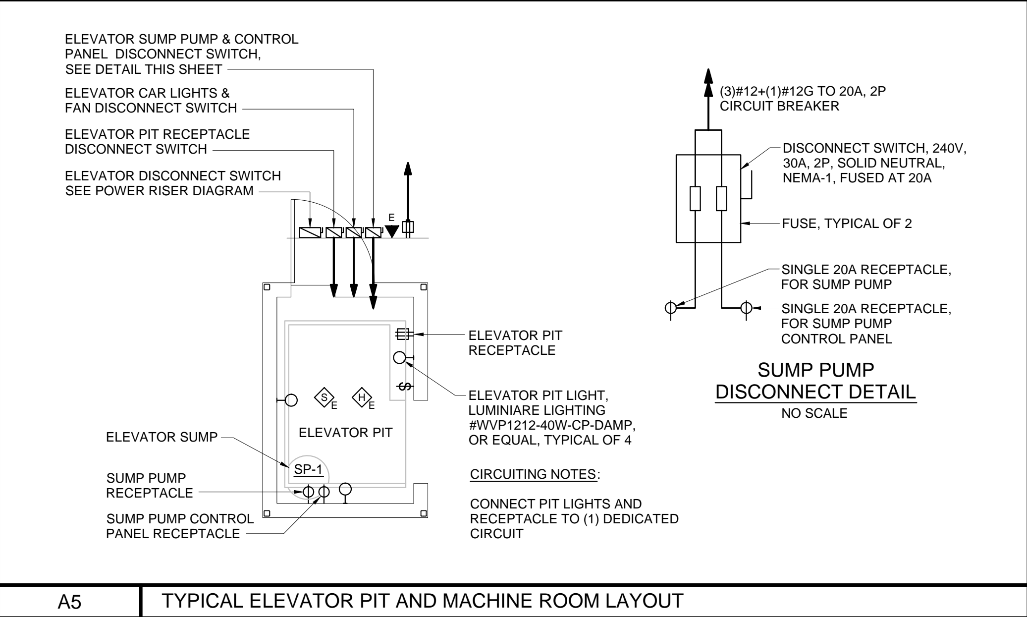
A5 TYPICAL ELEVATOR PIT AND MACHINE ROOM LAYOUT NO SCALE
