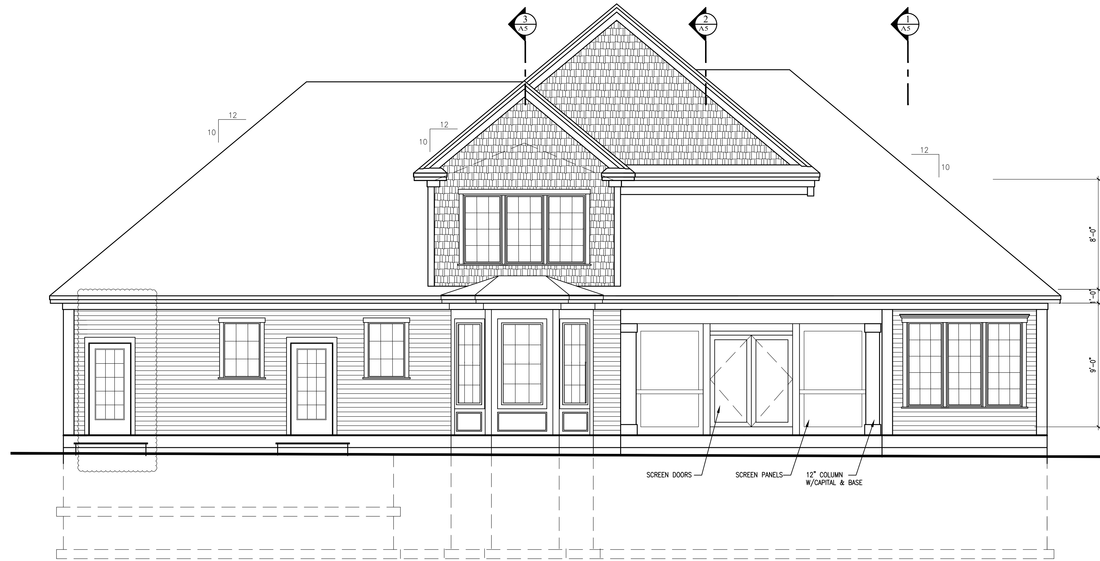
REAR ELEVATION
