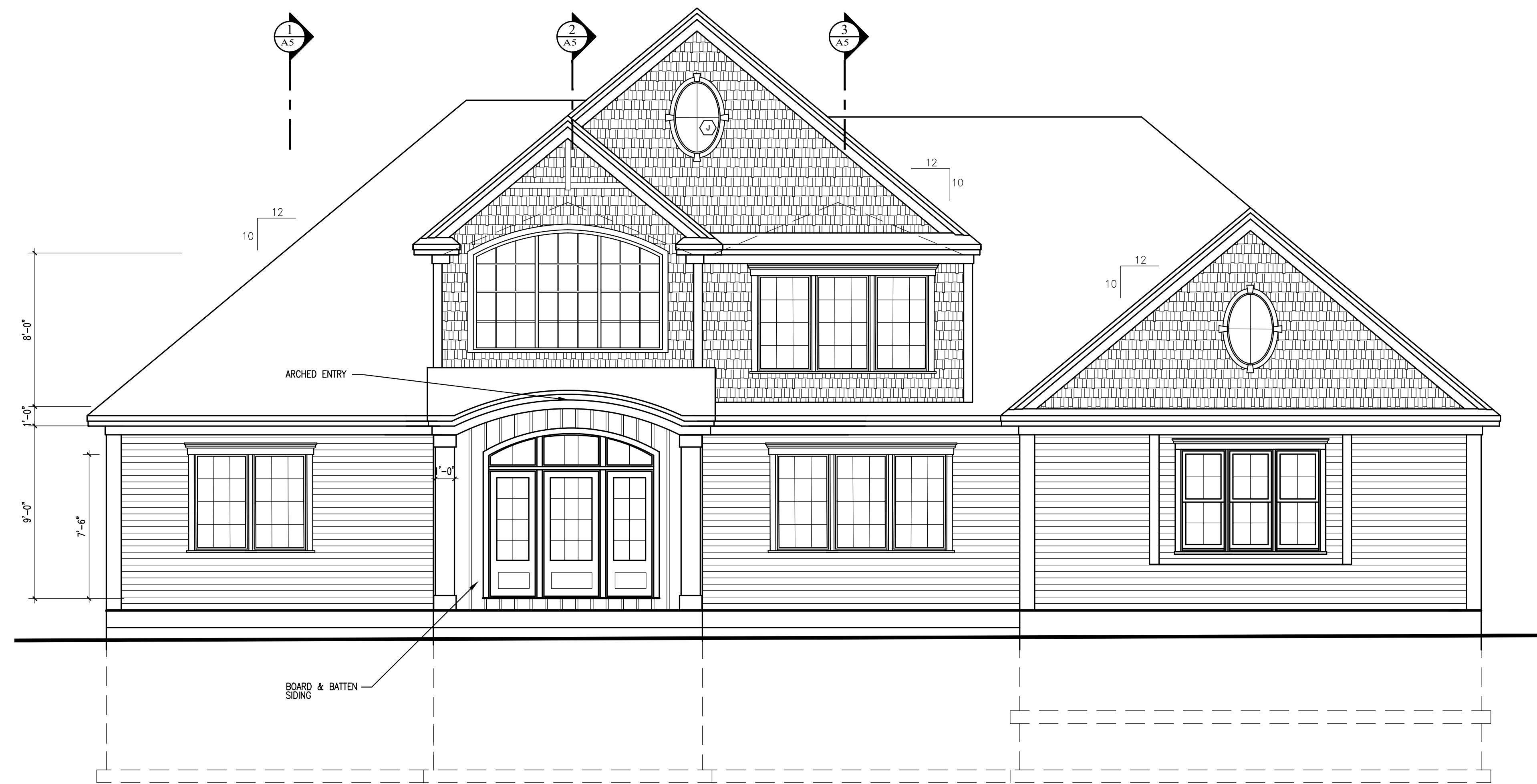
FRONT ELEVATION
