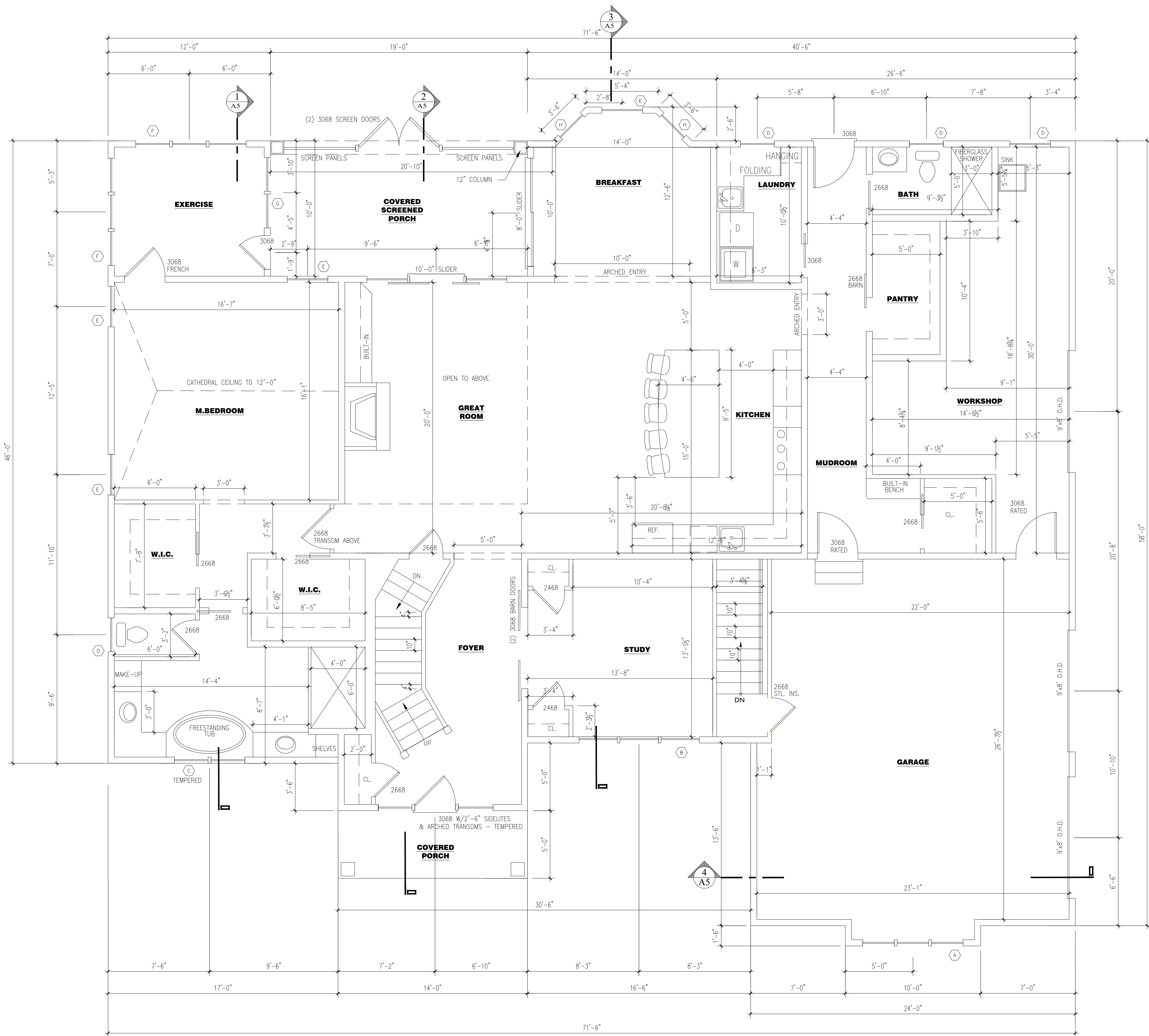
FIRST FLOOR PLAN FIRST FLOOR: 2,530 S.F. 1/4" = 1'-0" GARAGE: 660 S.F. WORK SHOP: 284 S.F. COVERED PORCH: 240 S.F.
