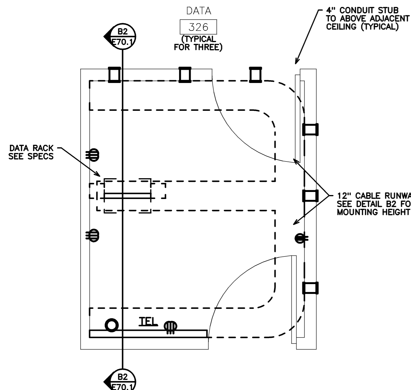
DATA ROOM ENLARGED PLAN
