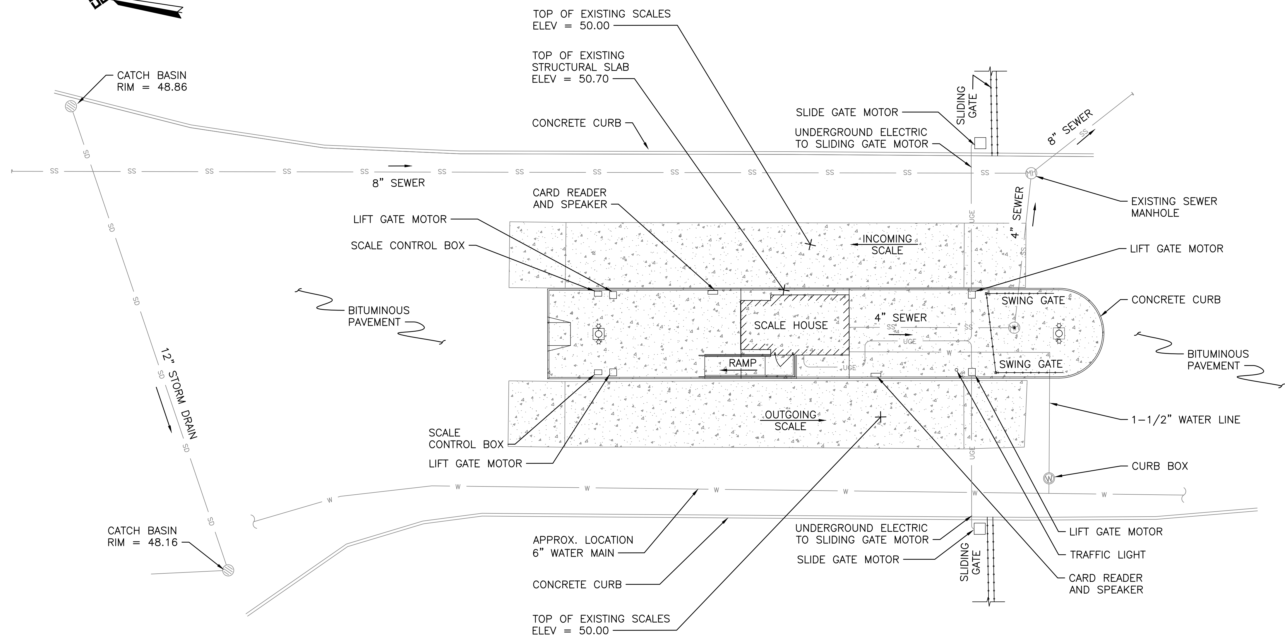
EXISTING CONDITIONS PLAN SCALE: 1" = 10'-0"
