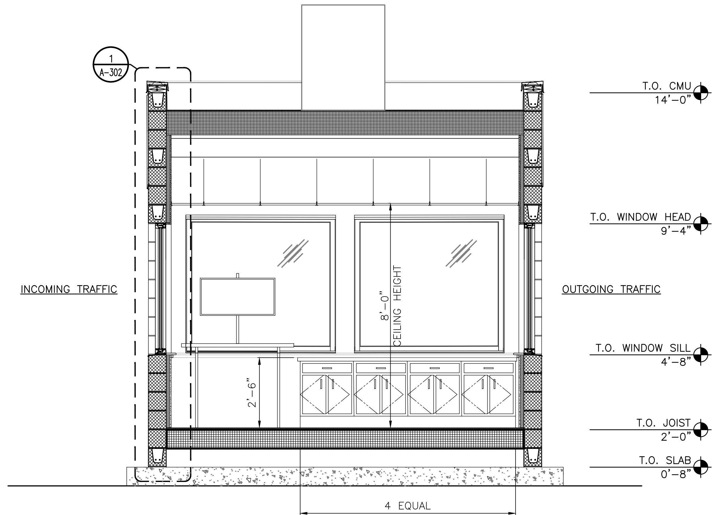
1 NORTH BUILDING SECTION A-301 SCALE: 1/2" = 1'-0" A-101
