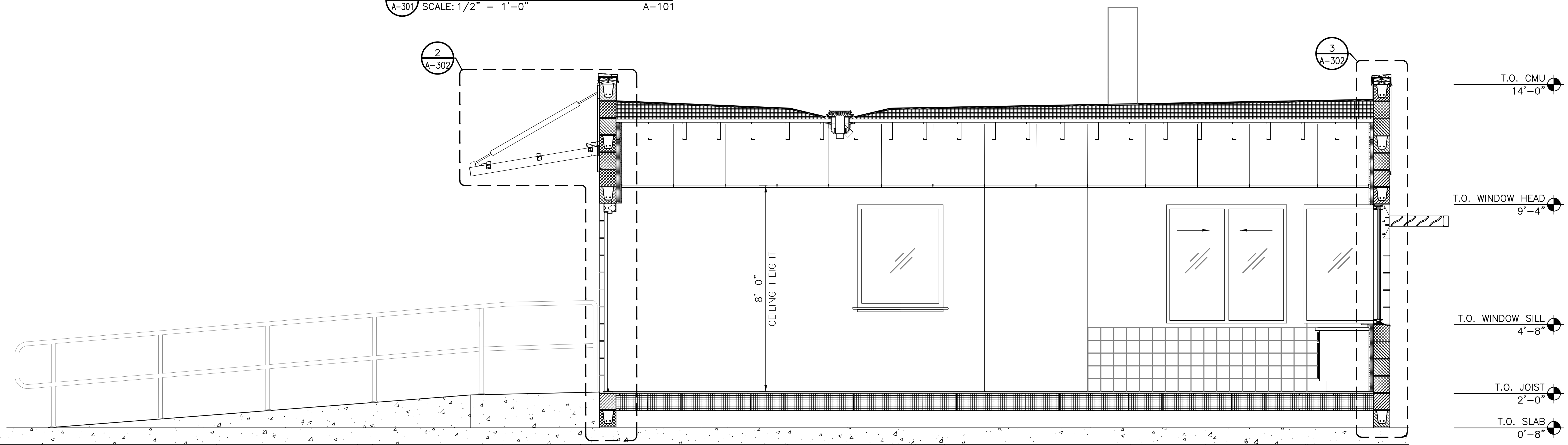
2 WEST BUILDING SECTION A-301 SCALE: 1/2" = 1'-0" A-101
