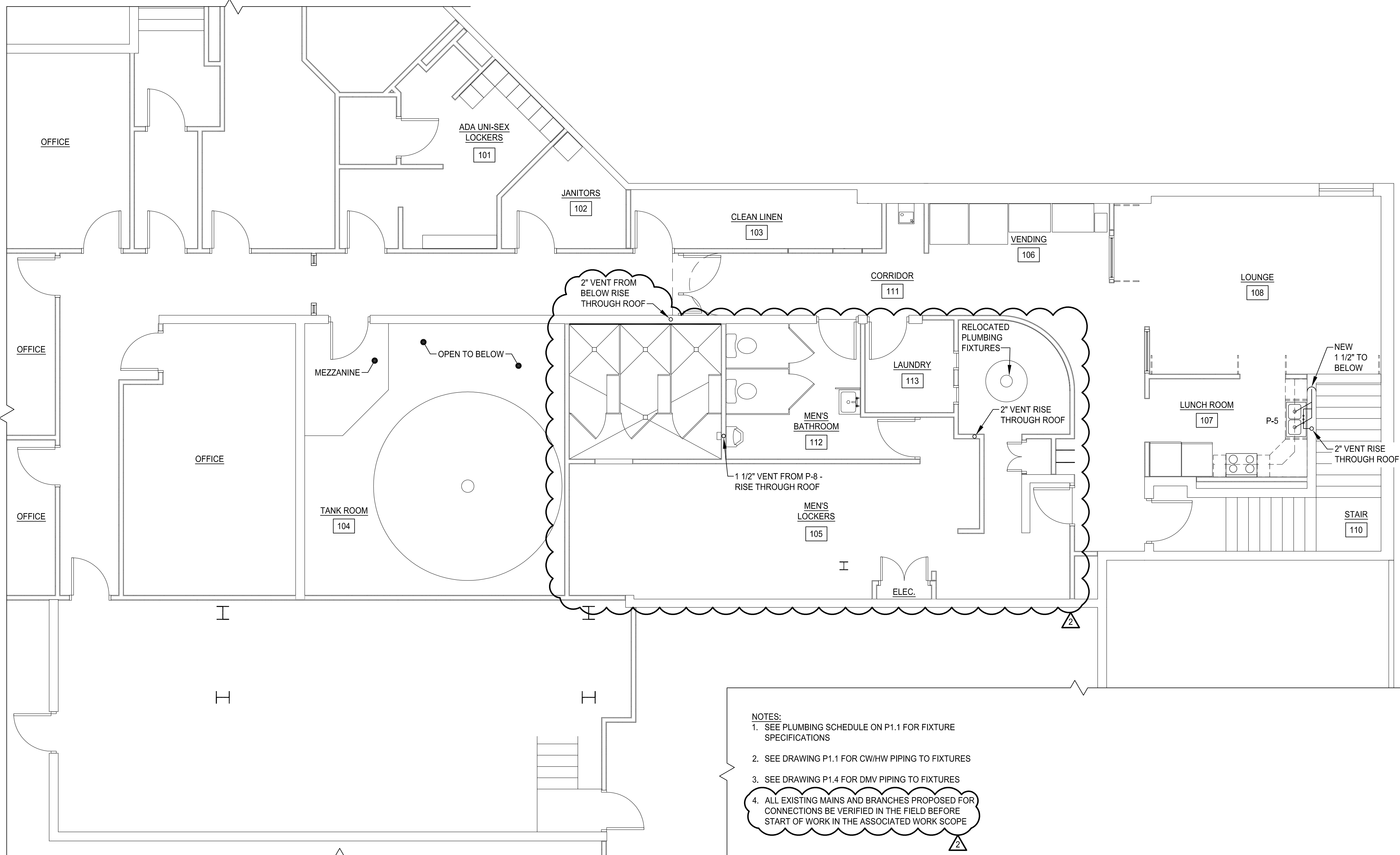
LEVEL 2 FLOOR SANITARY + VENT PLAN 1 22X34 SCALE: 1/4"=1'-0" 11X17 SCALE: 1/8"=1'-0" P1.5
