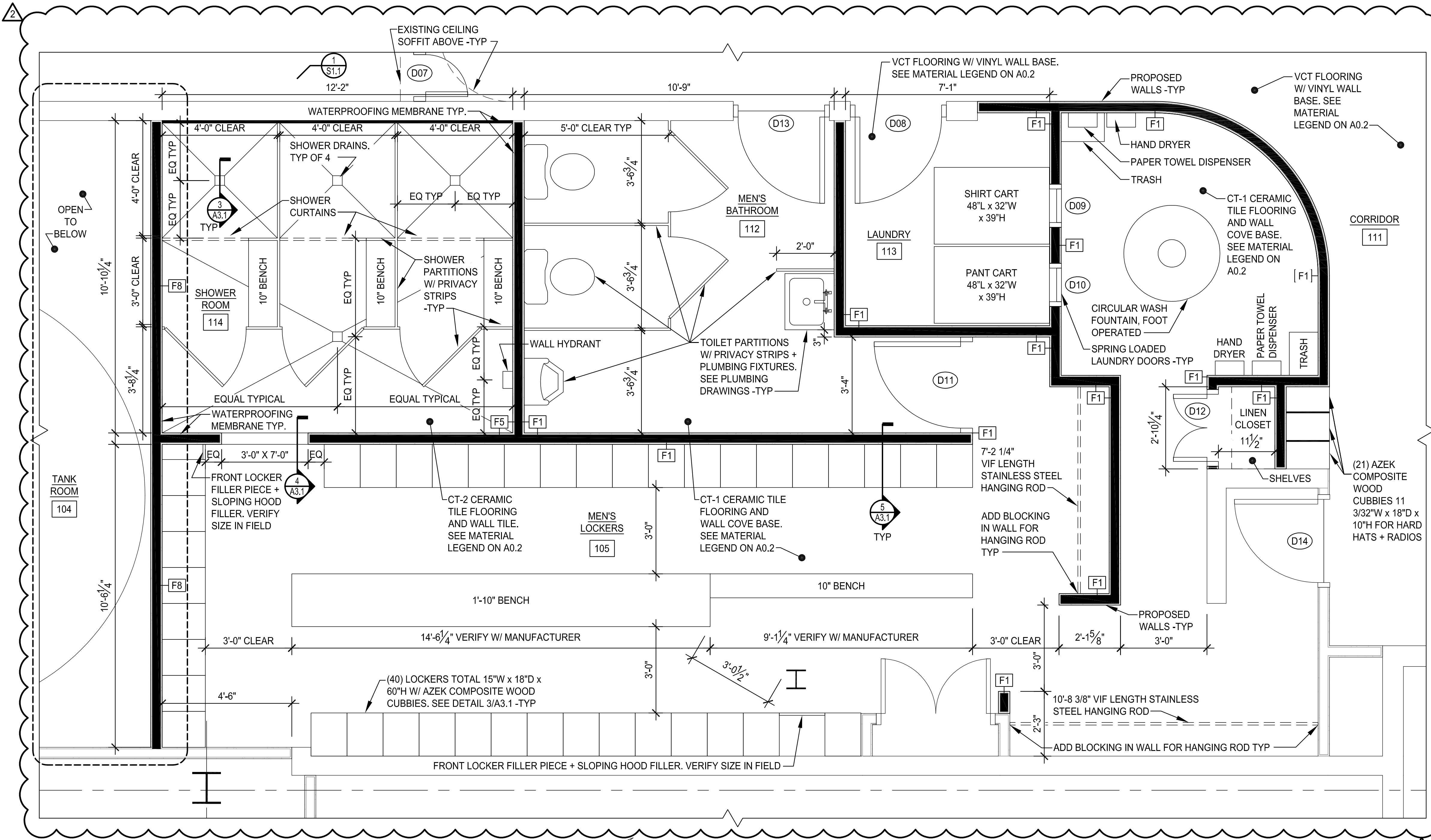
ENLARGED MEN'S LOCKER RM. PLAN 1 22X34 SCALE: 1/2"=1'-0" 11X17 SCALE: 1/4"=1'-0" A1.4
