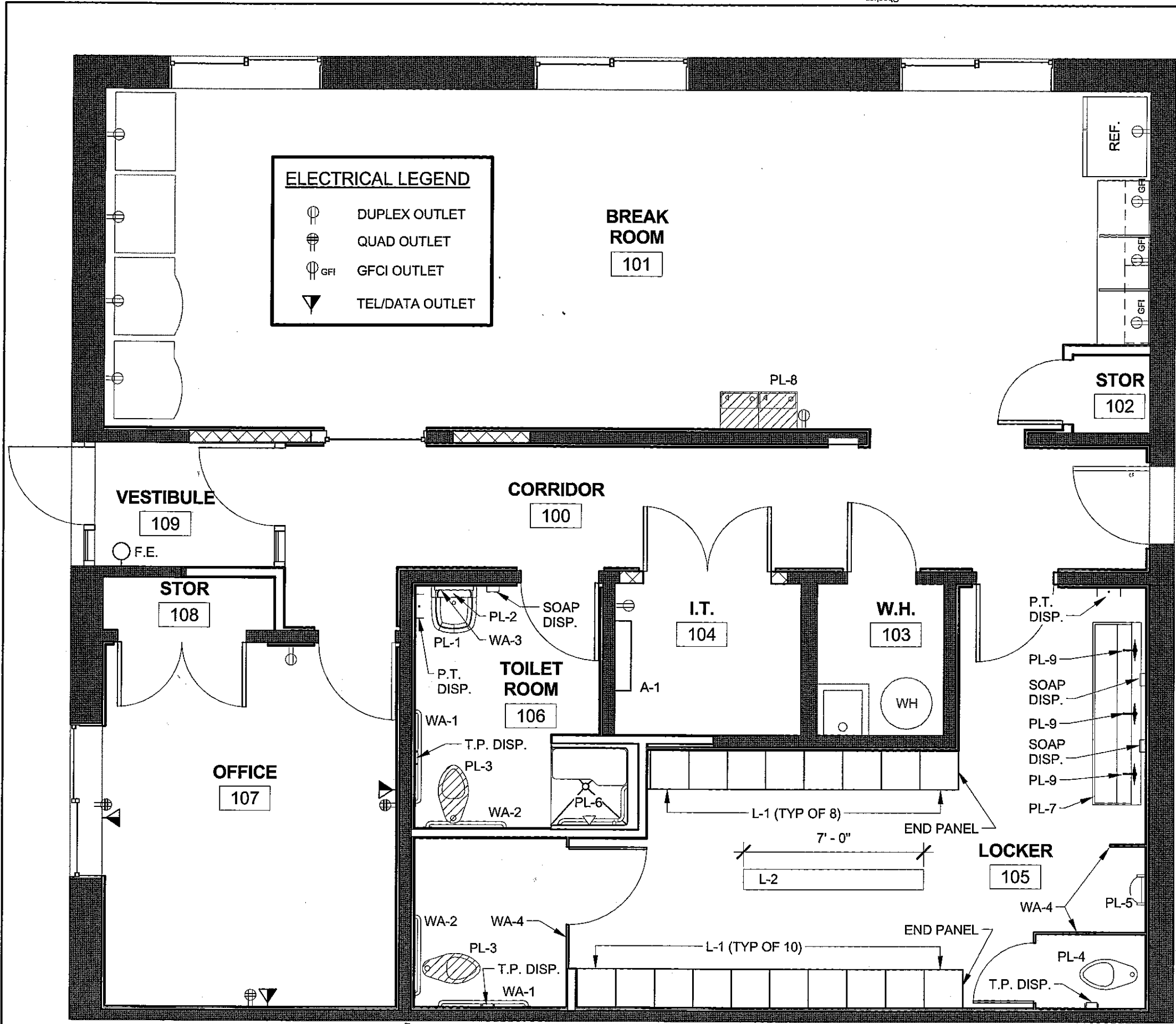
1 EQUIPMENT PLAN 1/4" = 1'-0"
