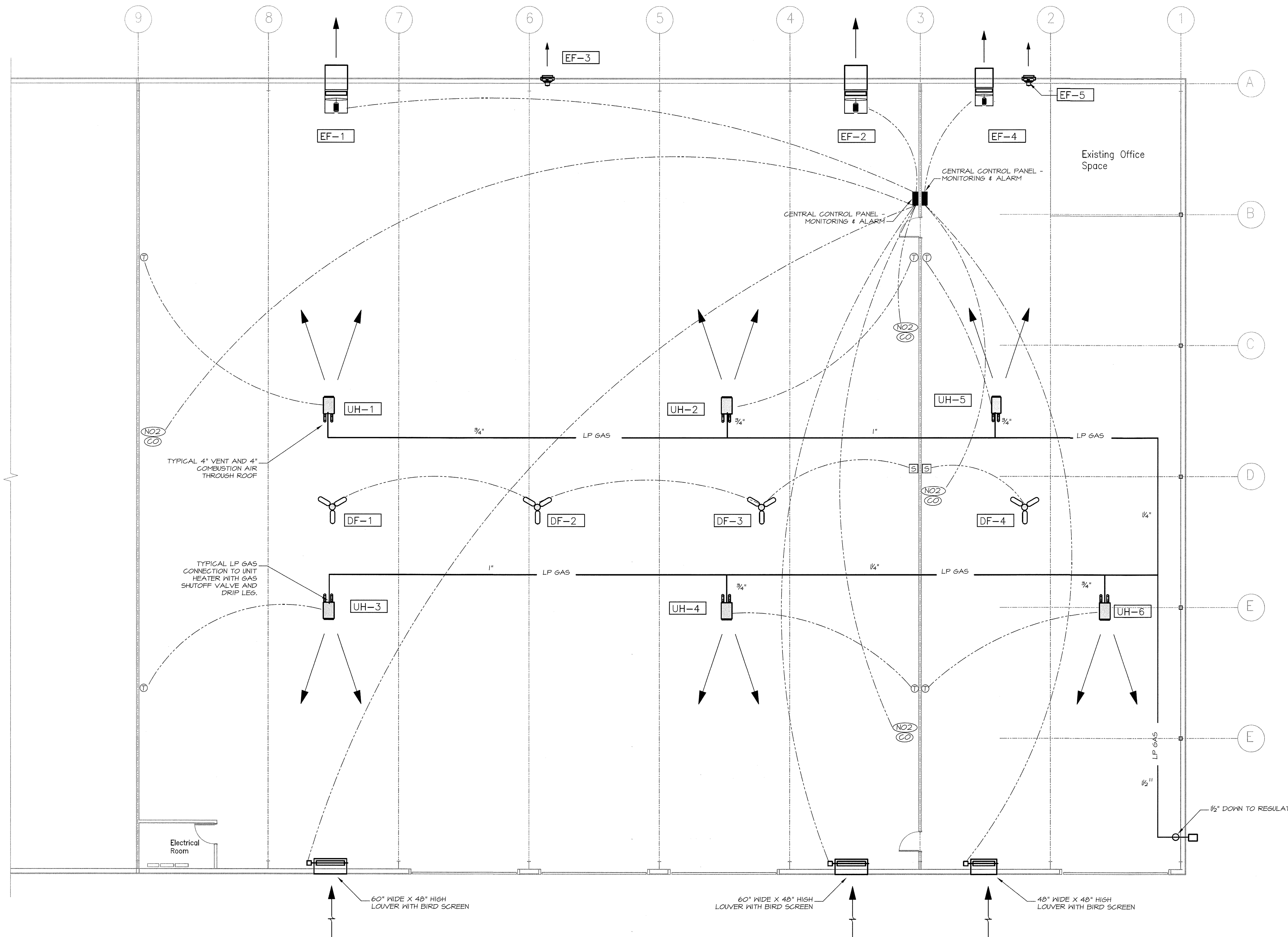
MECHANICAL HEATING & VENTILATION PLAN SCALE: 1/8" = 1'-0"
