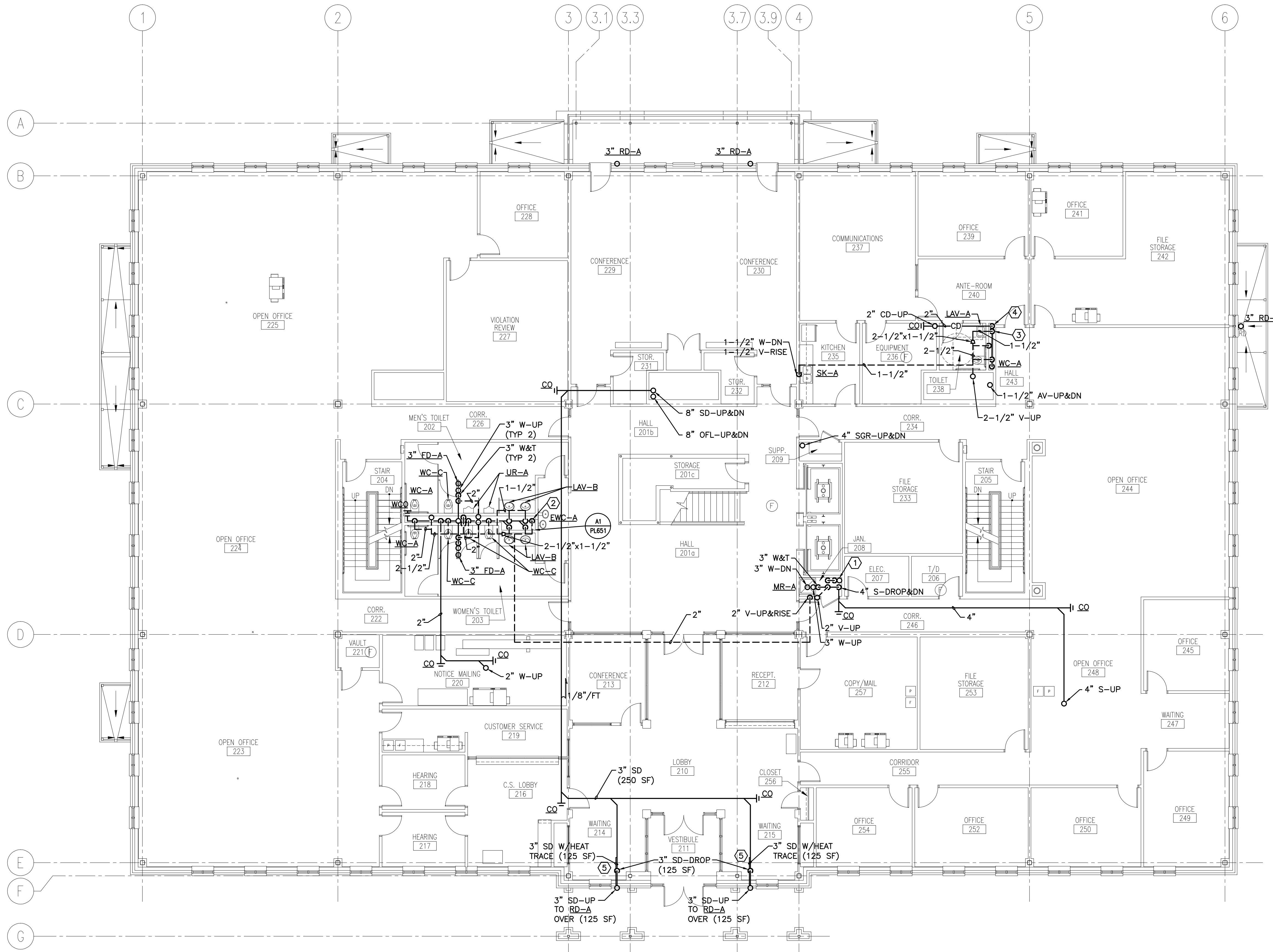
A1 SECOND FLOOR PLAN
