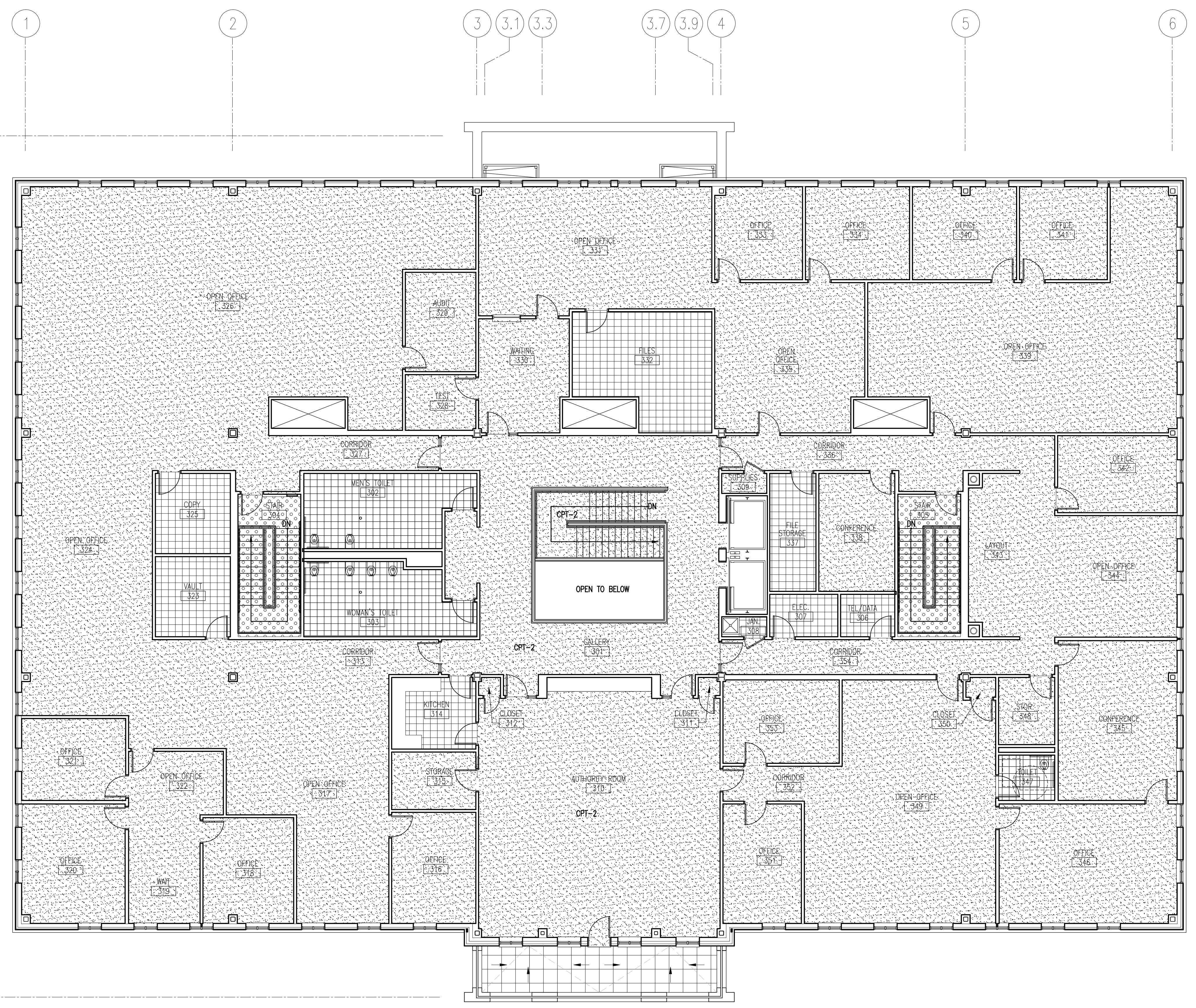
A1 THIRD FLOOR FINISH PLAN
