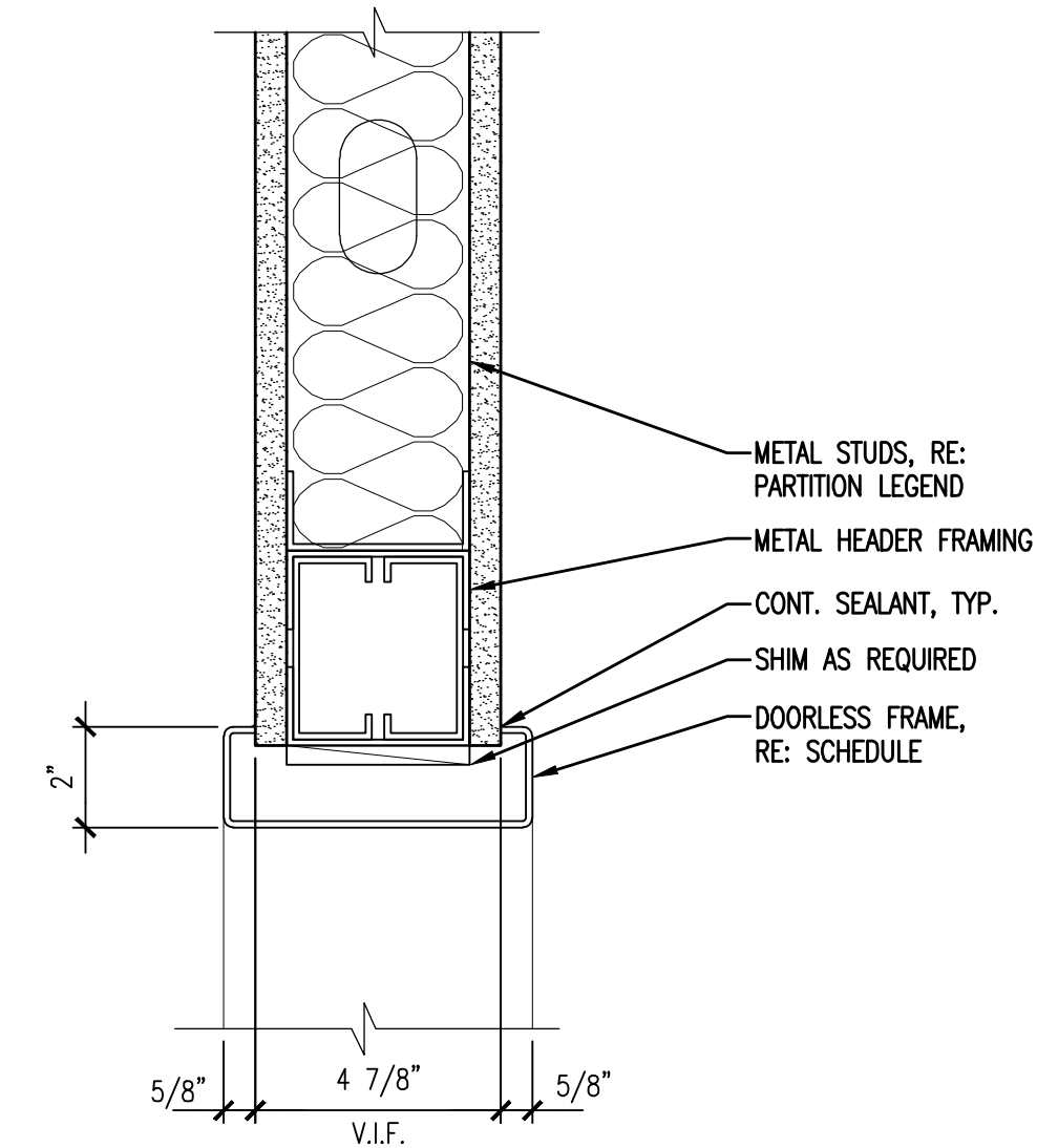
J4 HEAD DETAIL
