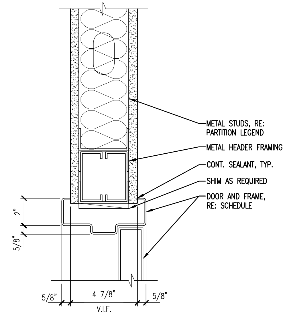
J1 HEAD DETAIL
