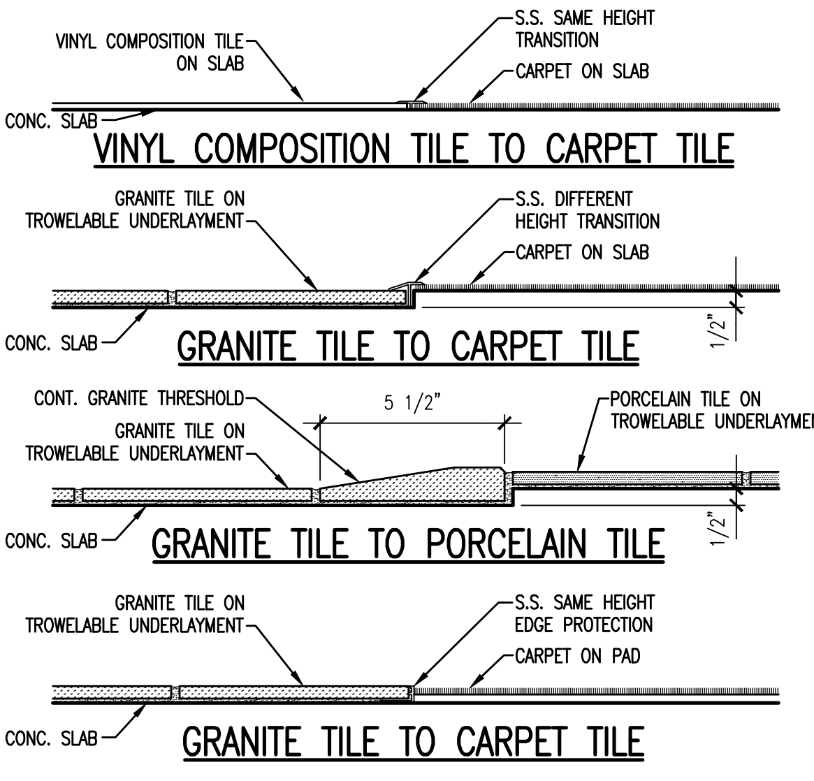
A1 FLOOR MATERIAL TRANSITIONS
