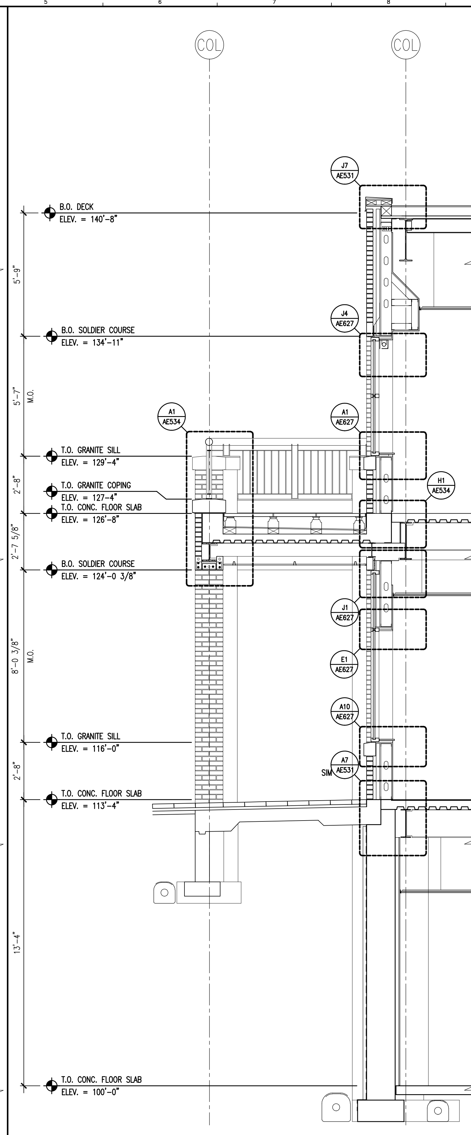
A1 WALL SECTION A5 WALL SECTION A9 WALL SECTION 3/8" = 1'-0" - 3/8" = 1'-0" - 3/8" = 1'-0" -
