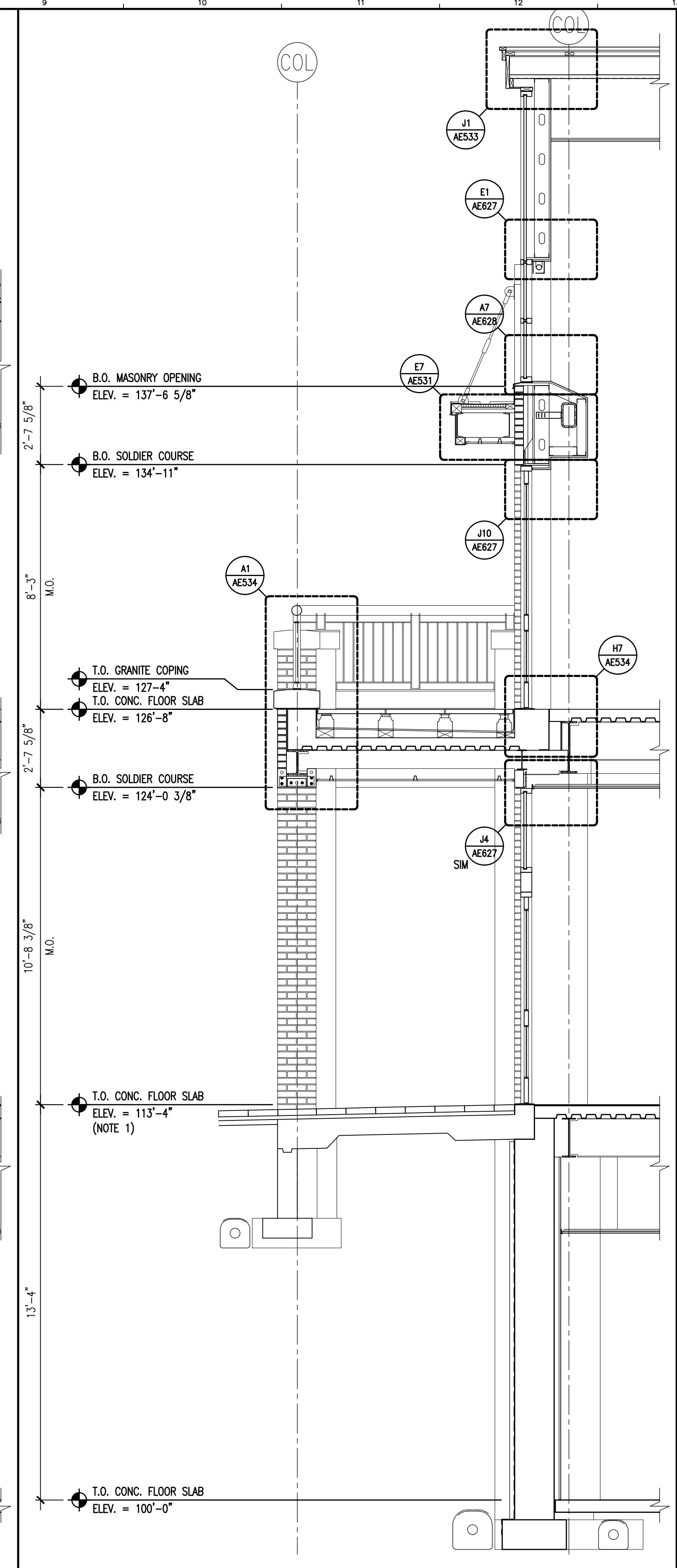
A1 WALL SECTION A5 WALL SECTION A9 WALL SECTION 3/8" = 1'-0" - 3/8" = 1'-0" - 3/8" = 1'-0" -
