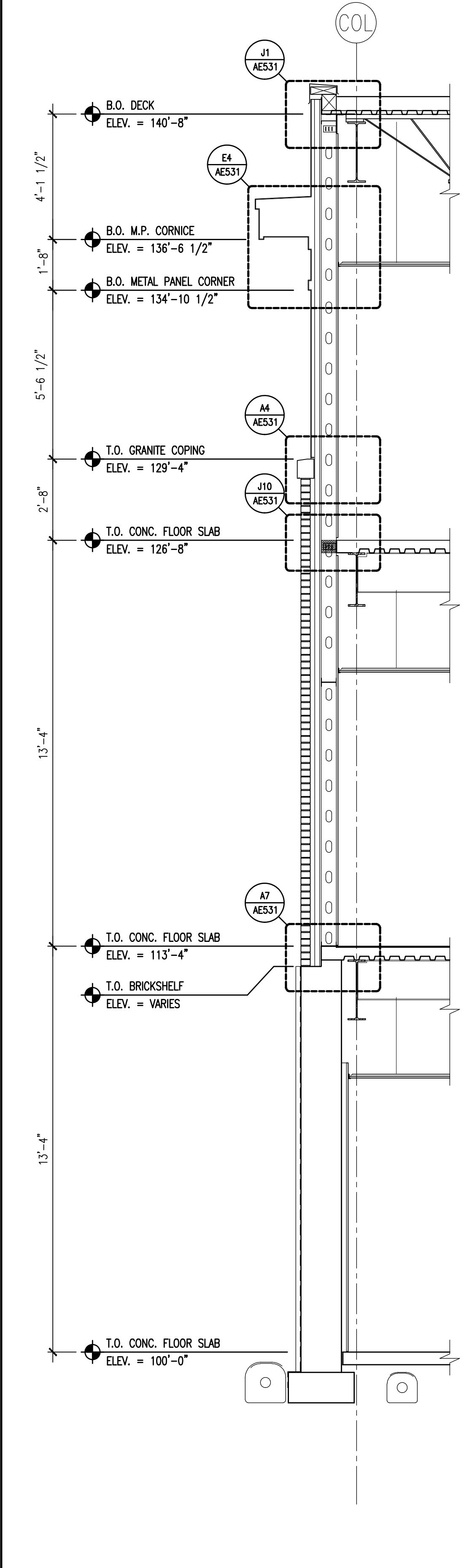
A7 WALL SECTION 3/8" = 1'-0"
