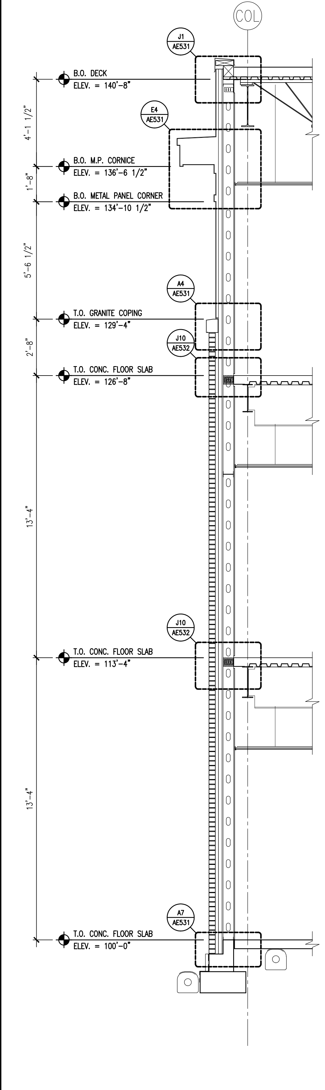
A10 WALL SECTION 3/8" = 1'-0"
