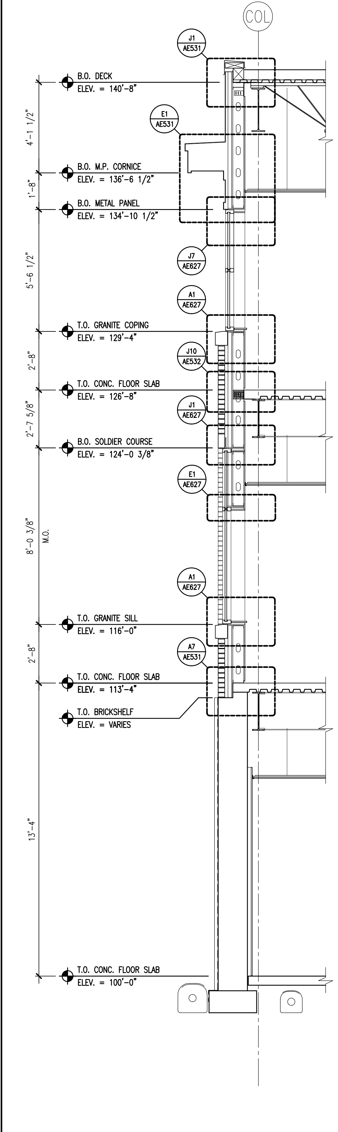
A4 WALL SECTION 3/8" = 1'-0"
