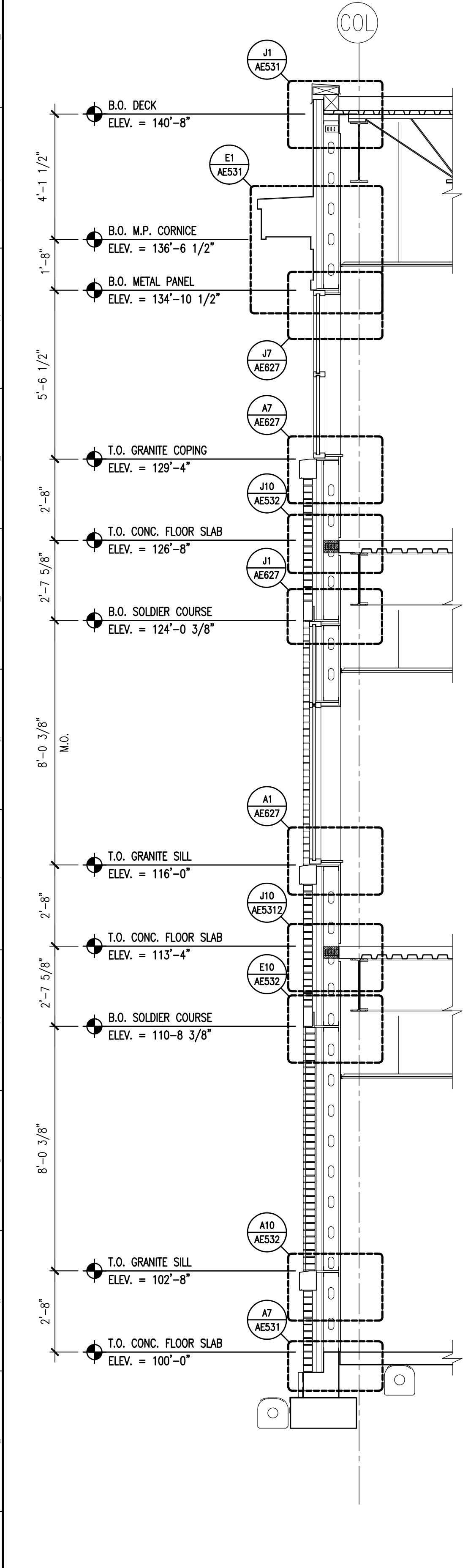
A1 WALL SECTION 3/8" = 1'-0"
