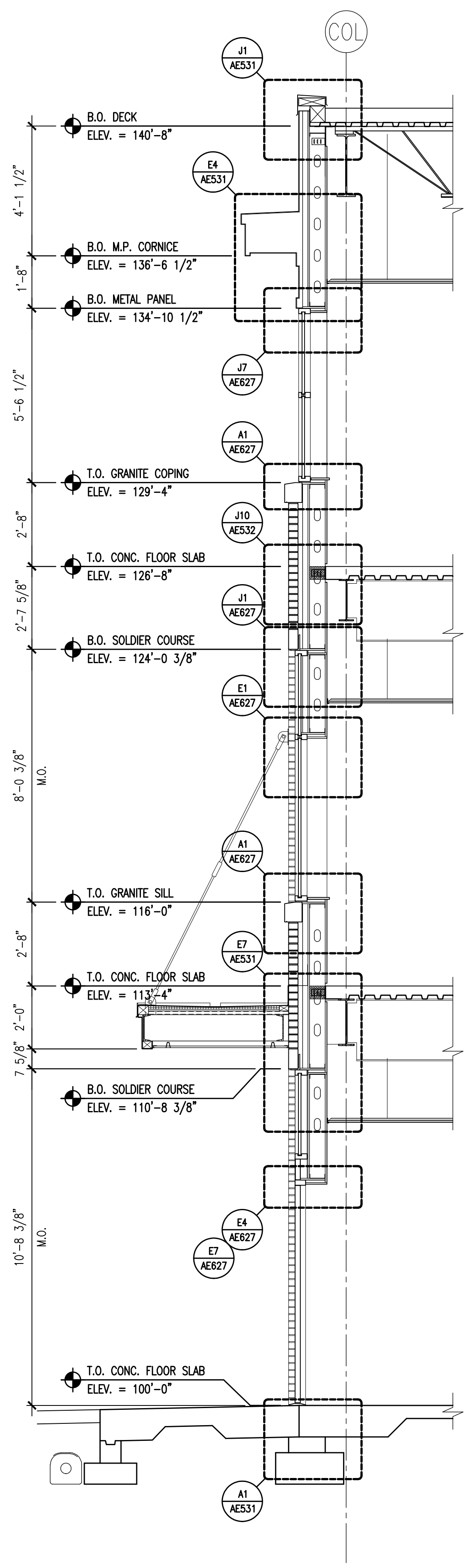
A1 WALL SECTION 3/8" = 1'-0"
