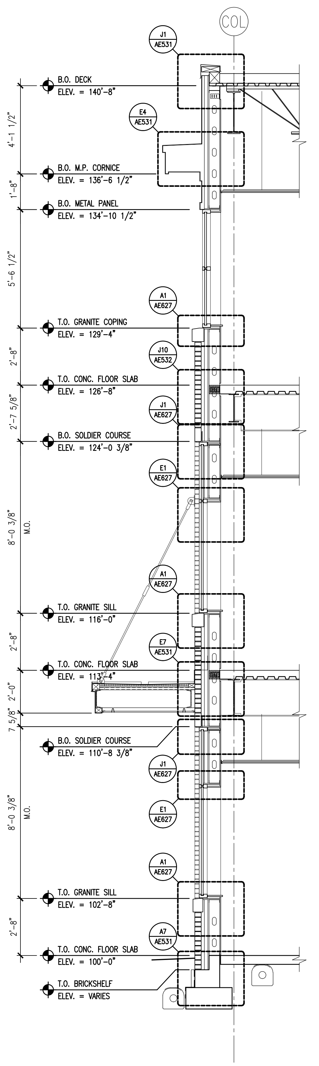
A7 WALL SECTION 3/8" = 1'-0"
