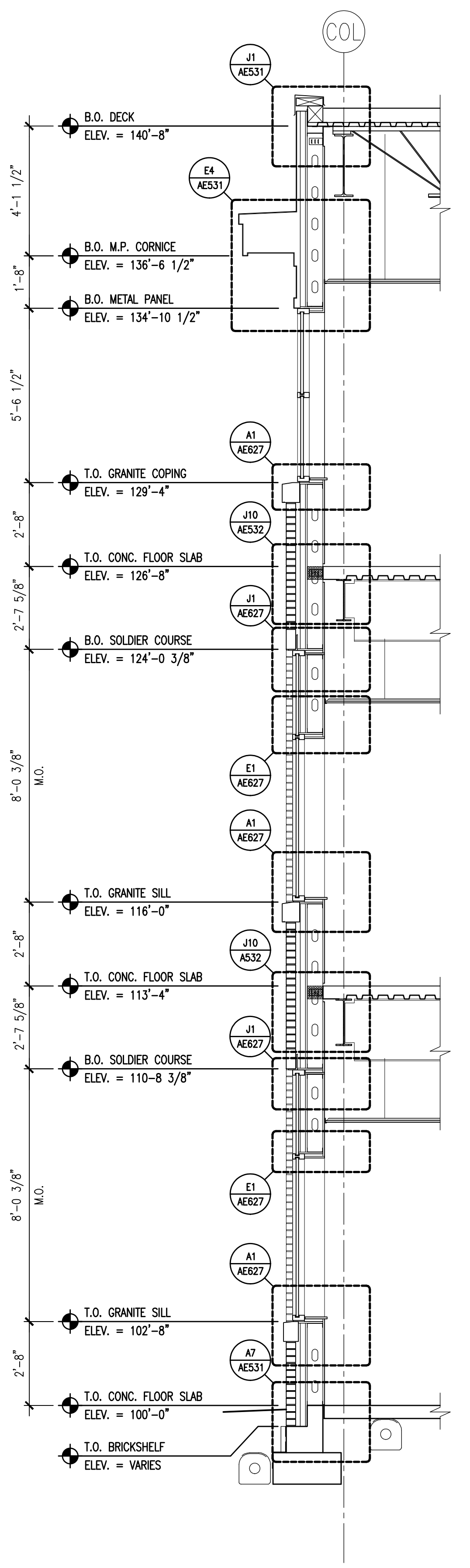
A10 WALL SECTION 3/8" = 1'-0"
