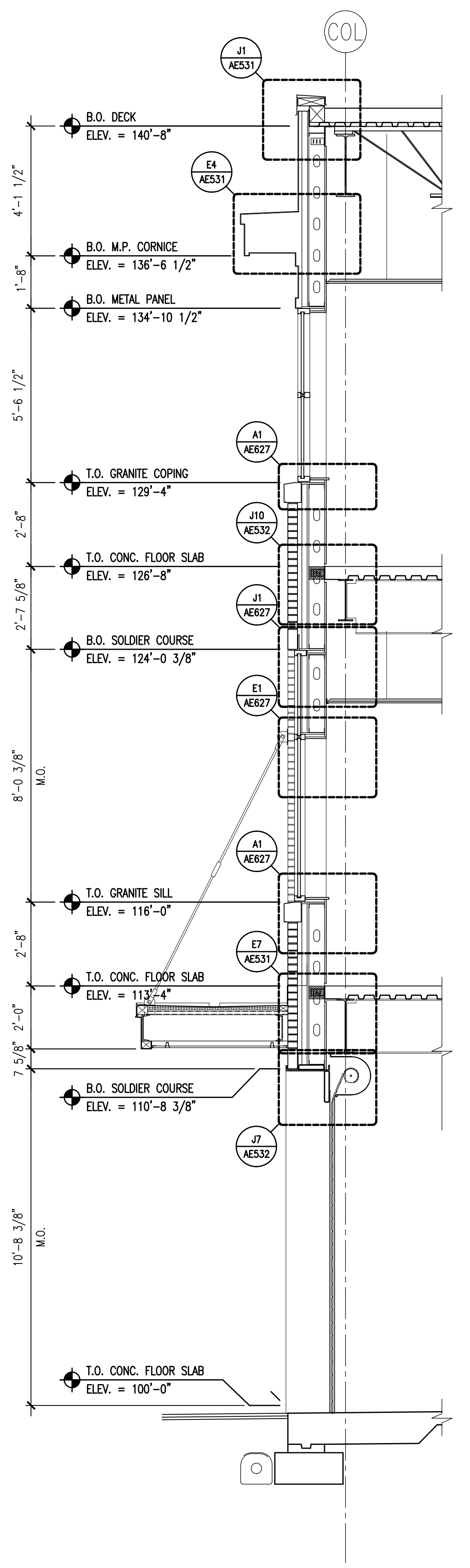
A4 WALL SECTION 3/8" = 1'-0"
