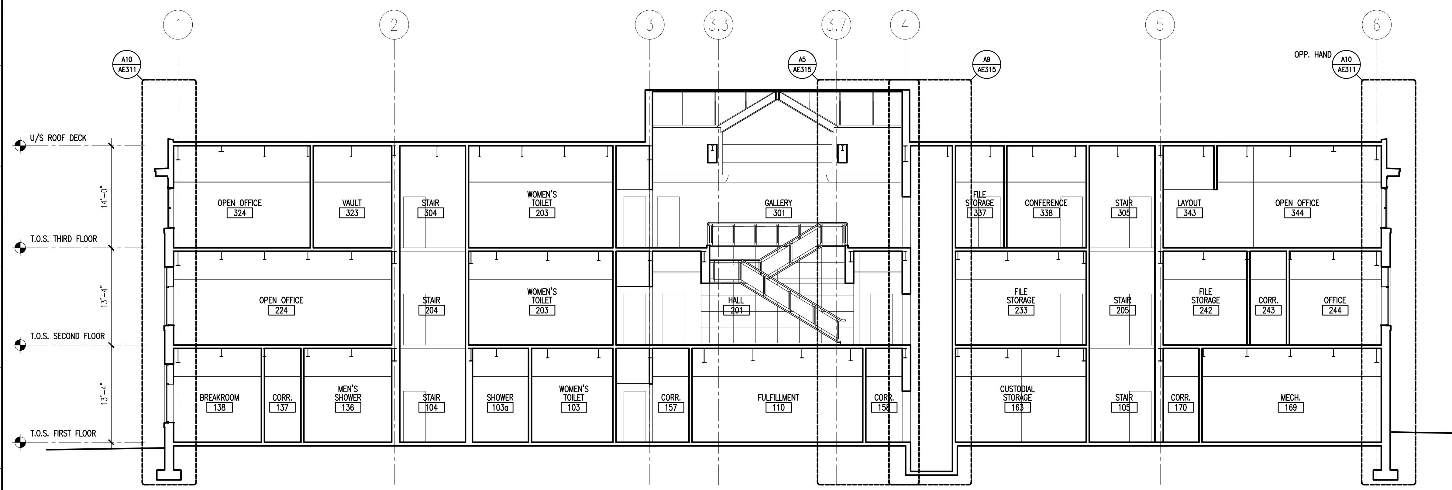
G1 BUILDING SECTION
