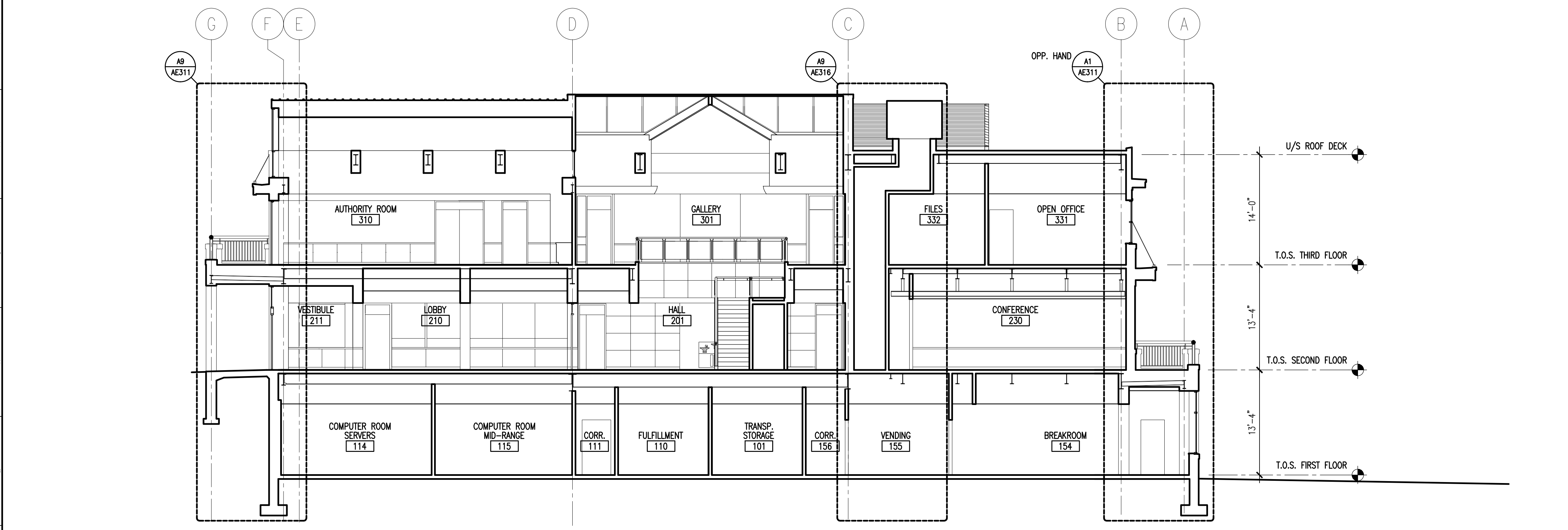
A1 BUILDING SECTION
